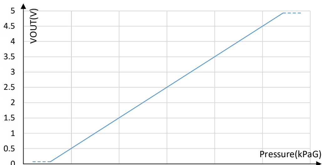
Figure 6.2 Analog Output Transfer Function
