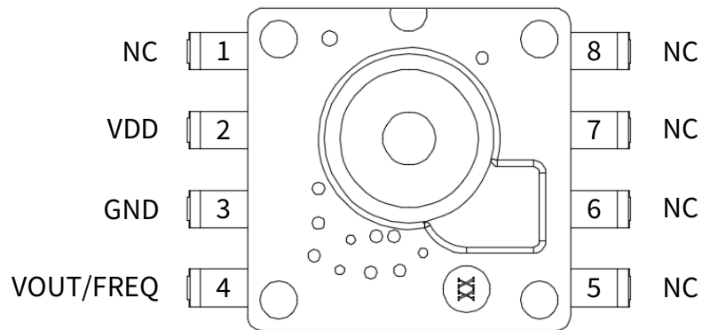
Figure 1.1 NSPGD1 Analog/ Frequency Output Pin Definition (top view)
