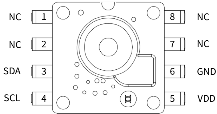
Figure 1.2 NSPGD1 Digital Output Pin Definition (top view)
