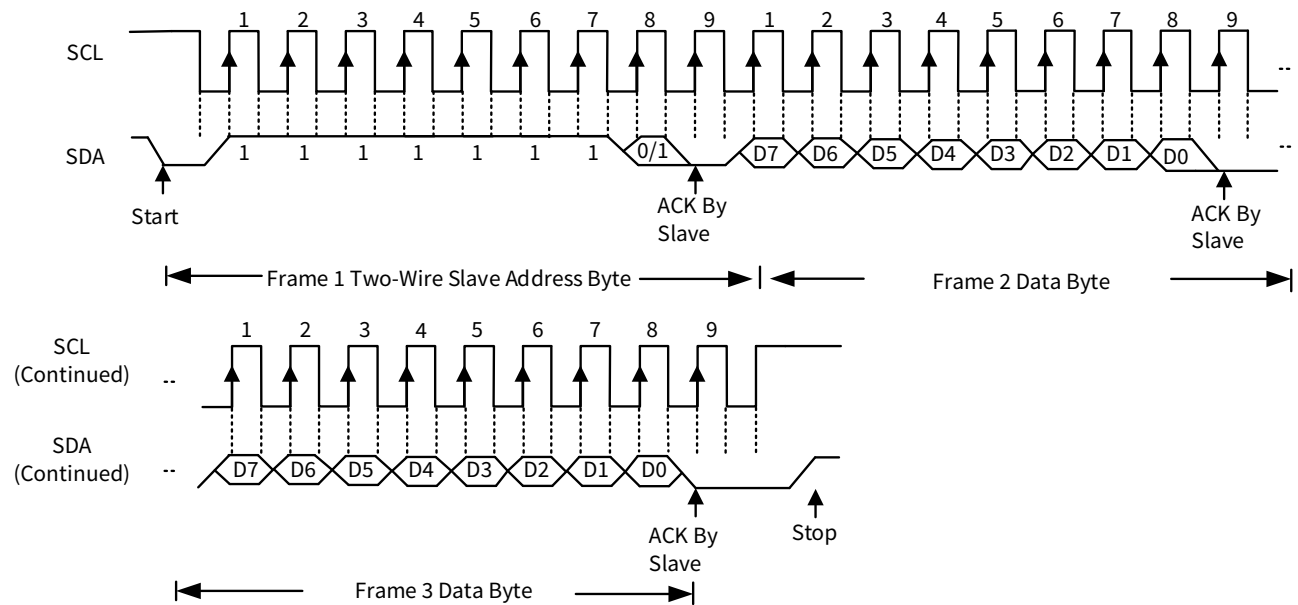
Figure 6.4 I²C Protocol
