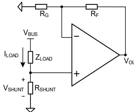
Figure 9-3 NSOPA810x-Q1 in a Low-Side, Current-Sensing Application
