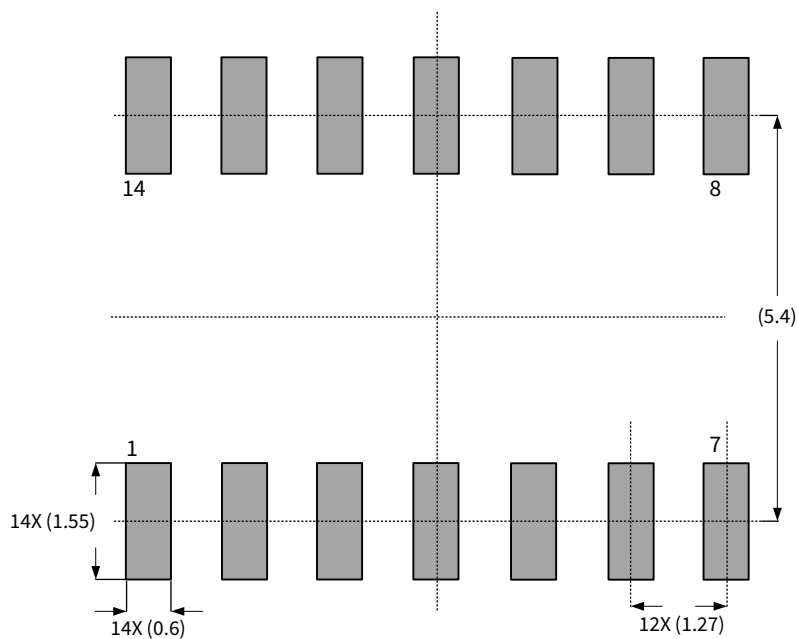
SOP14
