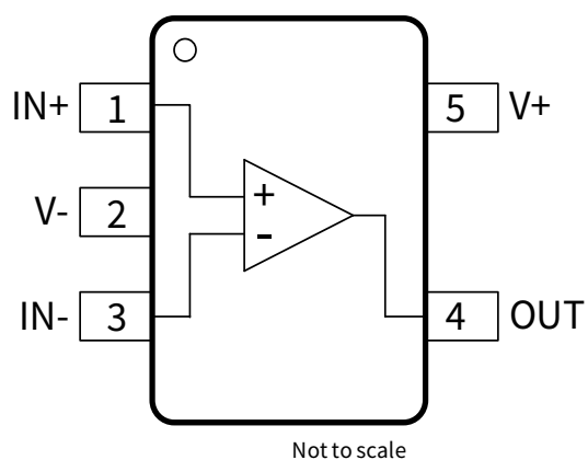
Figure 1-2 NSOPA8101-Q1 5-Pin SC70 Package Top View
