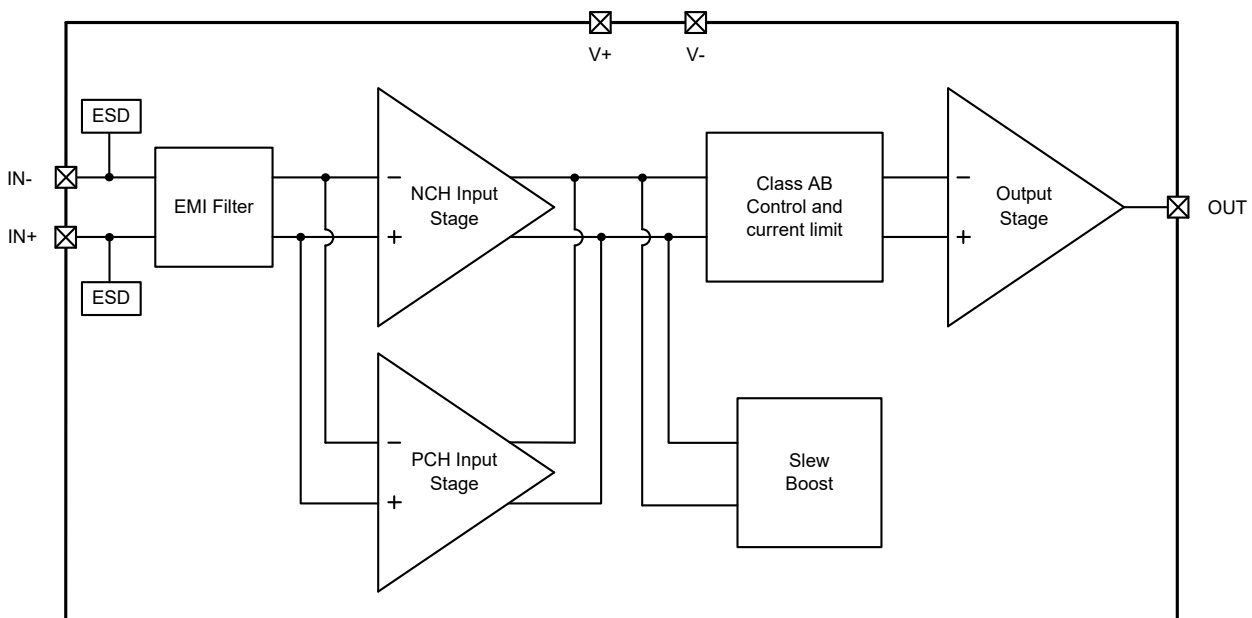
Figure 8-1 NSOPA810x-Q1 Functional block Diagram (One channel is shown)
