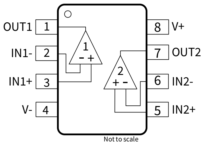
Figure 1-3 NSOPA8102-Q1 8-Pin SOP and MSOP Package Top View
