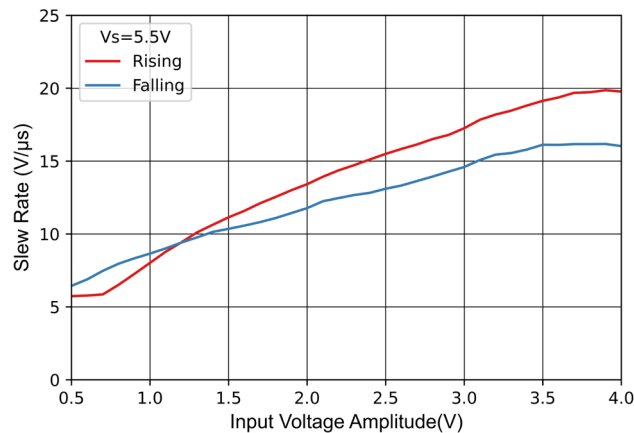
Figure 8-3 Slew-Rate vs Input Voltage Amplitude
