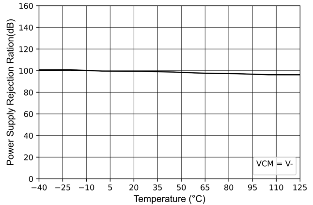
Figure 7-8 Power-Supply Rejection Ratio vs Temperature
