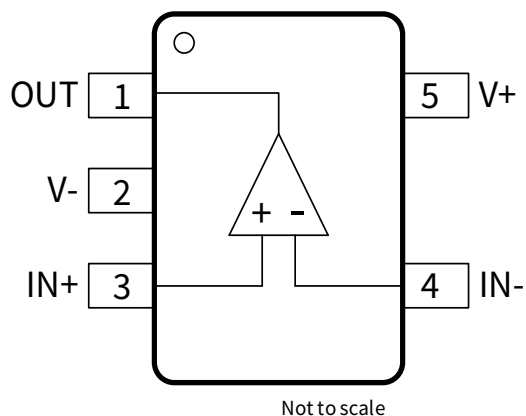
Figure 1-1 NSOPA8101-Q1 5-Pin SOT23 Package Top View
