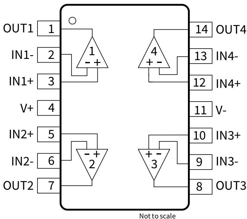
Figure 1-4 NSOPA8104-Q1 14-Pin SOP and TSSOP Package Top View
