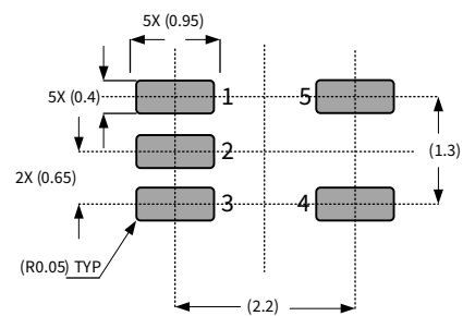
SC70-5
