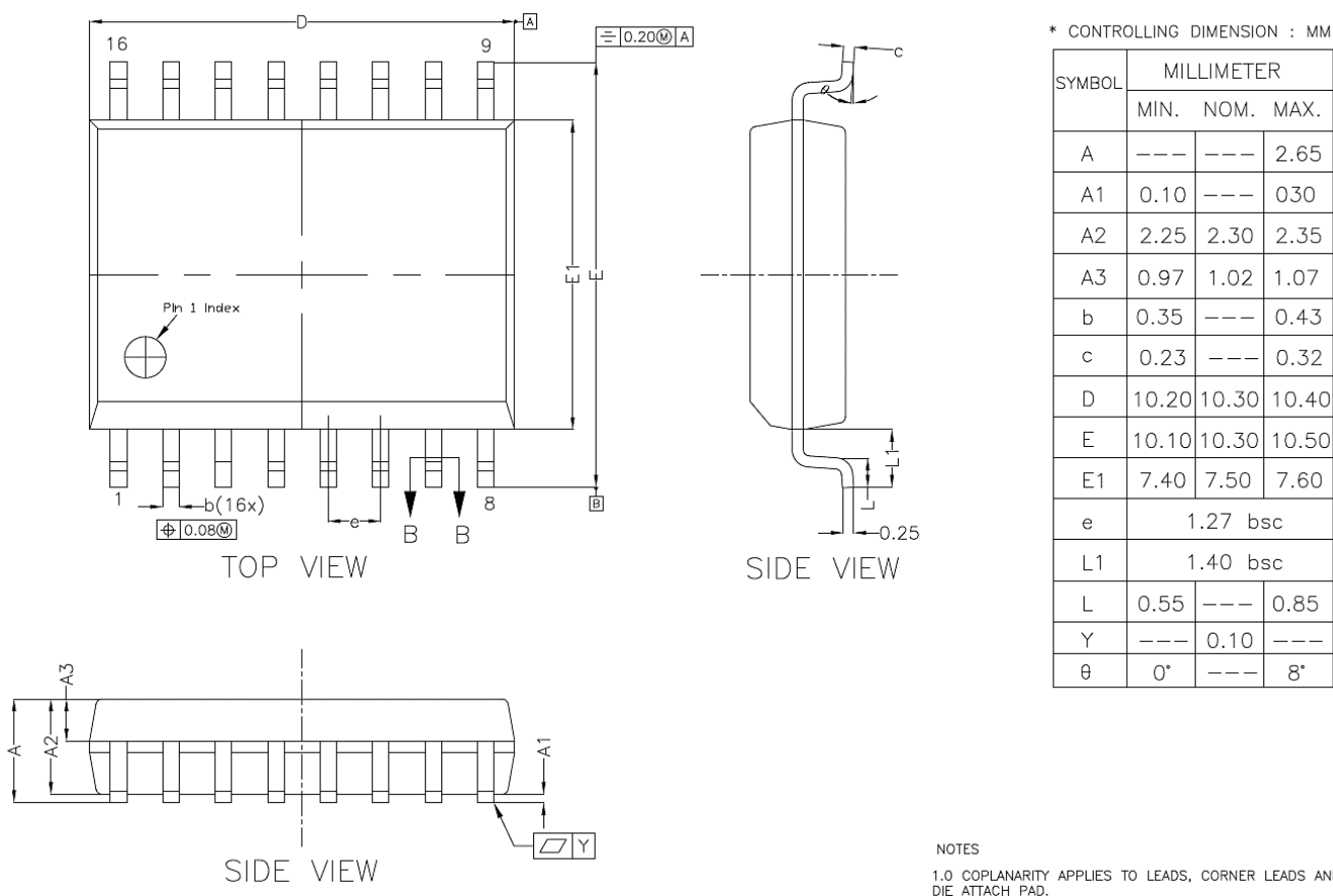
Figure 10.3 SOW16 Package Shape and Dimension
