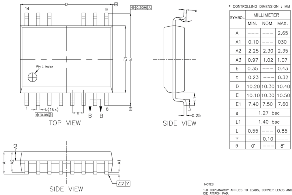
Figure 10.5 SOW14 Package Shape and Dimension
