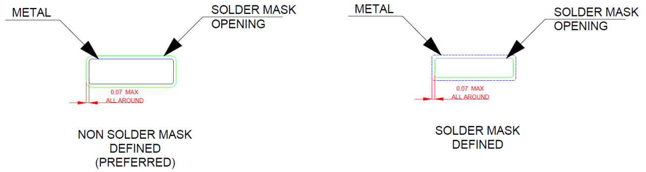
Figure 10.11 Solder Mask Details(mm)
