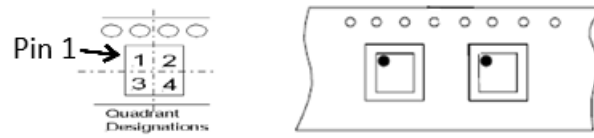
Figure 12.5 Quadrant Designation for Pin1 Orientation in Tape
