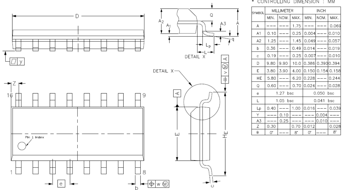
Figure 10.7 SOP16 Package Shape and Dimension
