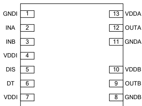
Figure 1.1 NSI6602V LGA13 Package
