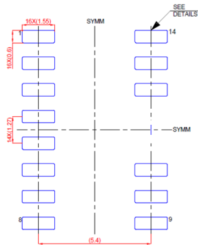
Figure 10.10 SOP14 Package Board Layout Example(mm)
