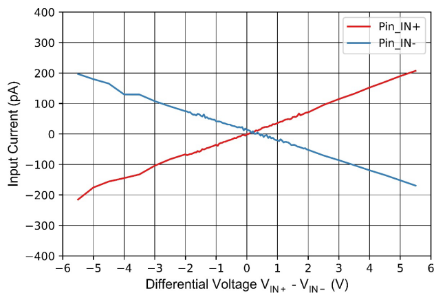
Figure 7-35 Input Current vs Differential Voltage
