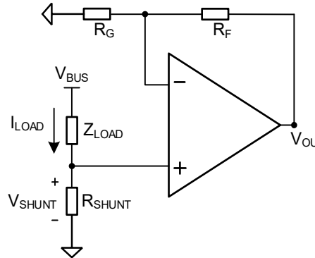
Figure 9-3 NSOPA810x in a Low-Side, Current-Sensing Application
