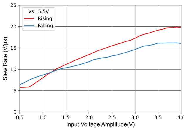
Figure 7-21 Slew Rate vs Input Voltage Amplitude
