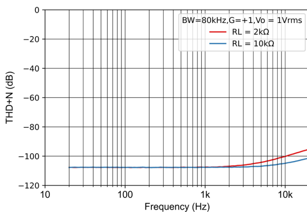
Figure 7-29 THD+N Ratio vs Frequency
