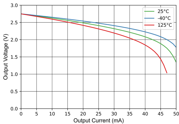
Figure 7-33 Output Voltage Swing vs Output Sourcing Current
