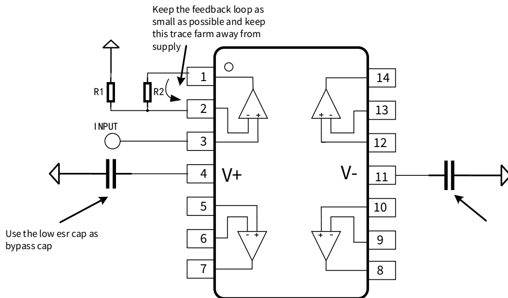
Figure 10-1 Layout example
