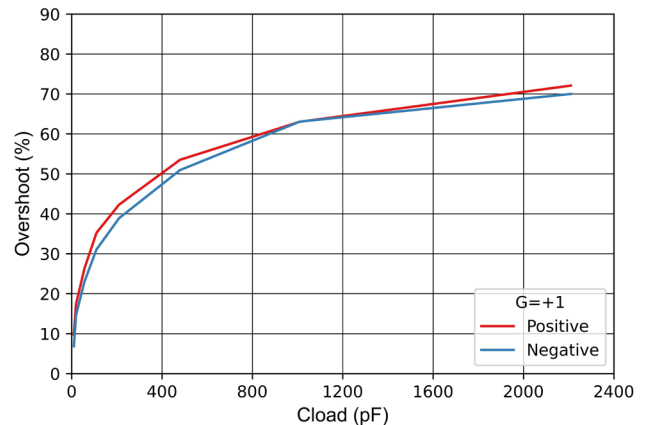
Figure 7-32 Small-Signal Overshoot vs Capacitive Load
