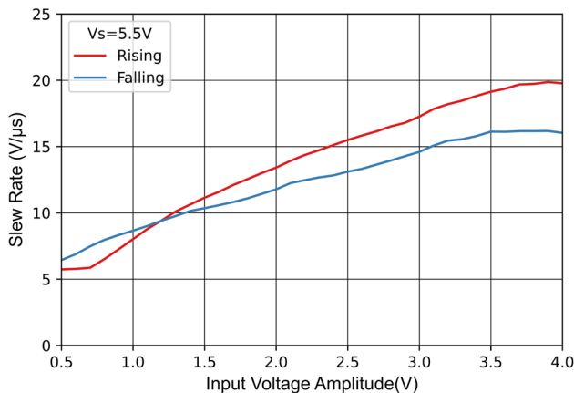
Figure 8-3 Slew-Rate vs Input Voltage Amplitude
