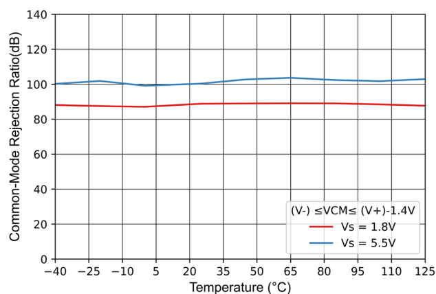
Figure 7-5 Common-Mode Rejection Ratio vs Temperature
