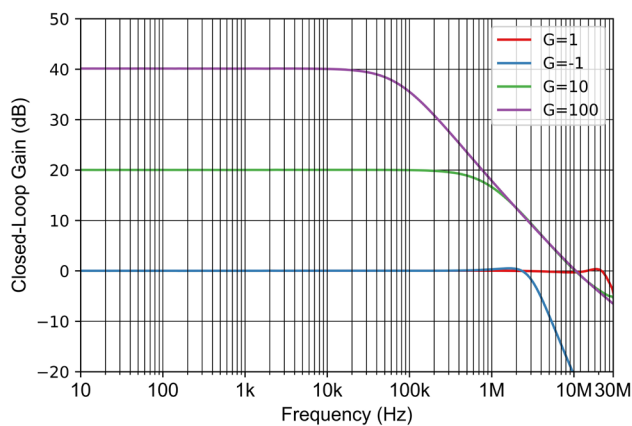
Figure 7-17 Closed Loop Gain vs Frequency
