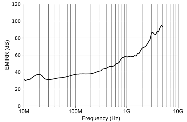
Figure 7-38 EMIRR vs Frequency
