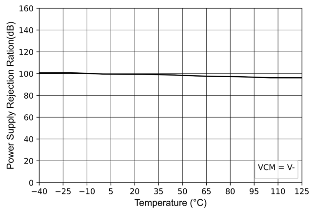
Figure 7-8 Power-Supply Rejection Ratio vs Temperature
