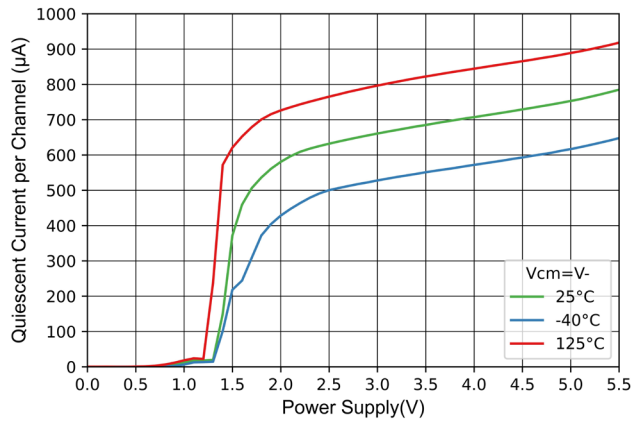
Figure 7-13 Quiescent Current vs Supply Voltage
