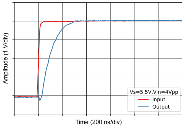
Figure 7-19 Large-Signal Step Response (Rising)
