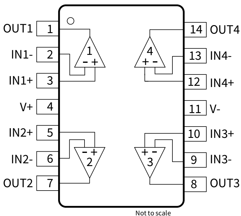
Figure 1-4 NSOPA8104 14-Pin SOP and TSSOP Package Top View
