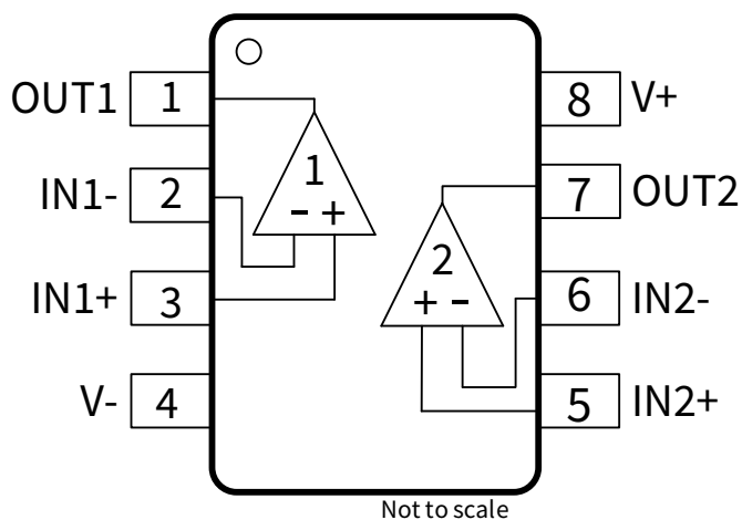
Figure 1-3 NSOPA8102 8-Pin SOP and MSOP Package Top View
