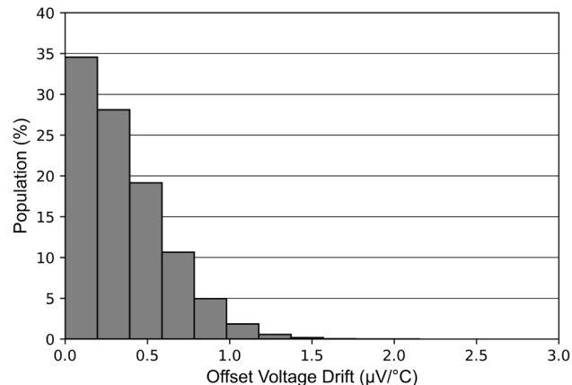
Figure 7-2 Offset Voltage Drift Distribution
