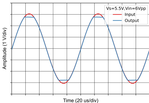
Figure 7-23 No Phase Reversal
