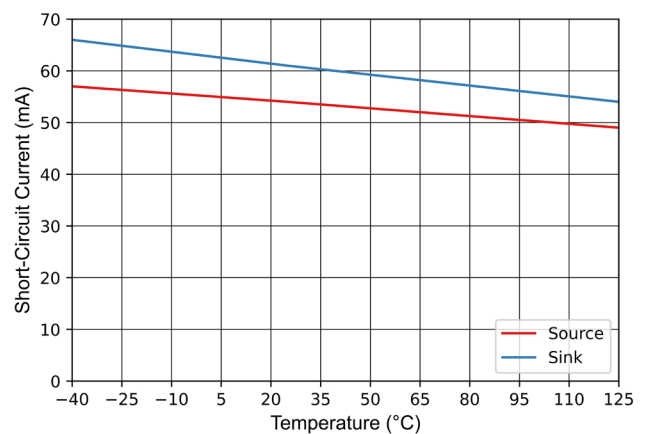
Figure 7-36 Short-Circuit vs Temperature
