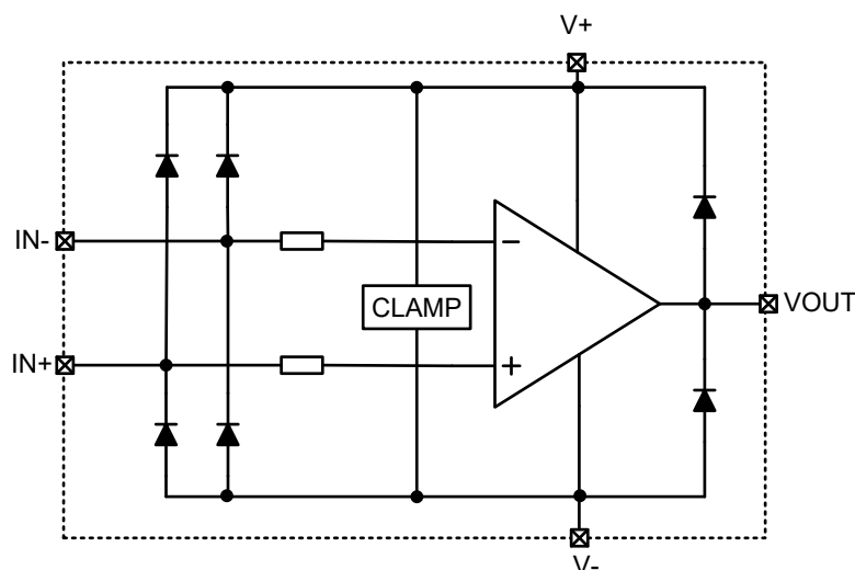
Figure 8-5 Internal ESD Equipment Model
