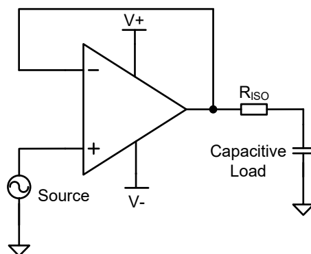
Figure 8-4 Insert isolation Resistor to drive large Capacitive Load
