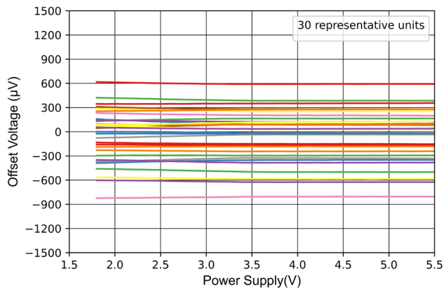
Figure 7-7 Offset Voltage vs Power Supply
