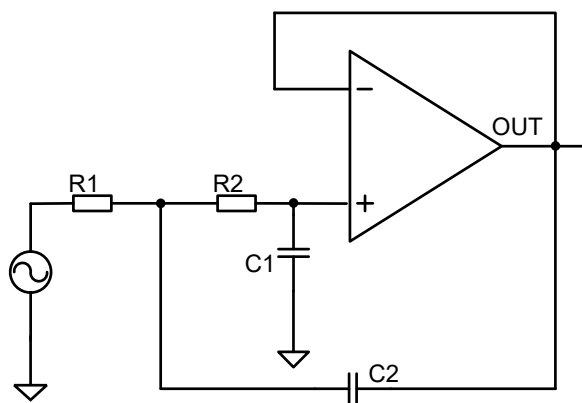
Figure 9-1 Second-Order Sallen-Key Filter
