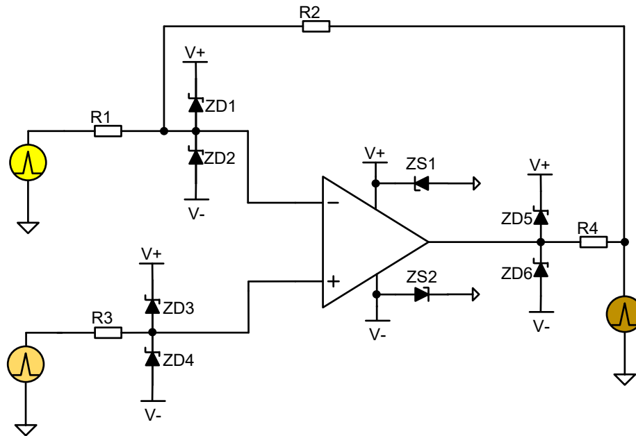
Figure 8-6 External component to enhance EOS performance
