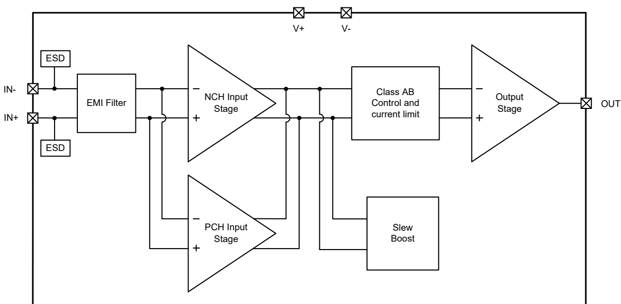
Figure 8-1 NSOPA810x Functional block Diagram (One channel is shown)
