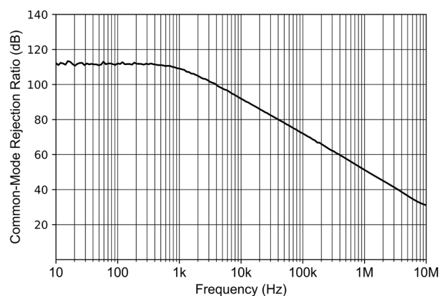
Figure 7-6 Common-Mode Rejection Ratio vs Frequency
