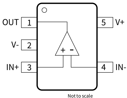
Figure 1-1 NSOPA8101 5-Pin SOT23 Package Top View
