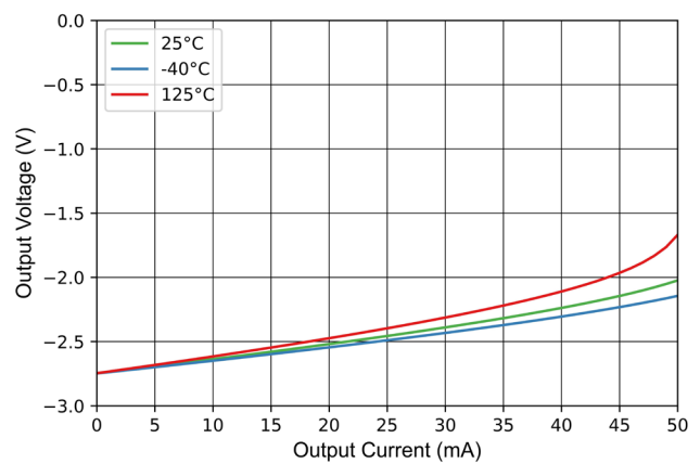
Figure 7-34 Output Voltage Swing vs Output Sinking Current
