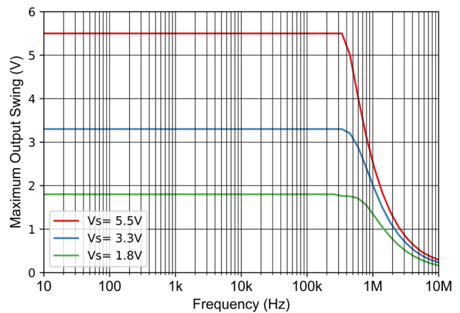
Figure 7-18 Maximum Output Voltage vs Frequency
