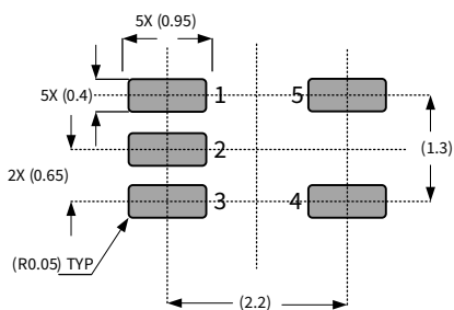
SC70-5
