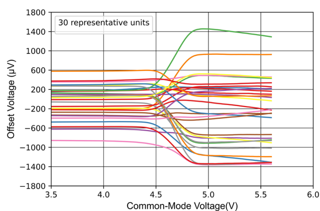
Figure 7-4 Offset Voltage vs Common-Mode Voltage(Transition)
