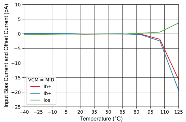
Figure 7-16 Input Bias Current vs Temperature
