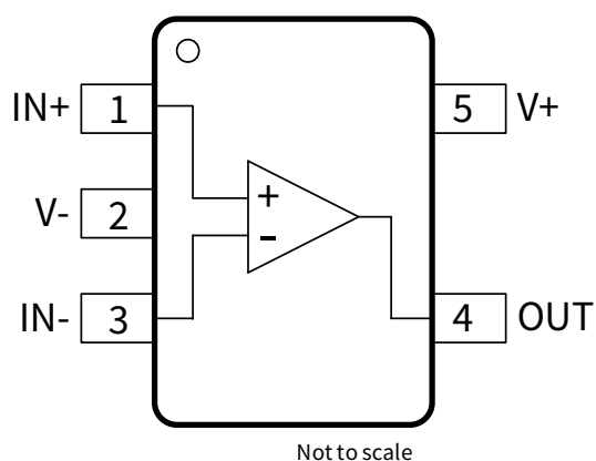
Figure 1-2 NSOPA8101 5-Pin SC70 Package Top View
