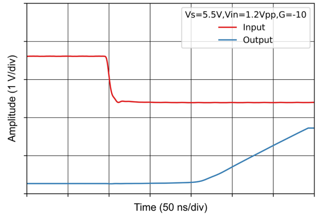
Figure 7-26 Negative Overload Recovery ( G = -10 )
