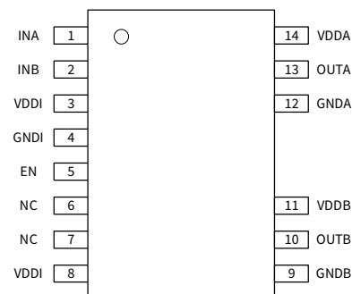
Figure 1.9 NSI6622N SOW14/ SOP14 Package
