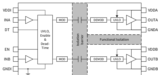
Figure 0.4 NSI6602N Block Diagram
