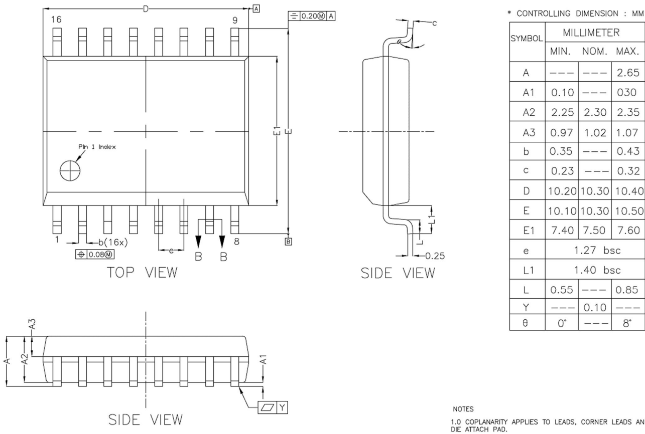
Figure 10.2 SOW16 Package Shape and Dimension
