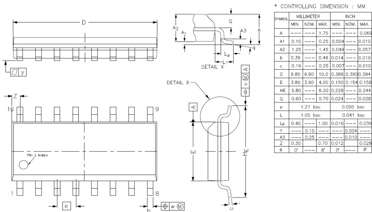
Figure 10.8 SOP16 Package Shape and Dimension
