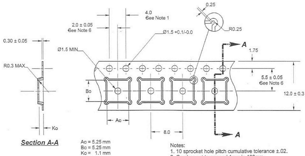
Figure 12.1 Tape Information
