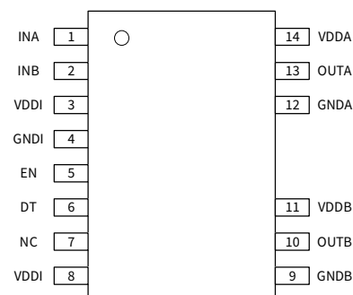
Figure 1.3 NSI6602N SOW14/ SOP14 Package
