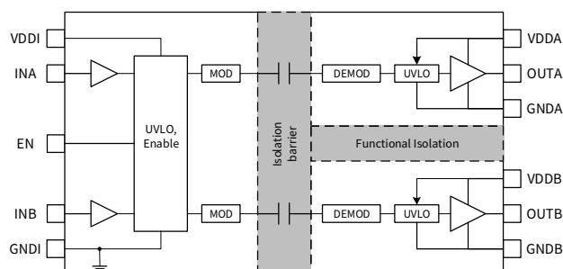
Figure 0.2 NSI6622N Block Diagram
