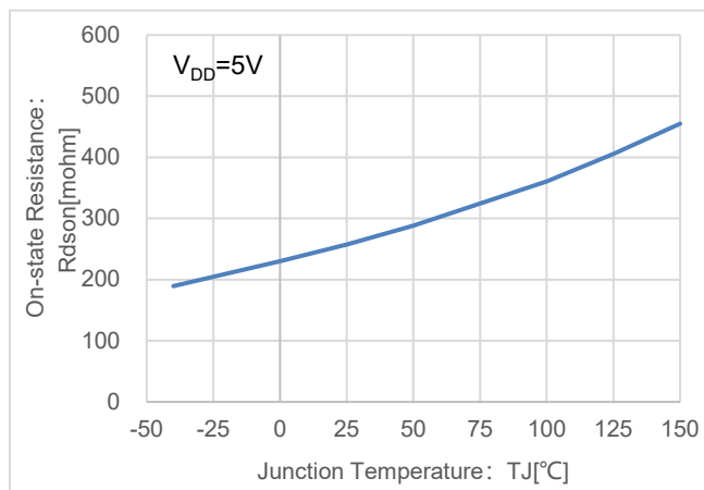
Figure 7.2 On-state Resistance vs Junction Temperature
