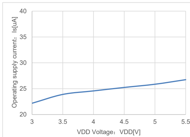
Figure 7.4 VDD Operating supply Current vs VDD Voltage
