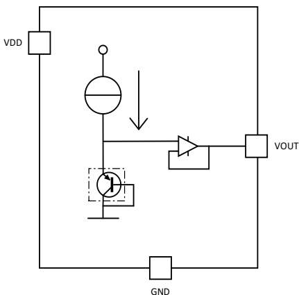
Figure 3.1 NST60 Functional Block Diagram
