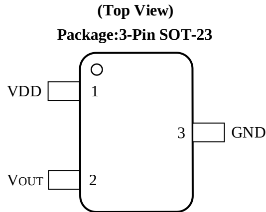
Figure 1.1 NST60 Pin Configuration
