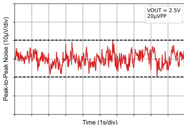
Figure 8.4 0.1Hz to 10Hz Voltage Noise
