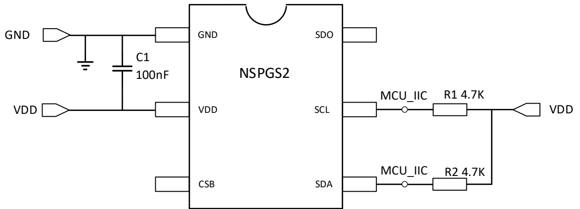
Figure 7.3 I 2 C Output Application Circuit
