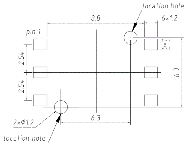
Figure 8.2 Footprint mm
