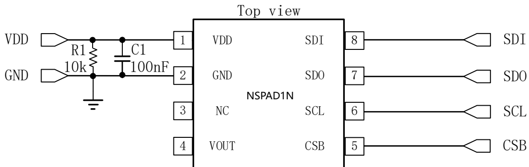
Figure 7.3 SPI Output Application Circuit
