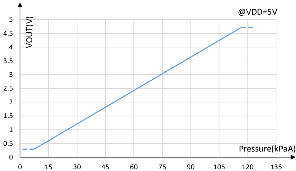
Figure 6.7 NSPAD1N115RR01 Transfer Function
