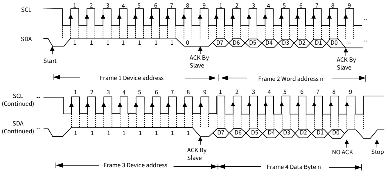
Figure 6.11 I 2 C Read Byte
