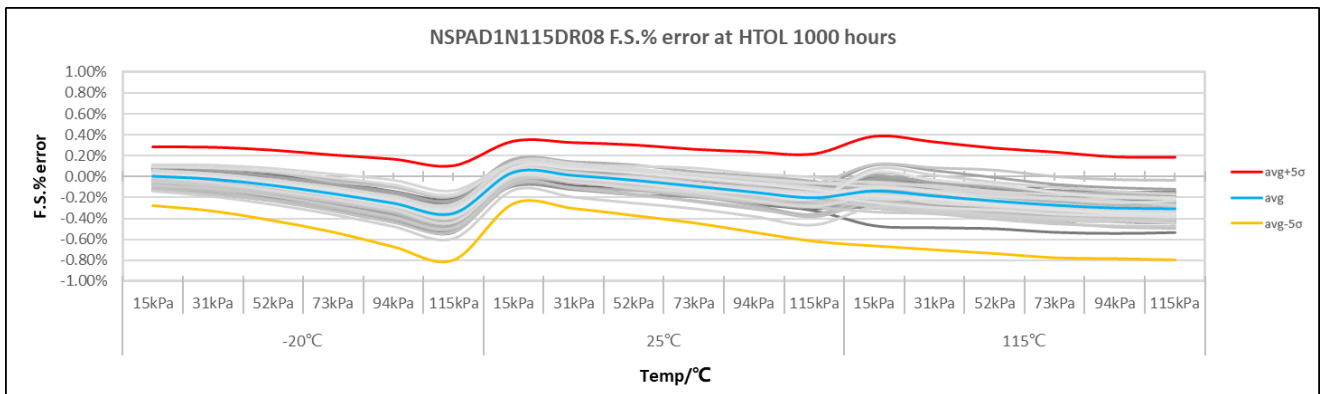
Figure 6.6 NSPAD1N115DR08 Full Scale Error at HTOL 1000-hours
