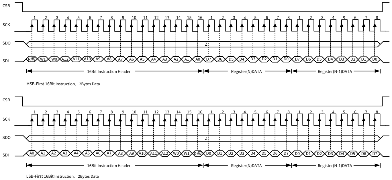
Figure 6.13 MSB First and LSB First Instruction and Data Phases
