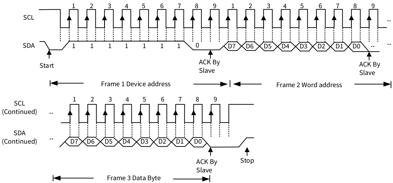
Figure 6.10 I 2 C Write Byte
