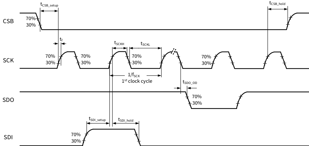
Figure 5.2 SPI Timing Diagram
