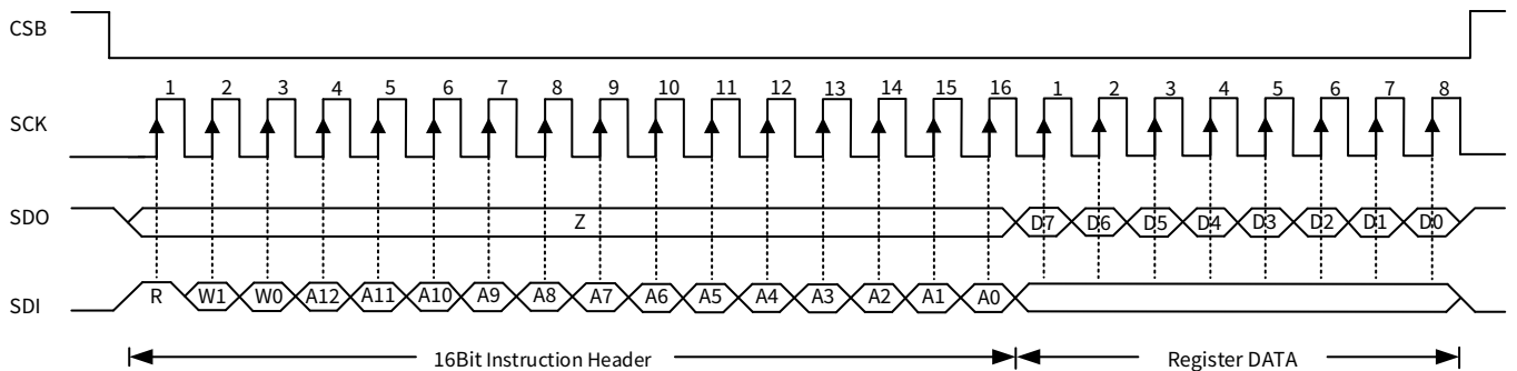
Figure 6.15 SPI Read Byte
