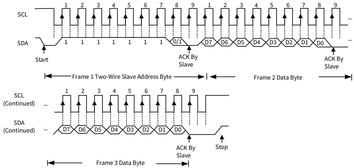
Figure 6.9 I 2 C Protocol
