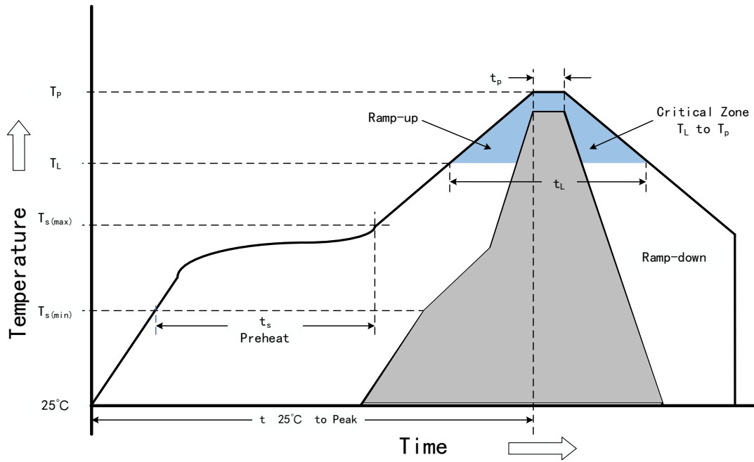
Figure 7.5 Soldering Profile
