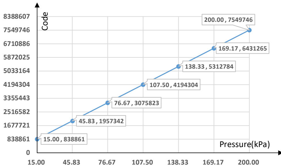
Figure 6.8 NSPAD1N200DR04 Transfer Function
