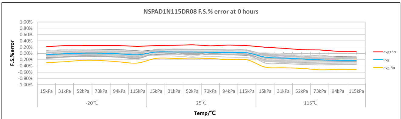
Figure 6.5 NSPAD1N115DR08 Full Scale Error at 0-hours
