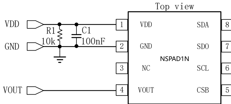
Figure 7.1 Analog Output Application Circuit
