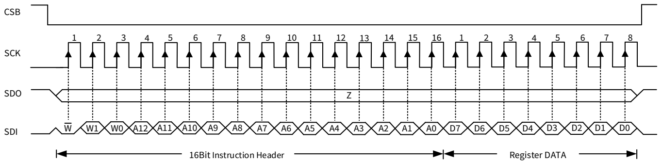
Figure 6.14 SPI Write Byte
