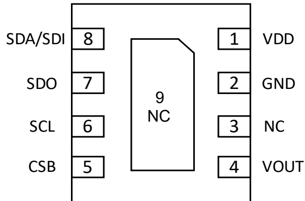
Figure 1.1 NSPAD1N Pin Definition (Bottom View)
