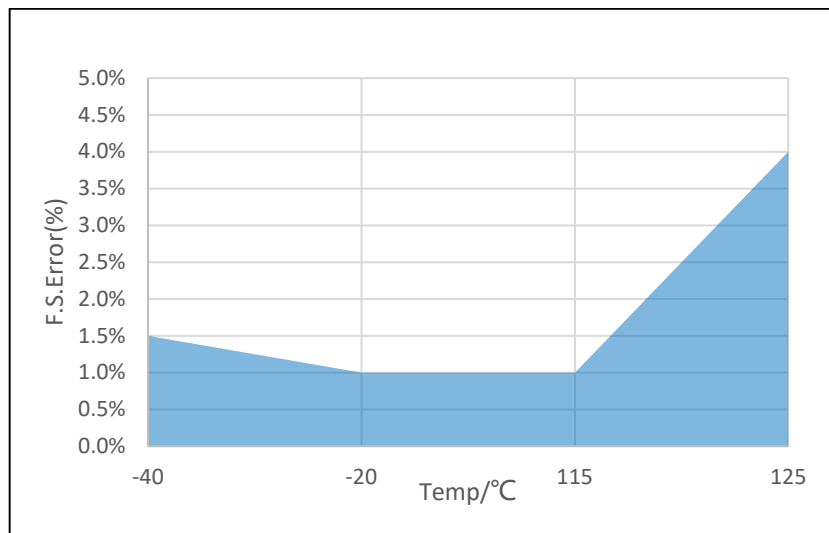
Figure 6.3 Digital Output Accuracy
