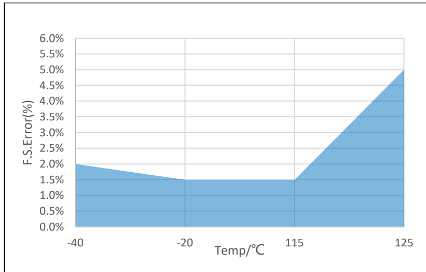
Figure 6.4 Analog Output Accuracy
