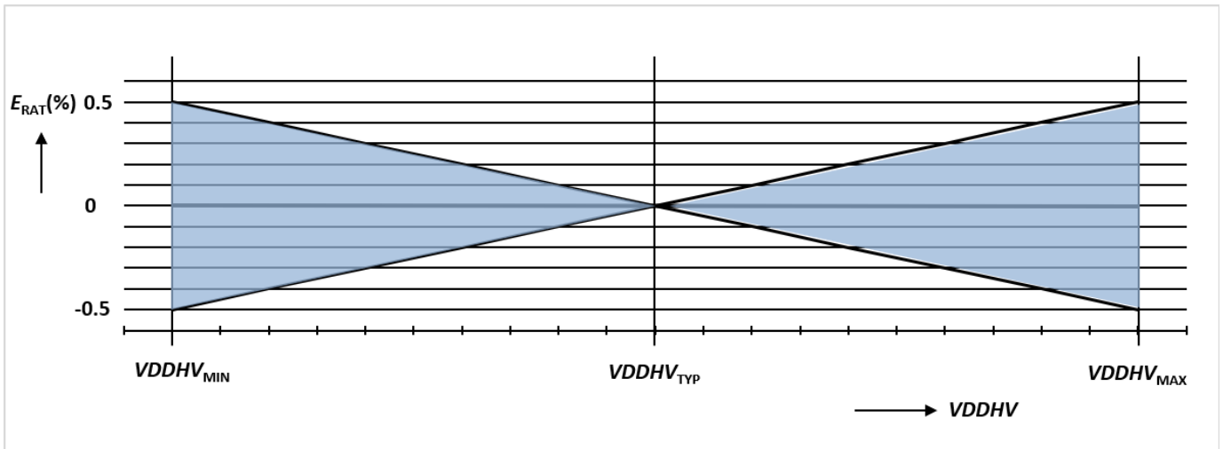
Figure 6.2 Ratiometric Error
