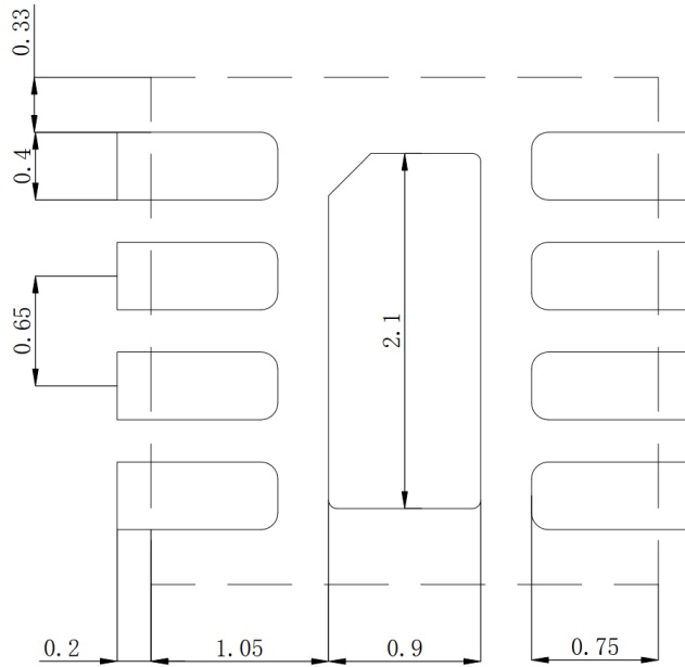
Figure 7.4 Footprint (unit: mm)
