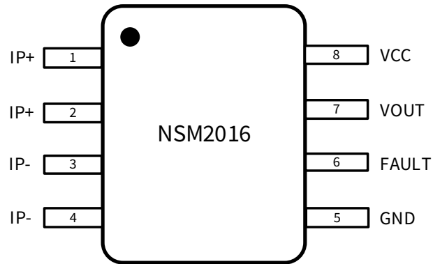
Figure 1.1 NSM2016 Package
