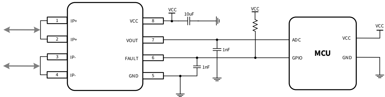
Figure 7.1 Typical application diagram of fixed output mode
