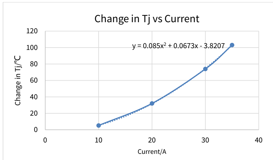
Figure 7.4 NSM2016 Estimation function of junction temperature at different currents (PCB is in worst case)
