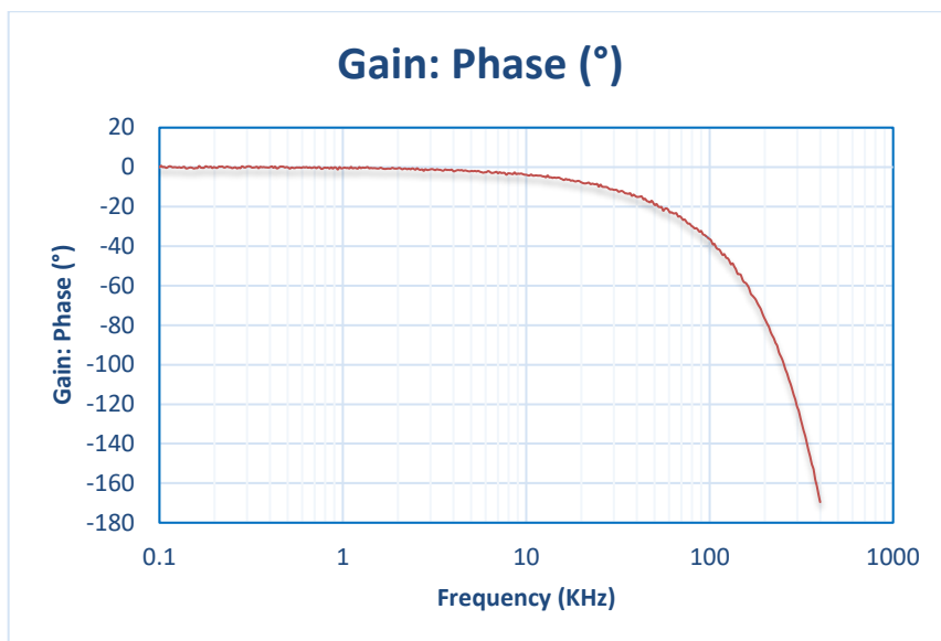
Figure 6.4 NSM2016 Phase frequency response curve
