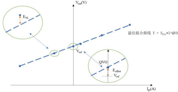
Figure 6.7 NSM2016 Sensitivity and Error
