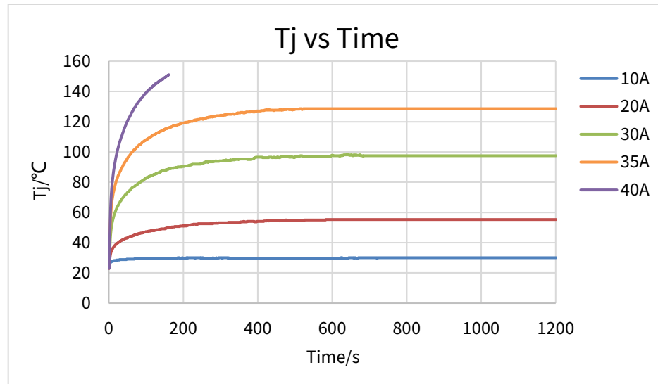
Figure 7.3 NSM2016 Junction temperature vs. Different continues current
