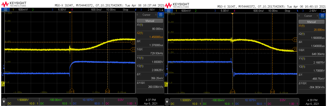
Rise time, yellow is Vout, blue line is step primary current
