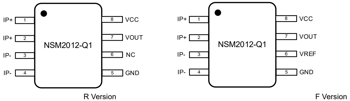
Figure 1.1 NSM2012-Q1 Package
