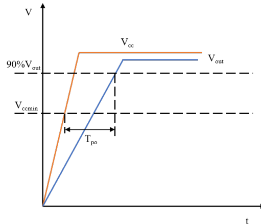
Figure 6.1 NSM2012-Q1 Power-on Time
