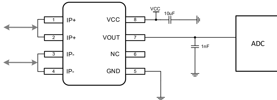
Figure 7.1 Typical application diagram of ratiometric output mode
