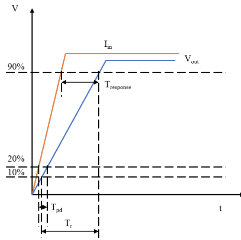
Figure 6.2 NSM2012-Q1 Response Time
