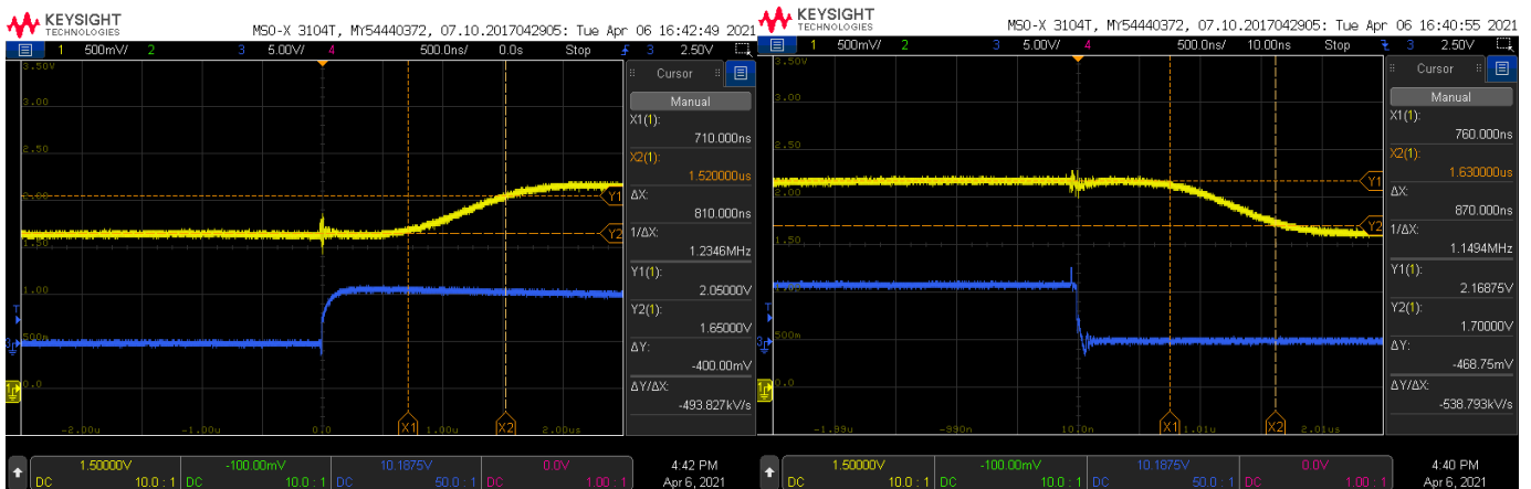
Yellow is Vout, blue is 1kHz , 1A primary current
