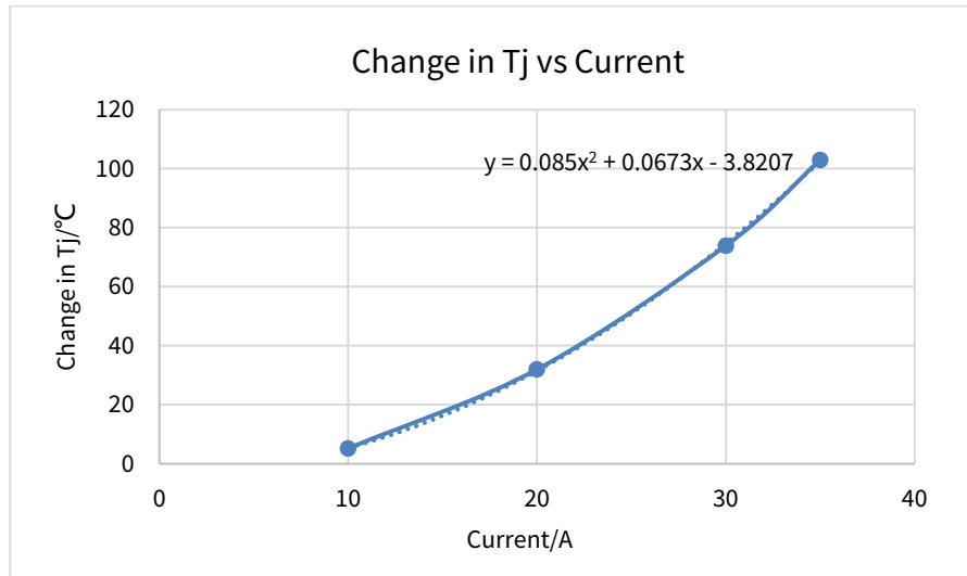
Figure 7.5 NSM2012-Q1 Estimation function of junction temperature at different currents (PCB is in worst case)
