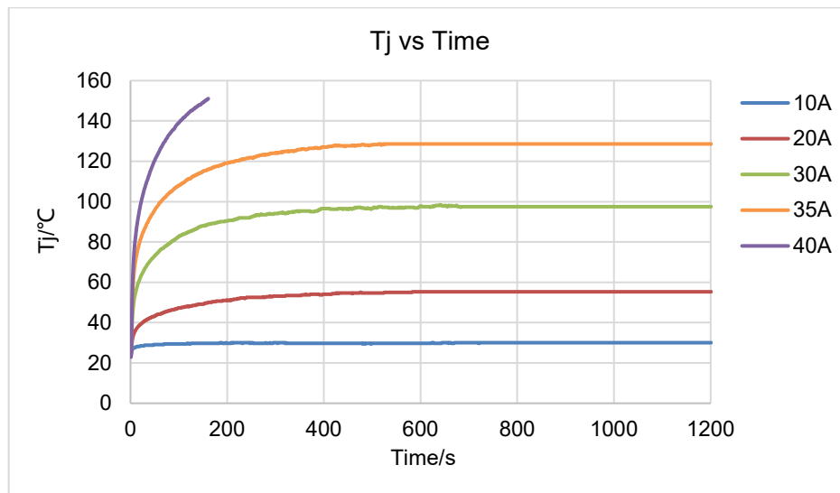
Figure 7.4 NSM2012-Q1 Junction temperature vs. Different continues current
