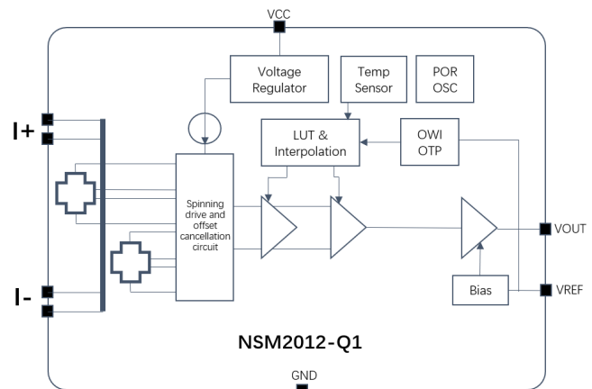
Figure 1. NSM2012-Q1 Block Diagram
