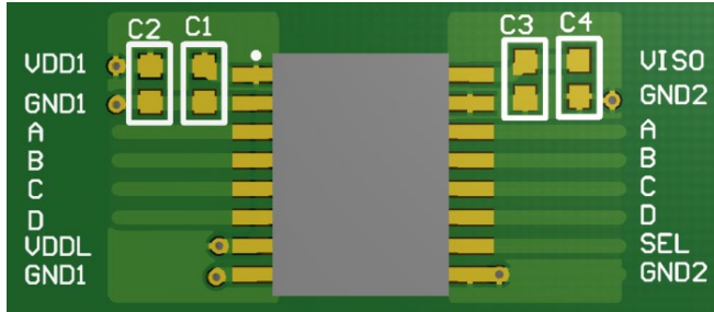
Figure 8.3 Recommended PCB Layout — Top Layer
