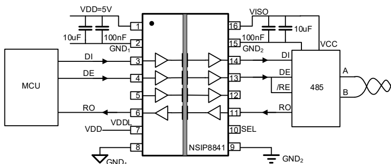
Figure 8.2 Isolated RS485 schematic using NSIP884x
