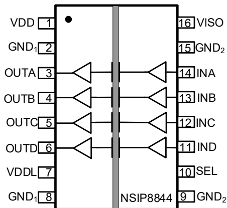
Figure 1.5 NSIP8844 Package
