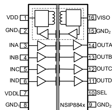
Figure 1. NSIP884x Block Diagram 1
