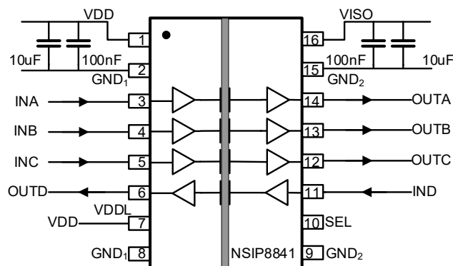
Figure 8.1 Basic schematic of NSIP884x
