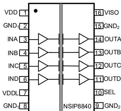
Figure 1.1 NSIP8840 Package
