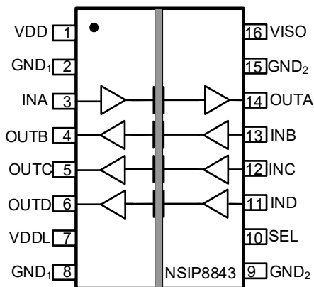
Figure 1.4 NSIP8843 Package
