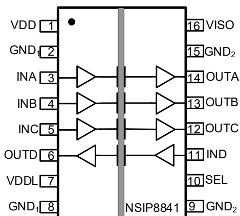
Figure 1.2 NSIP8841 Package
