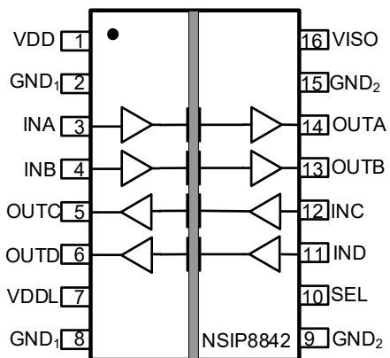
Figure 1.3 NSIP8842 Package
