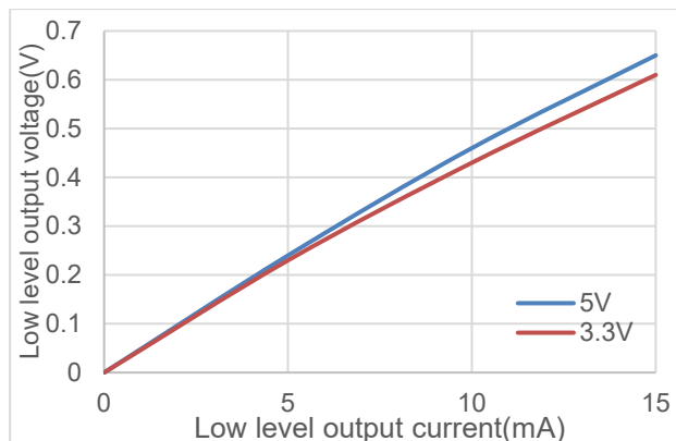
Figure 5.6 Low-Level Output Voltage vs Output Current
