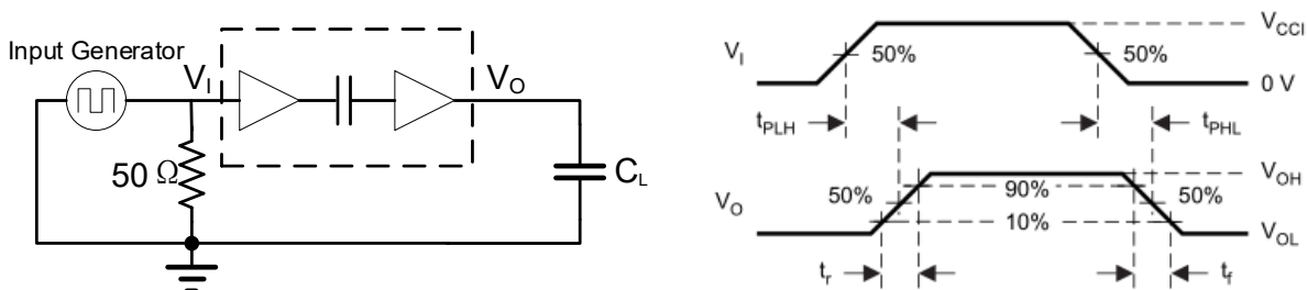
Figure 5.7 Switching Characteristics Test Circuit and Waveform
