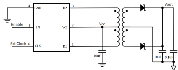
Figure 2. Simplified Schematic
