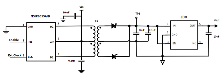
Figure 11.4 Stable output voltage and wide load current
