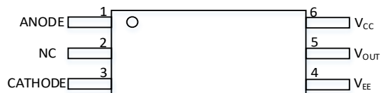
NSI6801E SOW6 and NSI6801E SOL6 Top View
