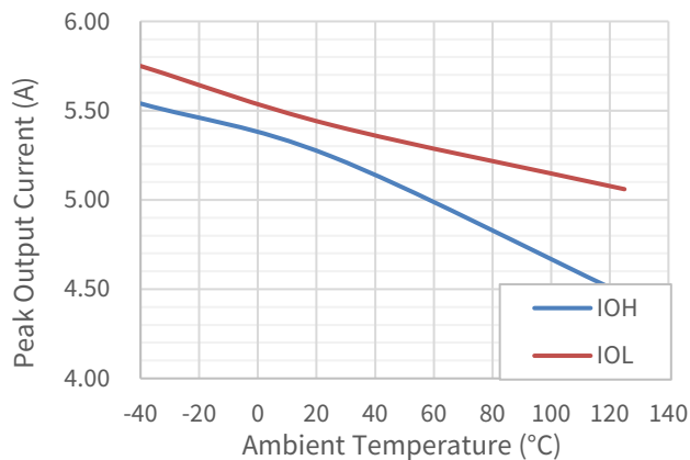
Figure 6.8 Output drive currents versus Temperature
