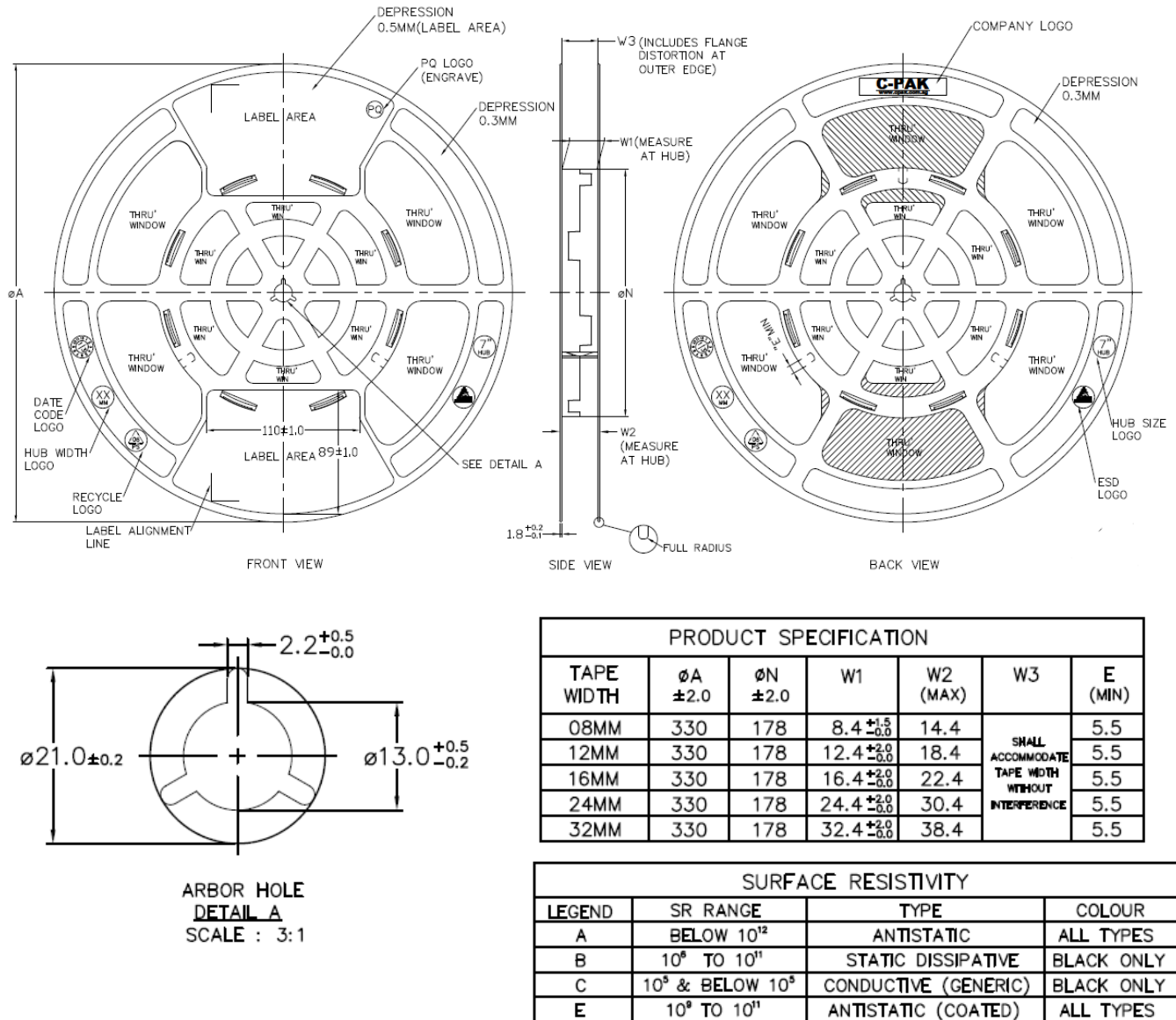
Figure 13.1 Reel Information
