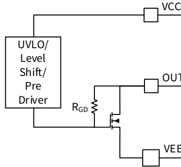
Figure 8.3 Active pulldown
