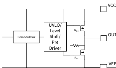
Figure 8.2 NSI6801E Output Stage
