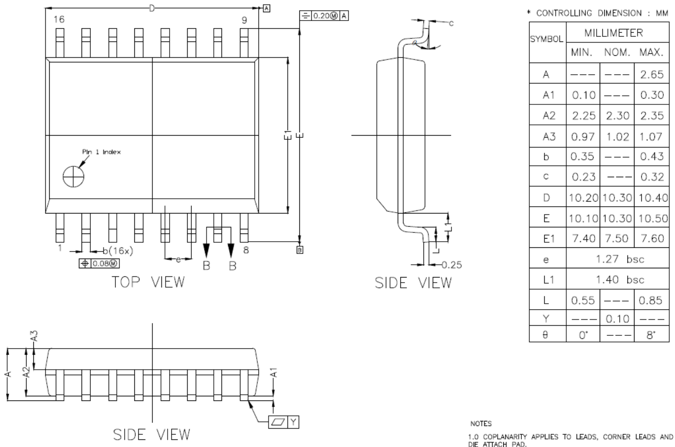
Figure 10.1 SOW16 package shape and dimension in millimeters
