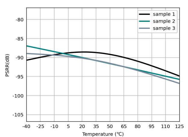
Figure 6.17 Power-Supply Rejection Ratio vs Temperature
