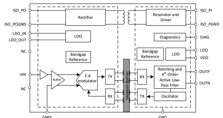
Figure 1. Function Block Diagram of NSI3611D
