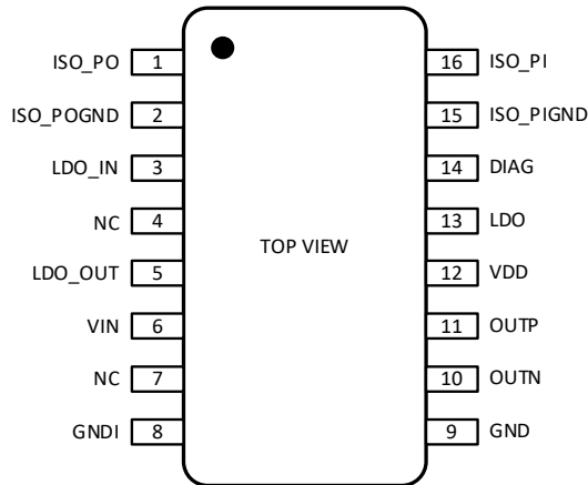
Figure 1.1 NSI3611D Package
