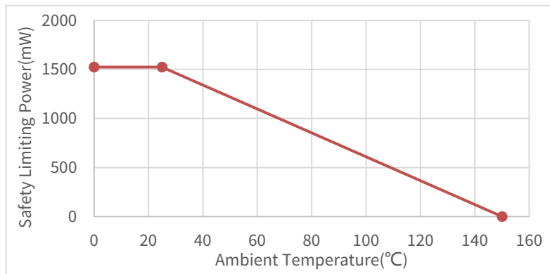
Figure 7.1 NSI3611D Thermal Derating Curve, Dependence of Safety Limiting Values with Case Temperature per DIN VDE V 0884-11
