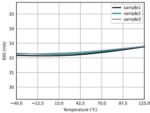
Figure 6.24 Input Supply Current vs Temperature ( I_E=1mA )
