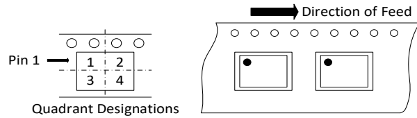
Figure 13.2 Reel Information of SOP16(300mil)
