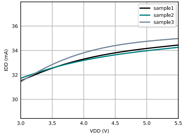
Figure 6.23 Input Supply Current vs Supply Voltage ( I_E=1mA )
