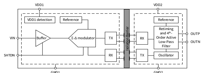
Figure 1. Block Diagram
