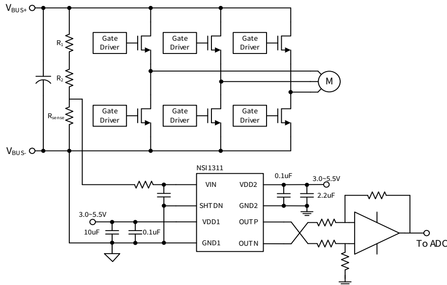
Figure 8.1 Typical application circuit in voltage sensing
