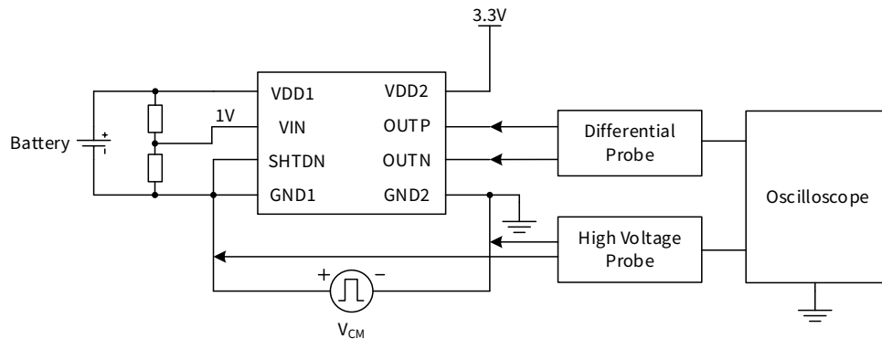
Figure 5.1212 Common-Mode Transient Immunity Test Circuit
