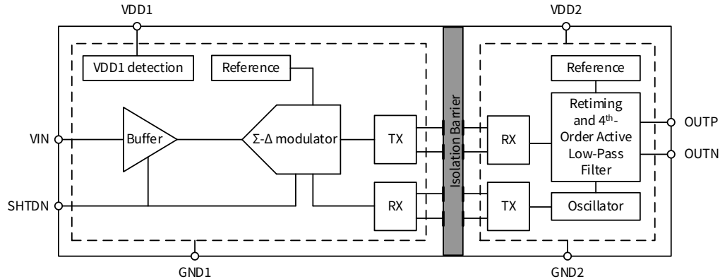
Figure 7.1 Function Block Diagram
