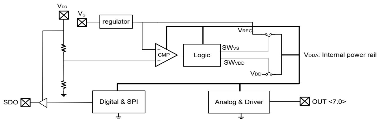
Figure 5.1 NSD56080 Internal Power Supply concept
