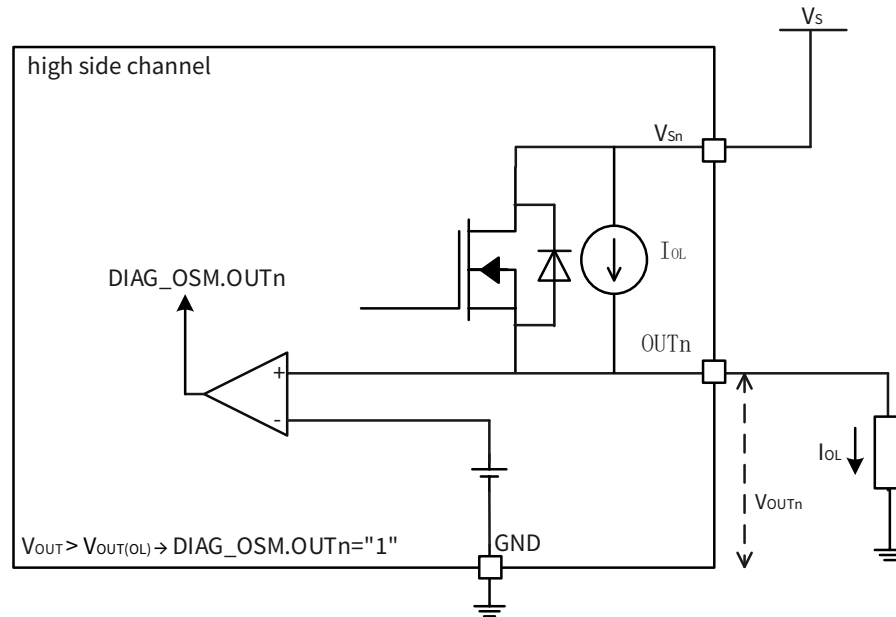
Figure 9.2 Output Status Monitor - concept
