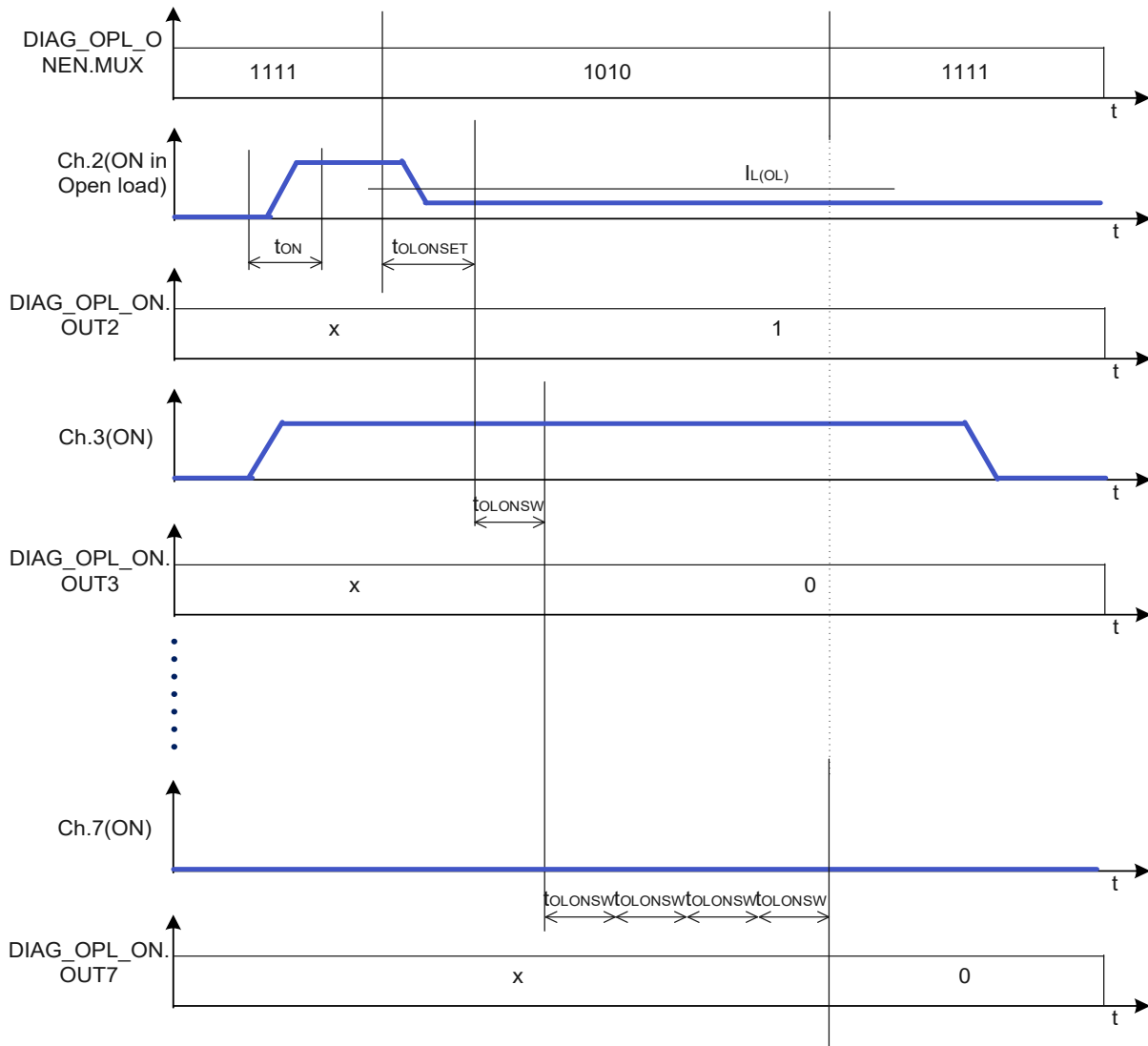
Figure 9.4 Open Load at ON timings (diagnosis loop - channels driven by micro-controller directly)
