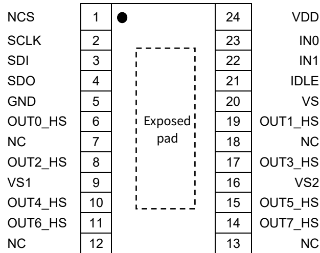
Figure 1.1 NSD56080 Package
