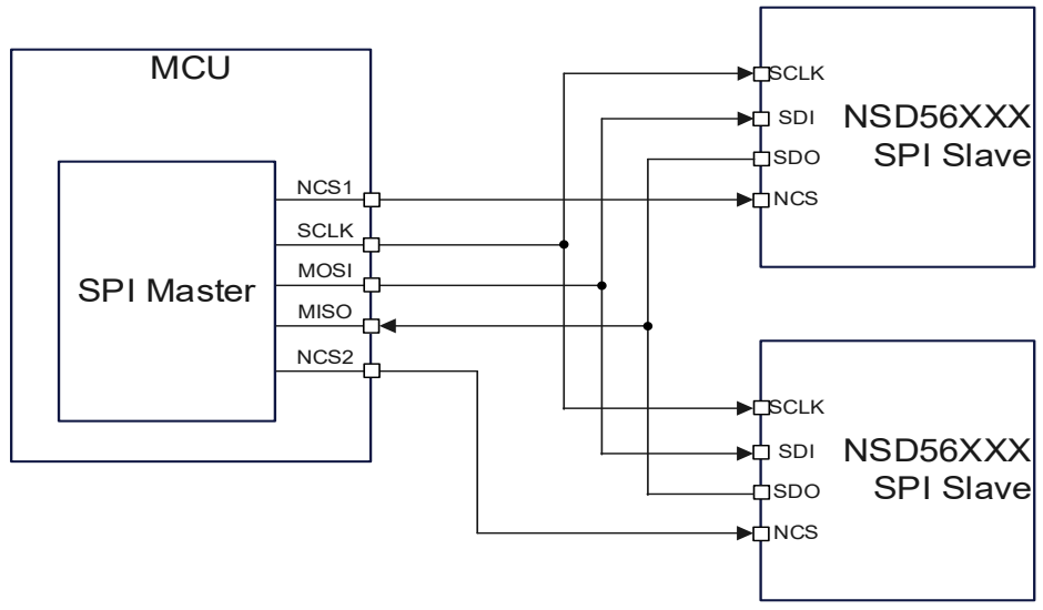
Figure 10.2 Parallel Configuration
