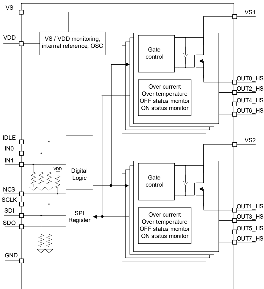
Figure 2.1 Block Diagram of NSD56080
