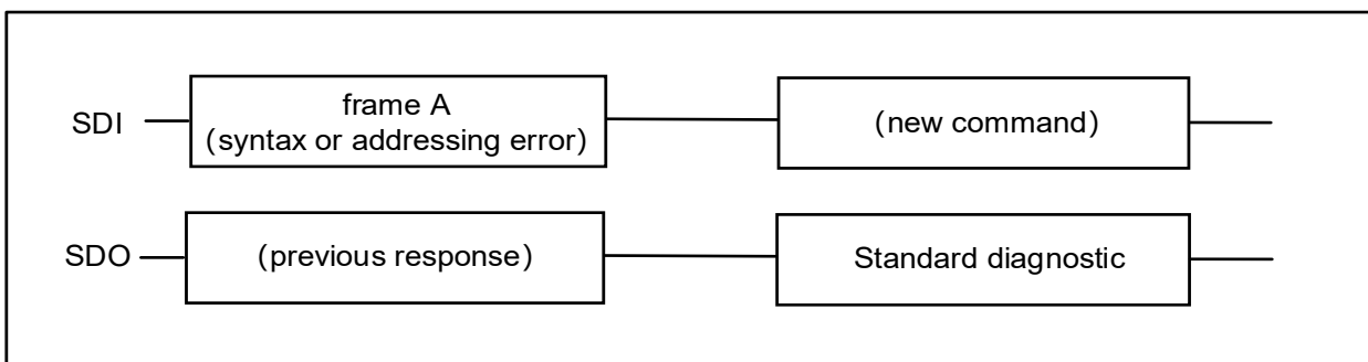
Figure 10.10 NSD56080 response after a command syntax error
