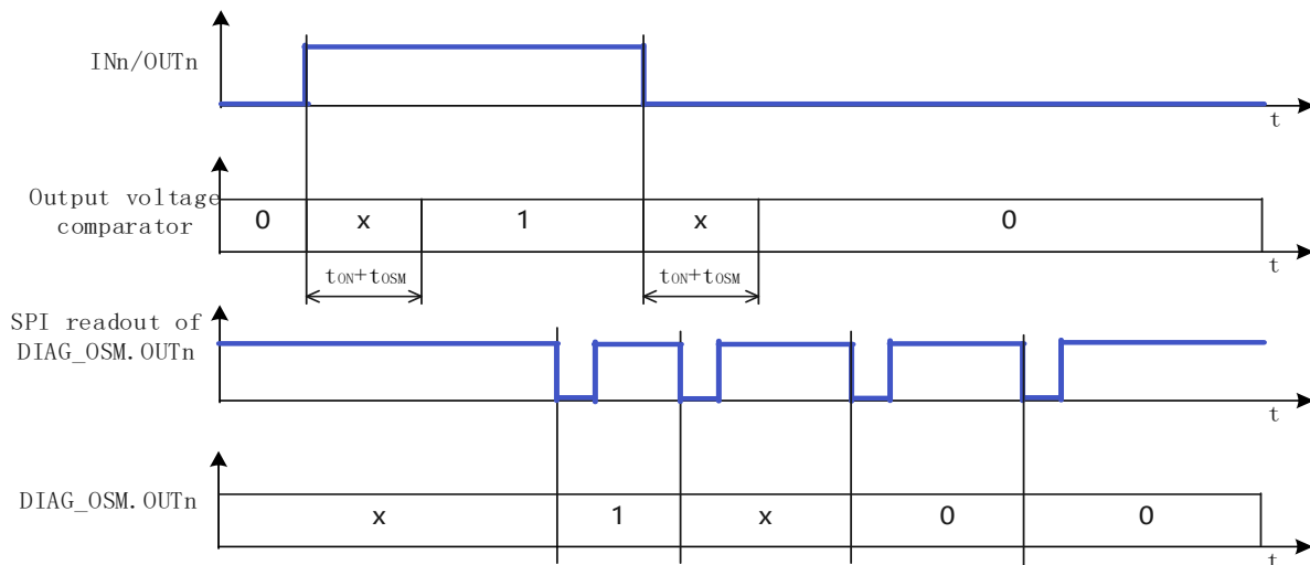
Figure 9.1 Output Status Monitor timing
