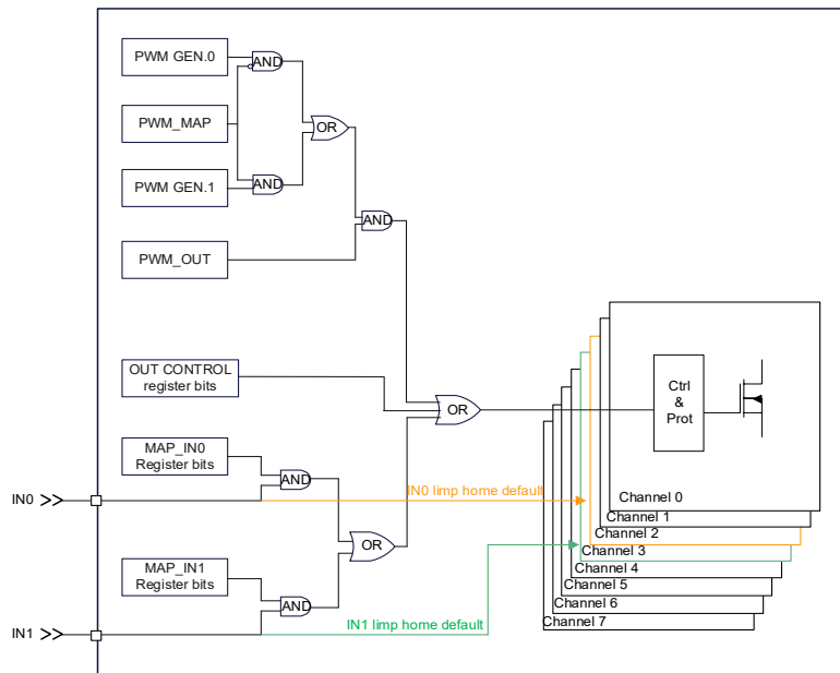
Figure 7.4 PWM Generator Mappings
