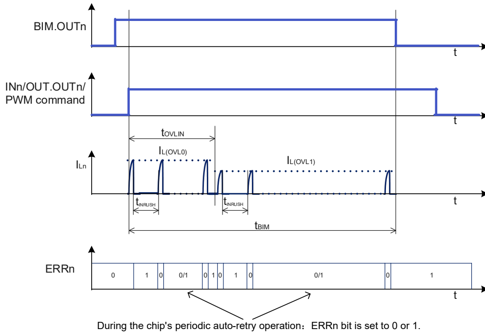
Figure 7.3 Bulb Inrush Mode (BIM) operation
