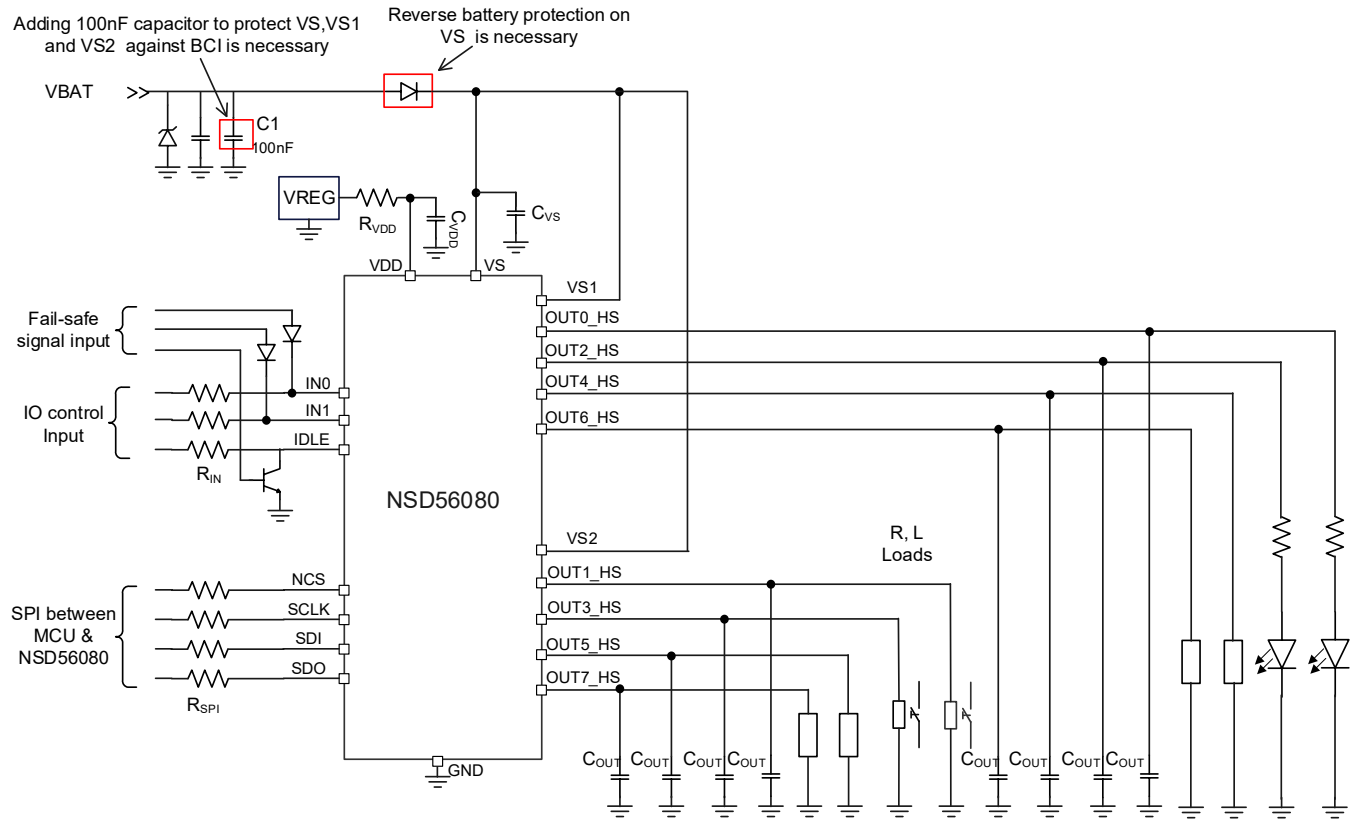
Figure 3.1 NSD56080 Application Diagram
