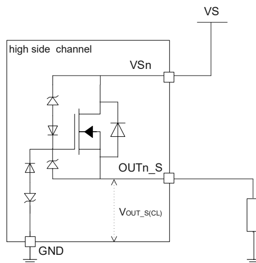
Figure 7.2 Output Clamp concept
