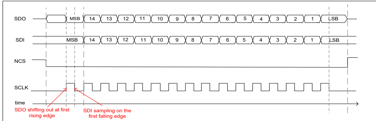
Figure 10.1 Serial Peripheral Interface
