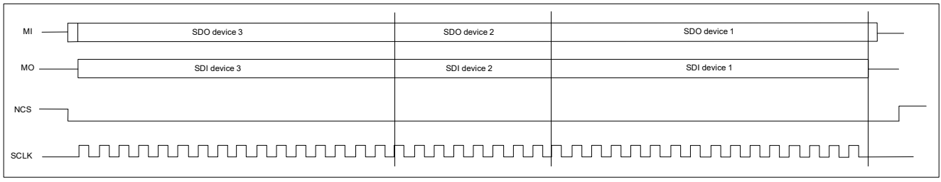
Figure 10.4 Data Transfer in Daisy Chain Configuration
