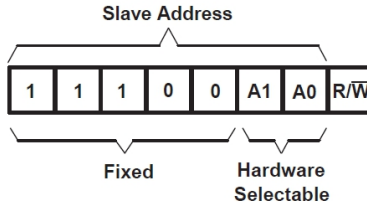
Figure 6.7 NCA9545 Address
