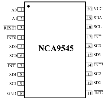
Figure 1.1 NCA9545 Package
