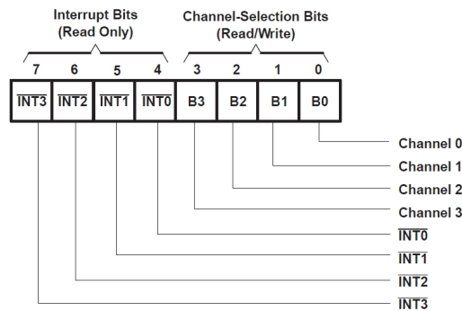
Figure 6.8 Control Register
