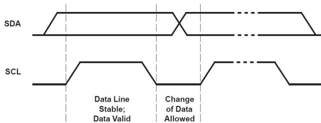
Figure 6.1 Bit Transfer
