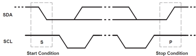
Figure 6.2 Definition of Start and Stop Conditions
