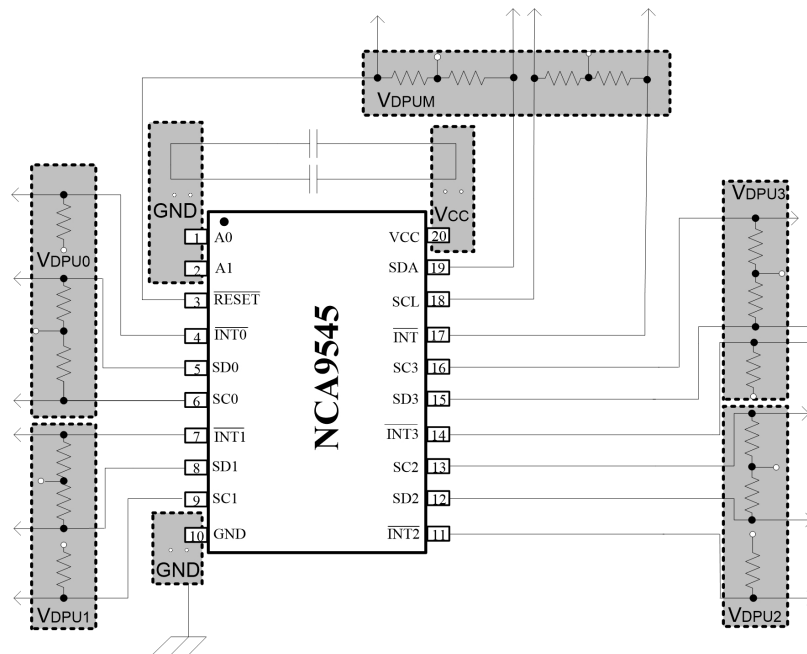
Figure 8.1 Typical Application PCB
