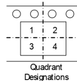
Figure 12.1 Tape and Reel Information of TSSOP
