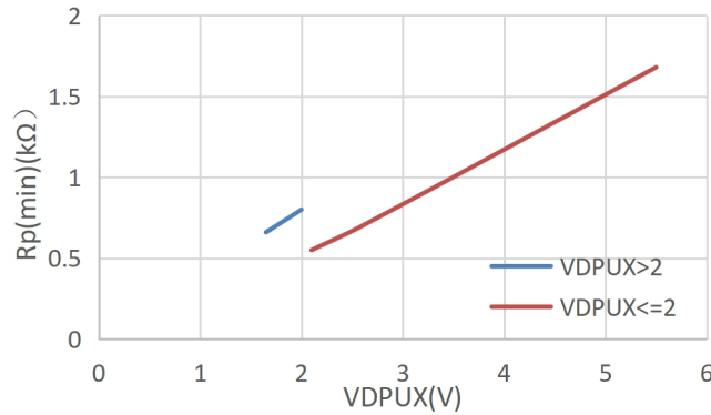
Figure 7.4 Minimum Pull-Up resistance( R_{p(min)} ) vs Pull-up reference voltage( V_{DPUX} )
