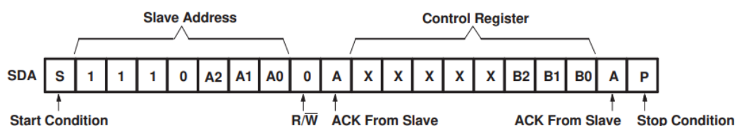
Figure 7.6 Write Control Register
