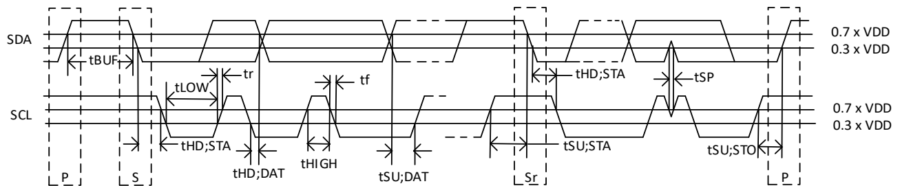
Figure 6.1 Definition of timing on I²C-bus
