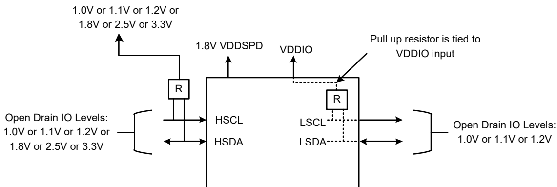
Figure 5 Open-Drain Interface; Internal Pullup Resistor
