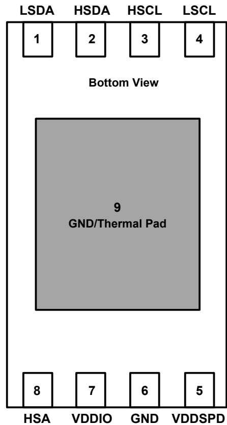
Figure 2 Bottom view for NCA95118A
