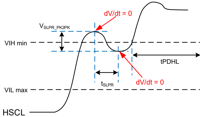
Figure 26 Slope Reversal on HSCL at VIH
