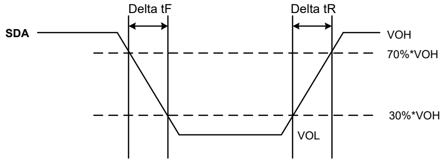
Figure 25 Rise and Fall Timing Parameter Definition
