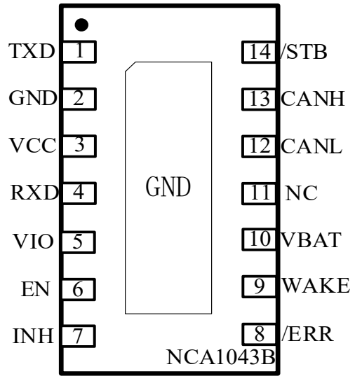
Figure 1.1.2 NCA1043B DFN14 Package
