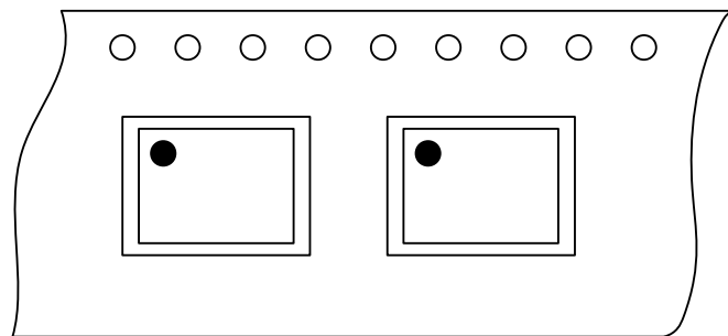
Figure 11.1 Tape and Reel Information of SOP14
