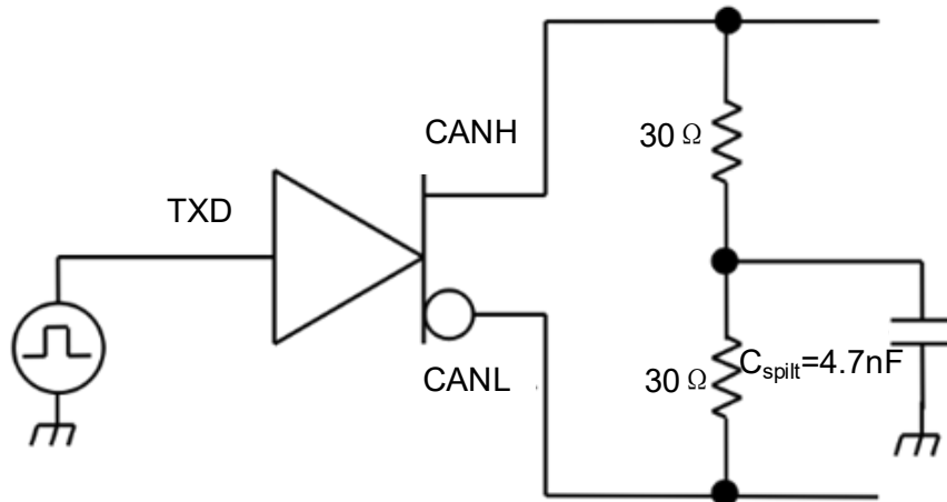
Figure 6.5 Transceiver Driver Symmetry Test Circuit
