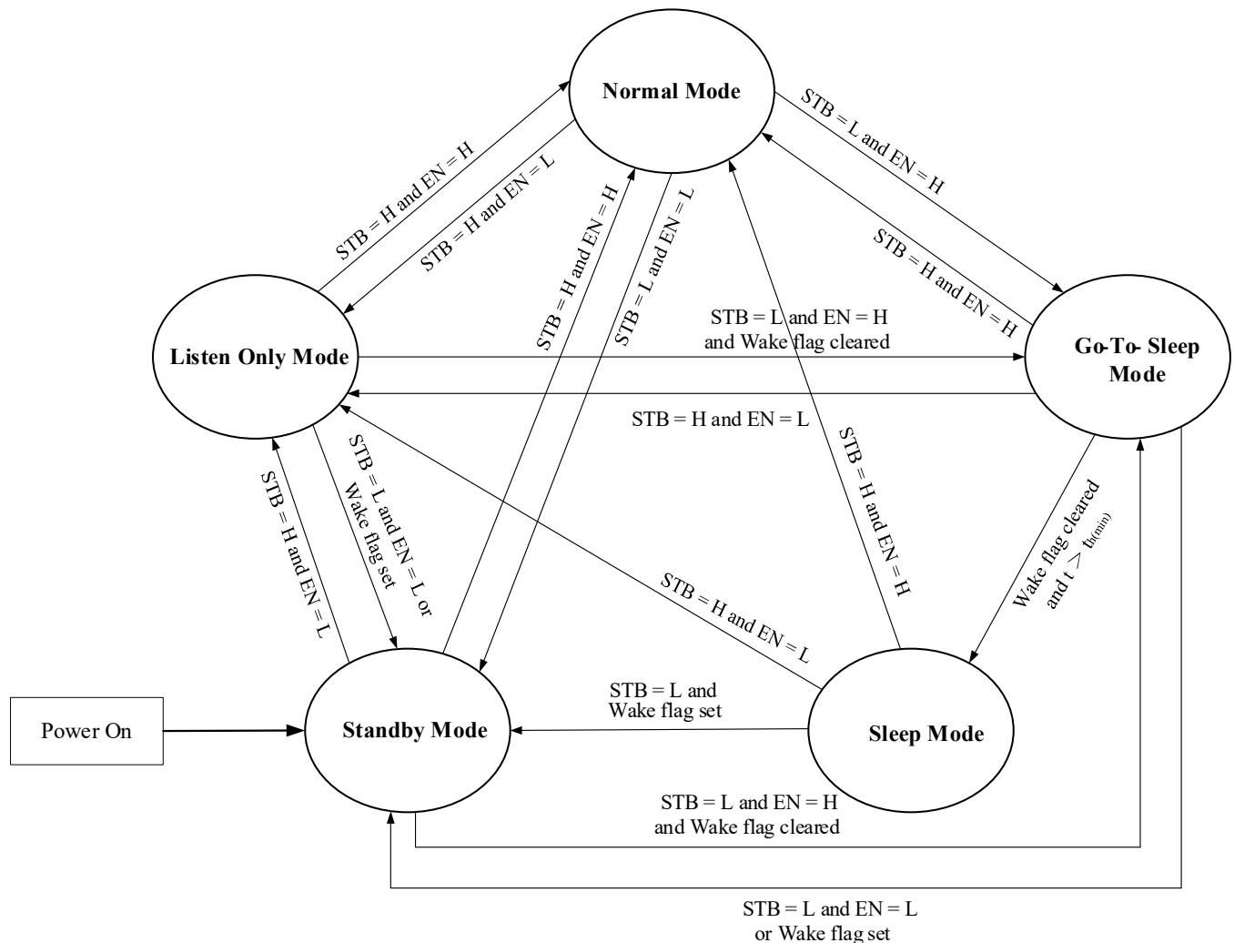
Figure 7.1 Mode transition
