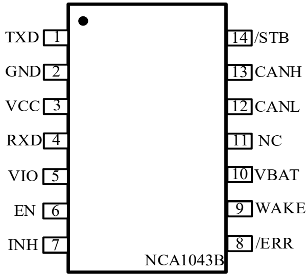
Figure 1.1.1 NCA1043B SOP14 Package
