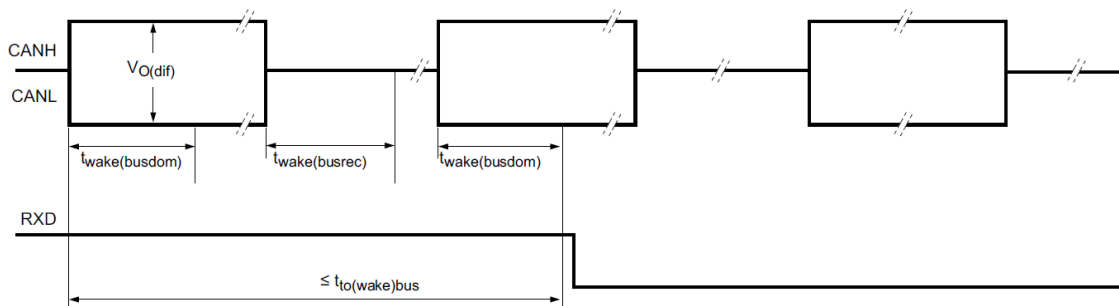
Figure 7.2 Wake-up timing
