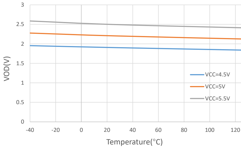
Figure 6.8 V OD(D) vs temperature (R Load = 60Ω)
