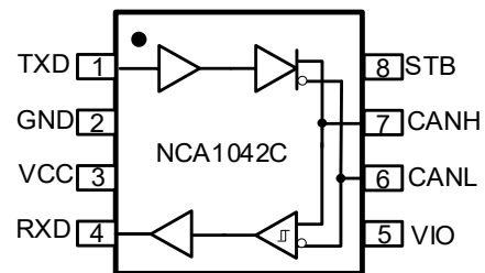
Figure 1. NCA1042C Block Diagram
