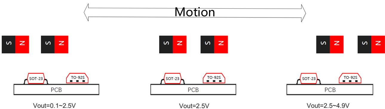
Figure.4 Feature Description
