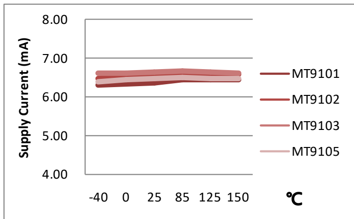
Figure.6 Supply Current vs. Temperature (At V CC =5.0V)
