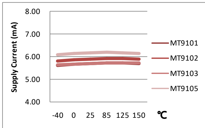
Figure.7 Supply Current vs. Temperature (At V CC =3.3V)
