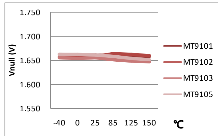
Figure.9 V null vs. Temperature (At V CC =3.3V)
