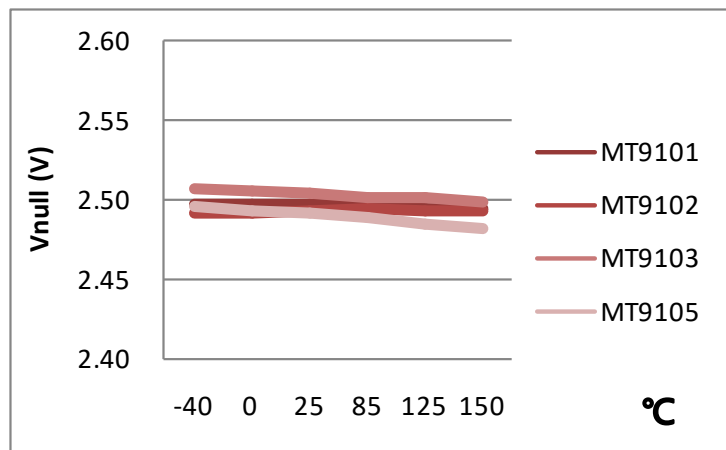
Figure.8 V null vs. Temperature (At V CC =5.0V)
