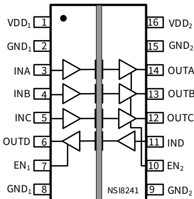
Figure 1.2 NSI8241 Package
