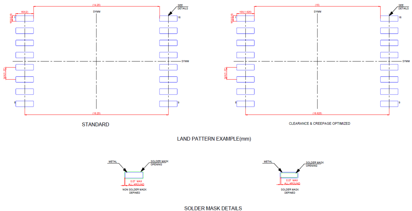
Figure 9.2 SOP16(600mil)/SOWW16 Package Board Layout Example
