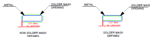
SOLDER MASK DETAILS
