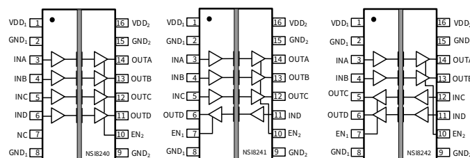
Figure 1. NSI824x Block Diagram
