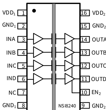
Figure 1.1 NSI8240 Package
