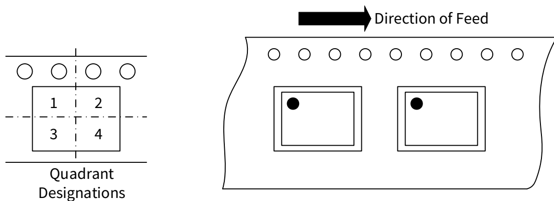
Figure 12.3 Tape Information of SOP16(150mil)
