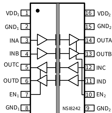
Figure 1.3 NSI8242 Package
