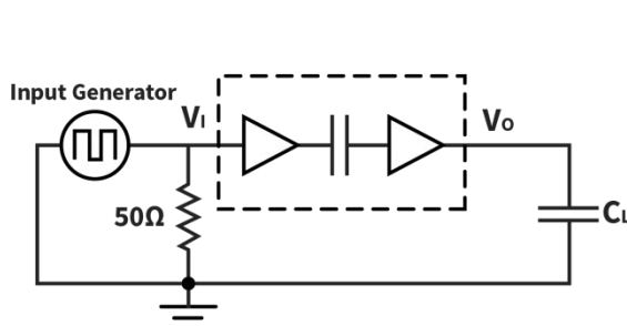
Figure 5.9 Switching Characteristics Test Circuit and Waveform
