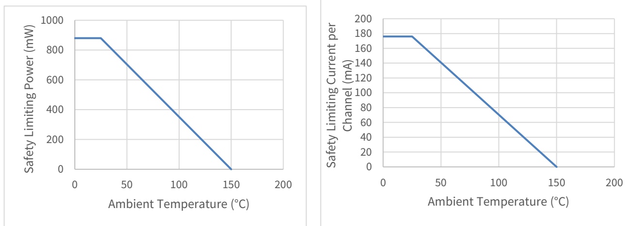
Figure 6.2 NSI824xS Thermal derating Curve, Dependence of Safety Limiting Values with Case Temperature per DIN EN IEC 60747-17 (VDE 0884-17).
