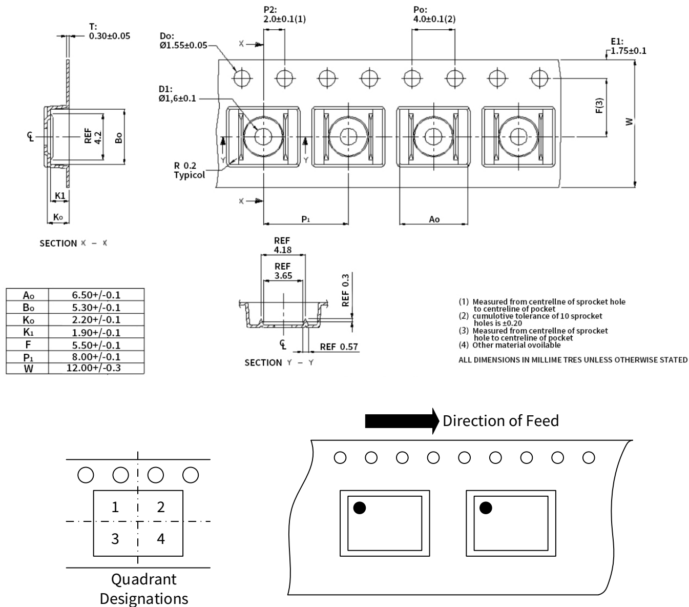
Figure 12.2 Tape Information of SSOP16
