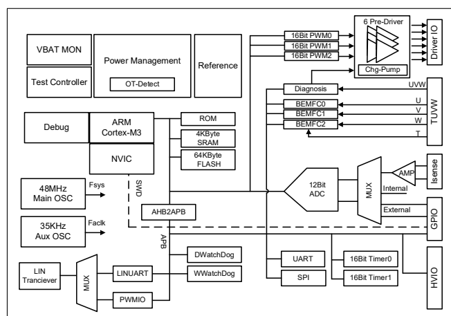
Figure 1. NSUC1602 Block Diagram
