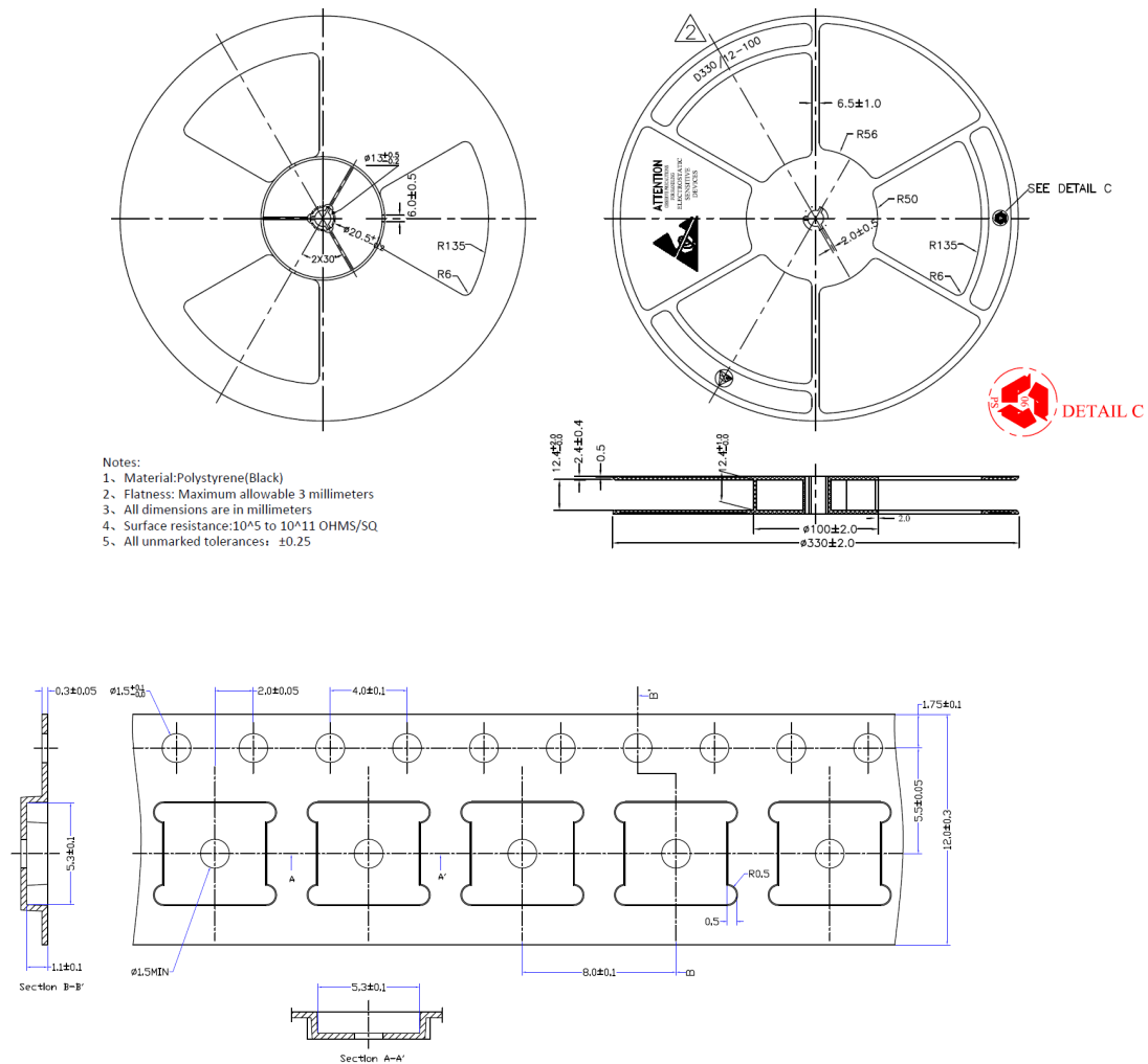
Figure 11.1 Tape and Reel Information of QFN40
