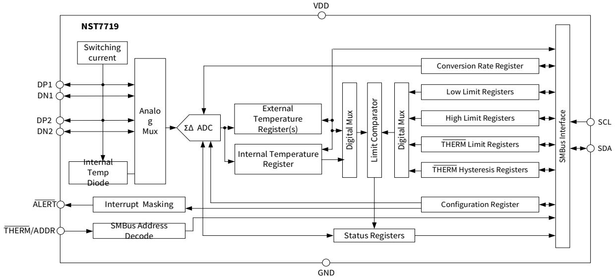
Figure 4.1 NST7719 Functional Block Diagram
