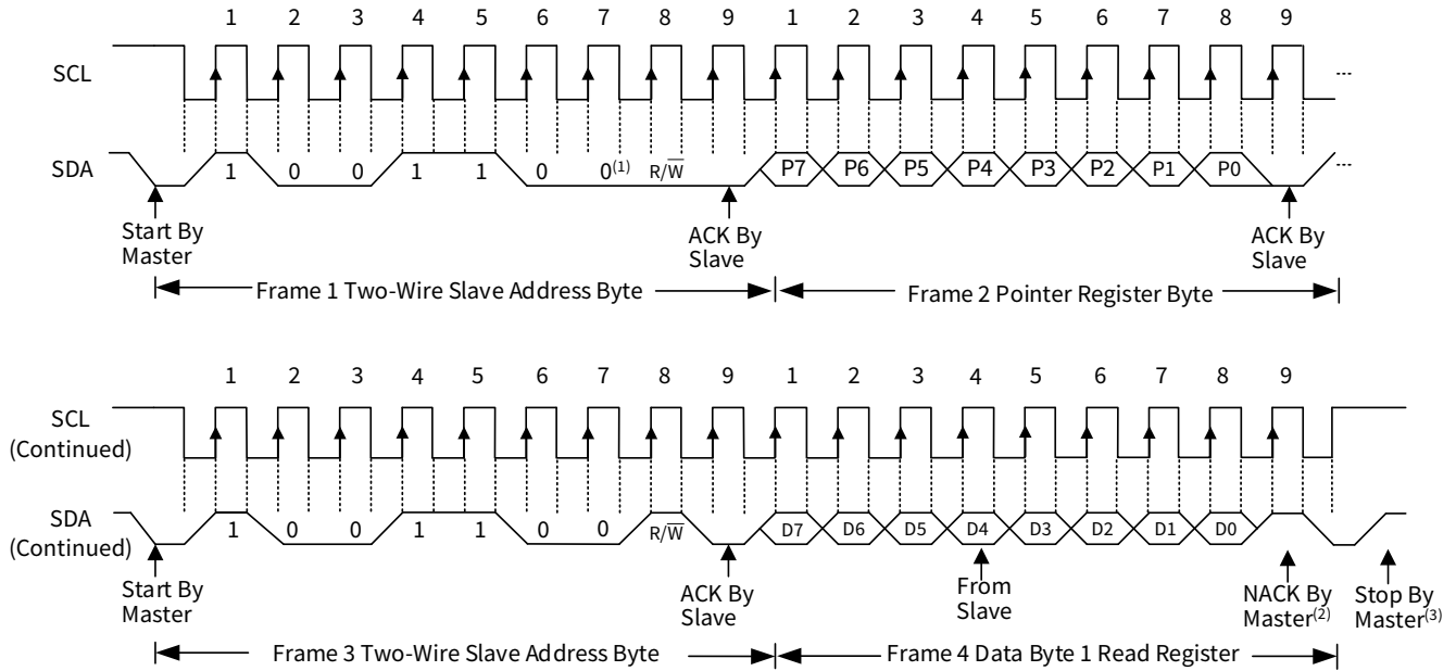
Figure 4.6. Two-Wire Timing Diagram for the NST7719 Write Word Format
