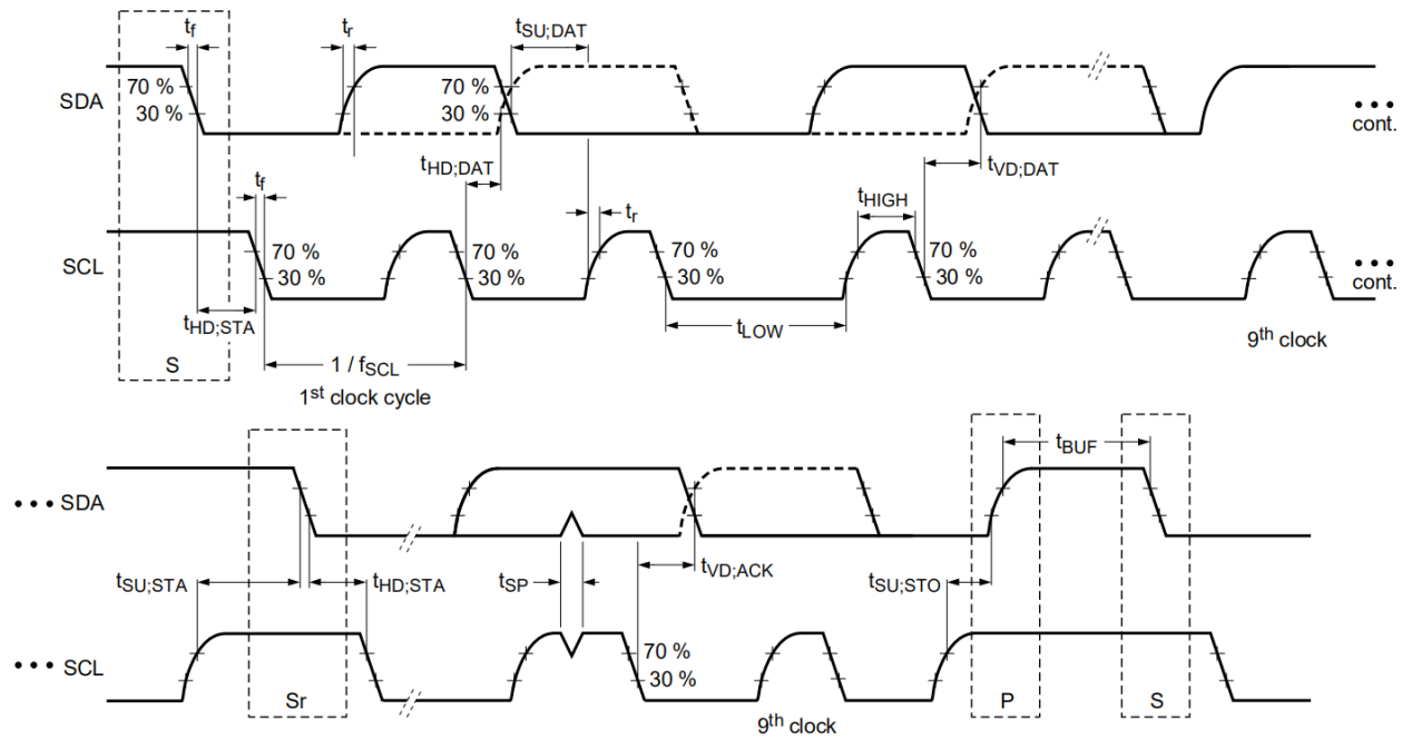
Figure 3.1 I 2 C Timing Diagram
