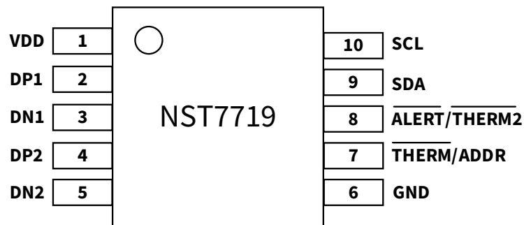
Figure 1.1 NST7719 Package
