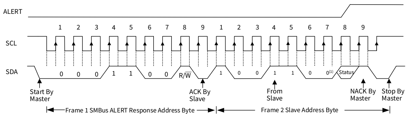
Figure 4.9. SMBus Alert Function
