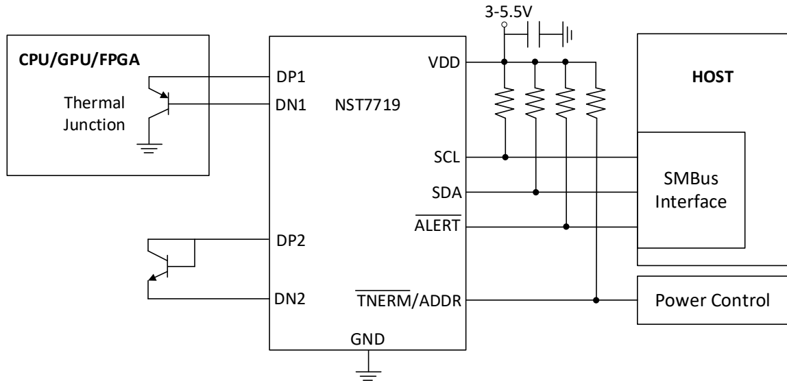
Figure 6.1. NST7719 Basic Connections Using a Discrete Remote Transistor
