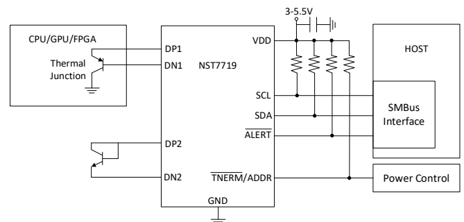
Figure 1. NST7719 Application Diagram
