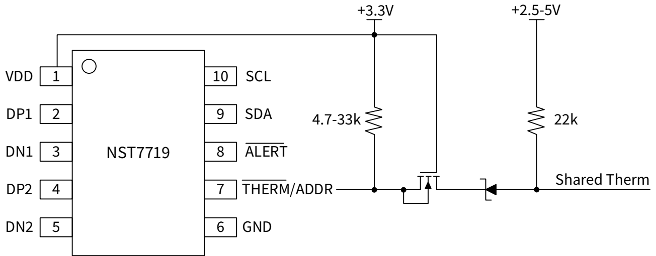
Figure 4.8. Isolating THERMPin
