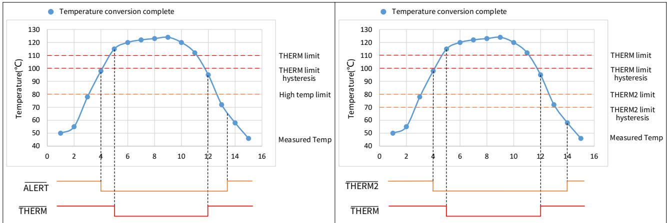
Figure 4.4 ALERT and THERM interrupt operation
