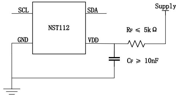
Figure 6.1 Noise Reduction
