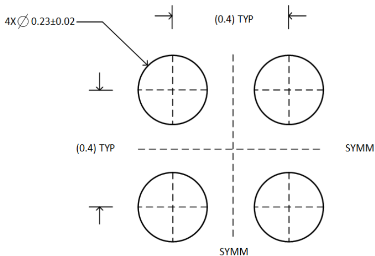
LAND PATTERN EXAMPLE SCALE:50X
