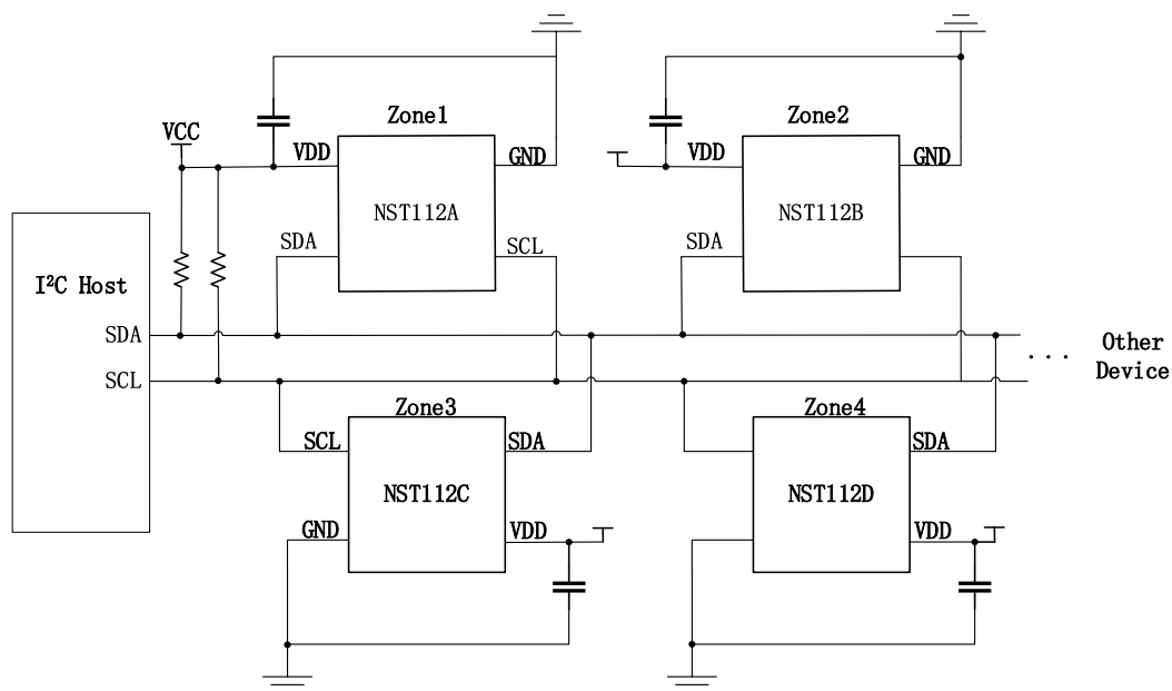
Figure 6. 2 Application Diagram
