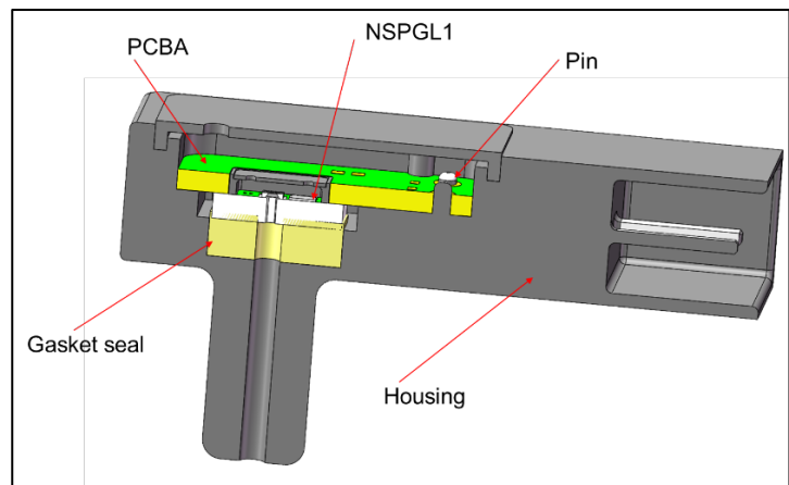
Figure 7.3 PCBA & Sensor Structure Design
