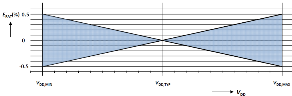
Figure 6.3 Ratiometric Error
