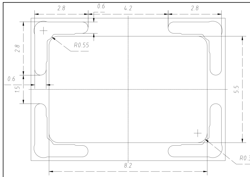
Figure 7.2 Footprint mm
