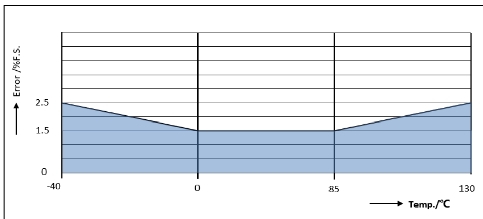
Figure 6.4 Accuracy for Pressure Acquisition
