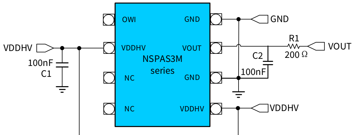
Fig 6.1 Application Circuit
