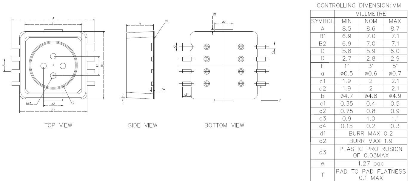
Fig 7.1 Package Outline mm
