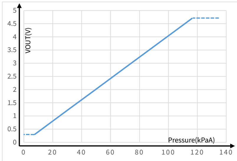
Fig 5.2 NSPAS3M115RRD1 Transfer Function
