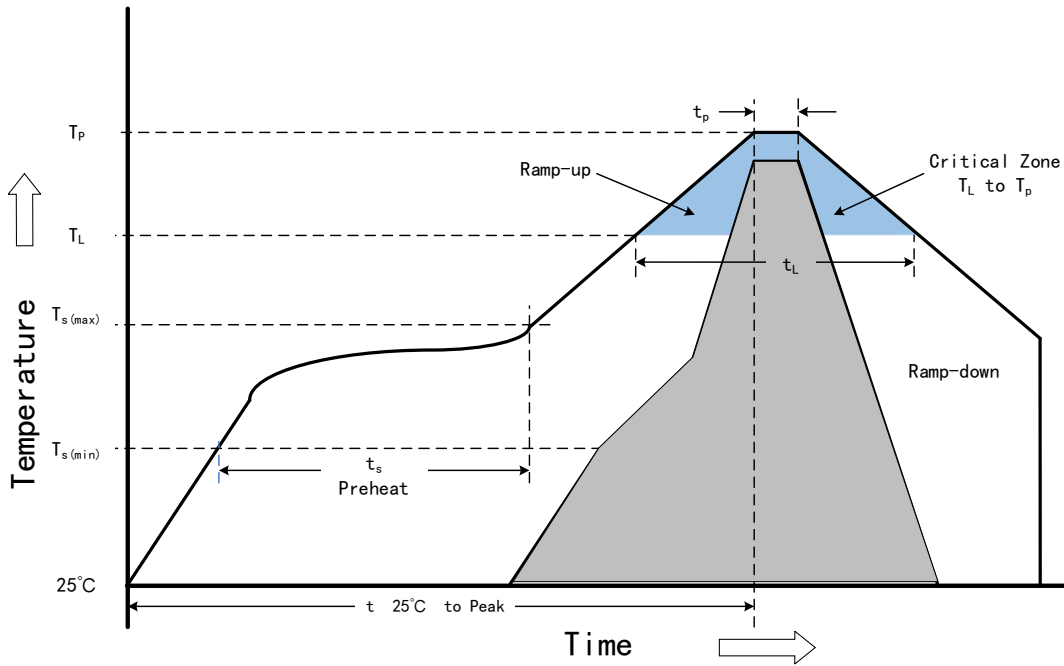
Fig 6.3 Soldering Profile
