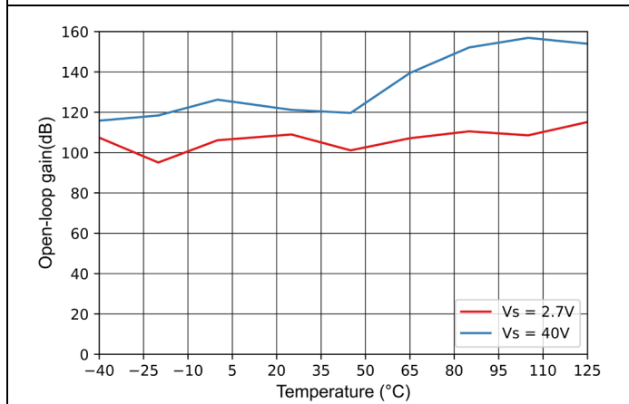
Figure 7-11 Open-Loop Voltage Gain vs Temperature
