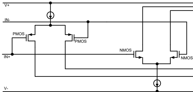
Figure 8-5 NSOPA901x-Q1 Rail-to-rail Input Stage
