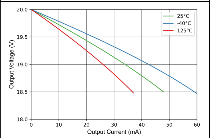
Figure 7-34 Output Voltage Swing vs Output Sourcing Current
