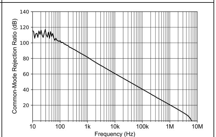
Figure 7-6 Common-Mode Rejection Ratio vs Frequency
