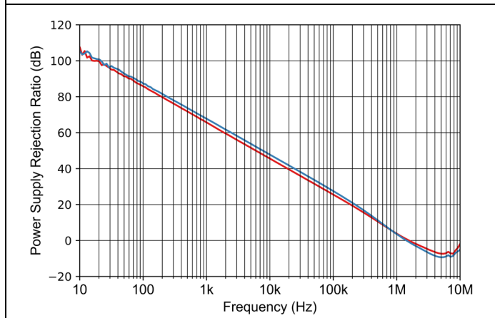
Figure 7-9 Power-Supply Rejection Ratio vs Frequency
