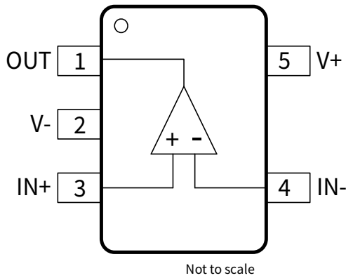
Figure 1-1 NSOPA9011-Q1 5-Pin SOT-23 Package Top View
