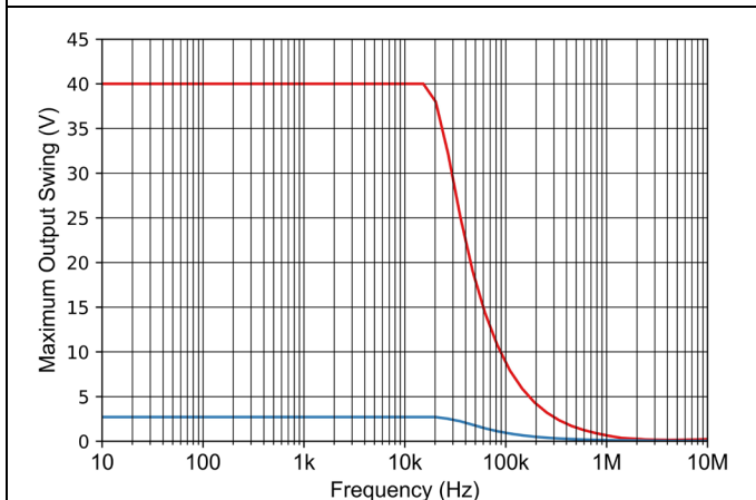
Figure 7-17 Maximum Peak Output Voltage vs. Frequency
