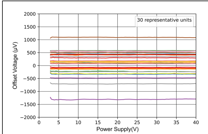
Figure 7-7 Offset Voltage vs Power Supply ( V_{CM} = V_- )
