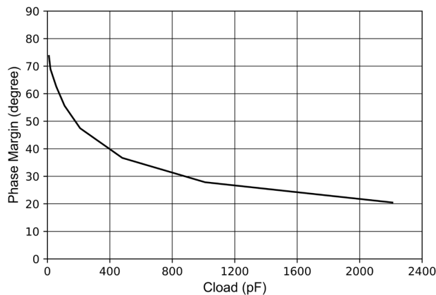
Figure 8-7 NSOPA901x-Q1 Phase Margin vs Capacitive Load
