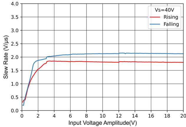
Figure 8-4 Slew-Rate vs Input Voltage Amplitude
