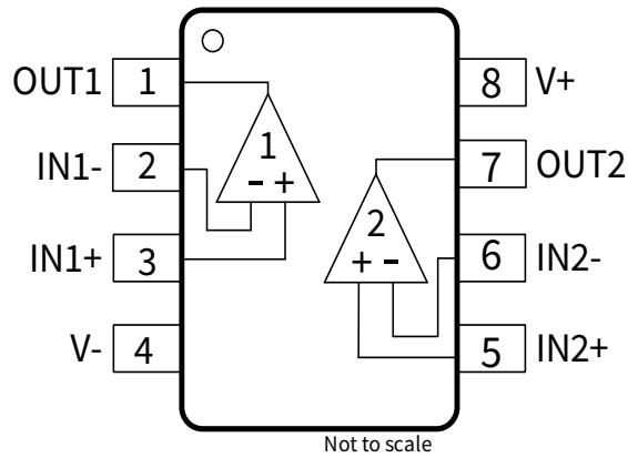
Figure 1-3 NSOPA9012-Q1 8-Pin SOP and MSOP Package Top View
