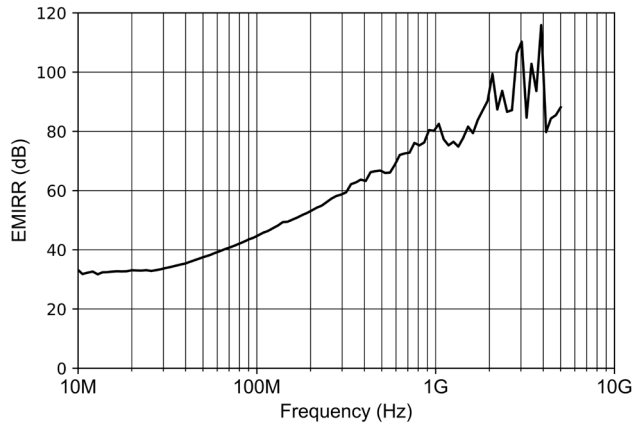
Figure 8-6 NSOPA901x-Q1 EMIRR vs Frequency
