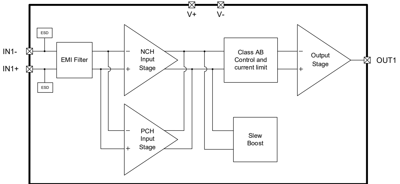
Figure 8-1 NSOPA901x-Q1 Functional block Diagram (One channel is shown)
