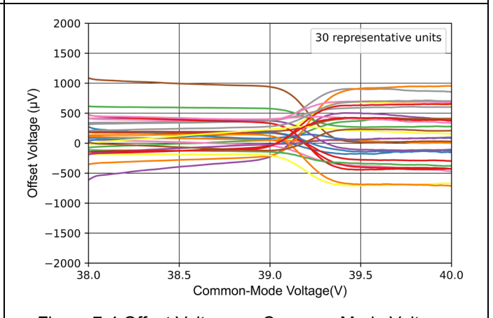
Figure 7-4 Offset Voltage vs Common-Mode Voltage, Transition
