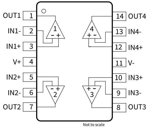
Figure 1-4 NSOPA9014-Q1 14-Pin SOP and TSSOP Package Top View
