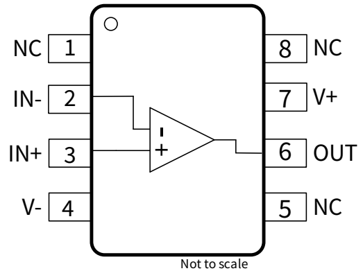
Figure 1-2 NSOPA9011-Q1 8-Pin SOP Package Top View
