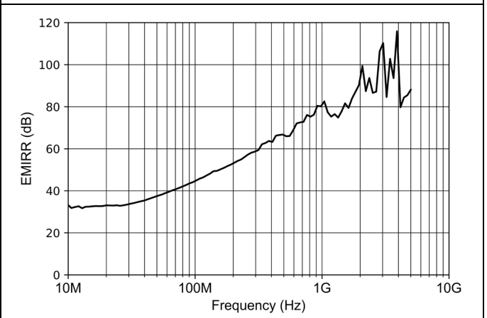
Figure 7-36 EMIRR vs Frequency
