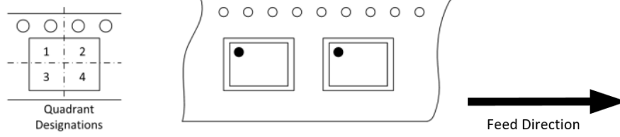
Figure 10.1 Tape and Reel Information of SOW16
