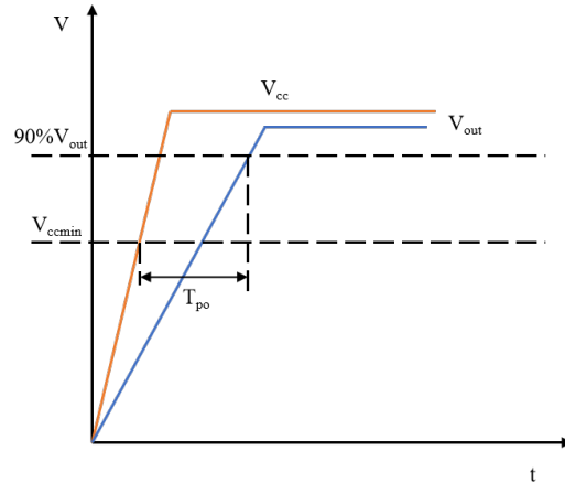
Figure 6.6 NSM2015 Power-on time
