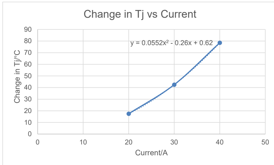
Figure 7.4 NSM2015 Estimation function of junciton temperature at different currents (PCB is in worst case)
