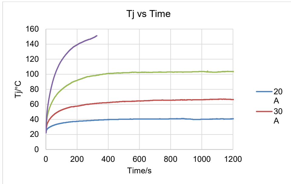
Figure 7.3 NSM2015 Junction temperature vs. Different continues current
