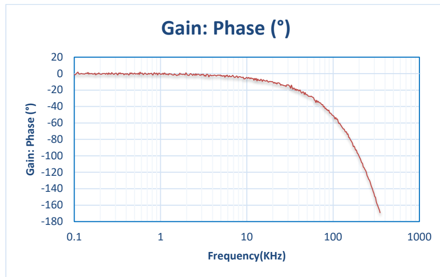
Figure 6.5 NSM2015 Phase frequency response curve
