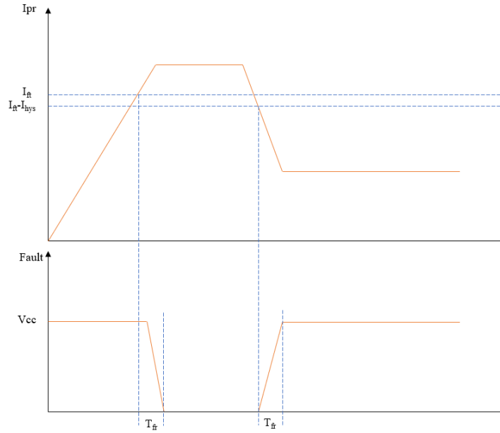
Figure 6.1 NSM2015 Overcurrent Performance
