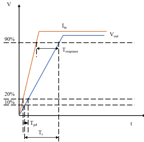
Figure 6.7 NSM2015 response time
