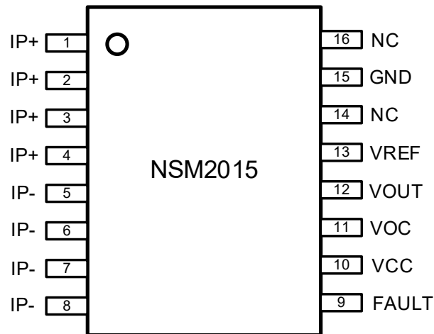
Figure 1.1 NSM2015 Package
