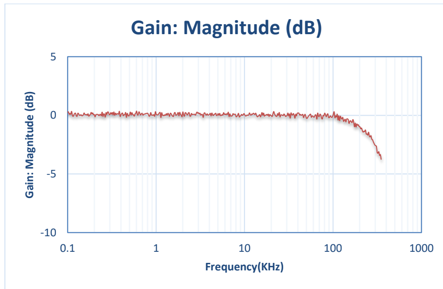
Figure 6.4 NSM2015 Amplitude frequency response curve
