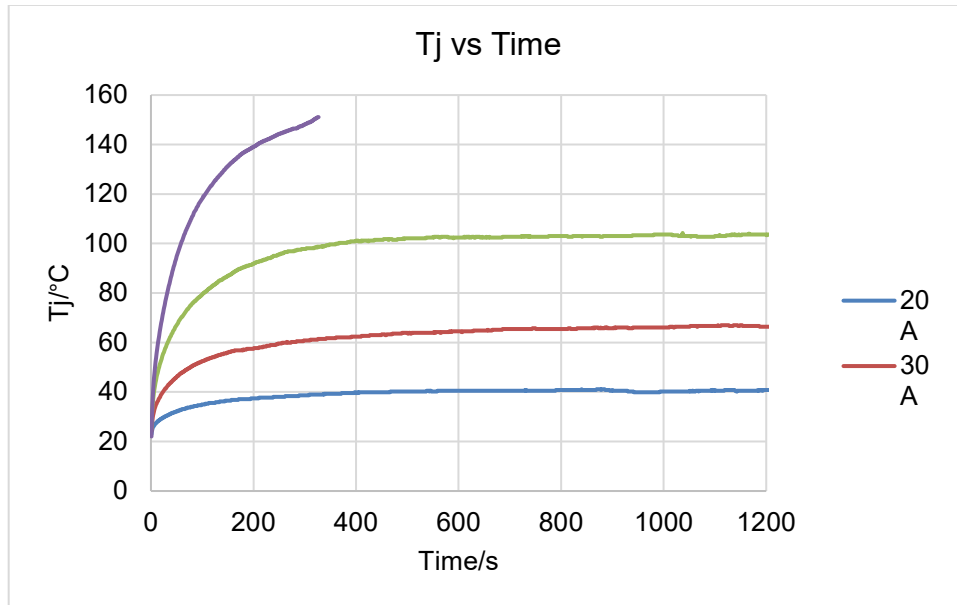
Figure 7.3 NSM2015-Q1 Junction temperature vs. Different continues current
