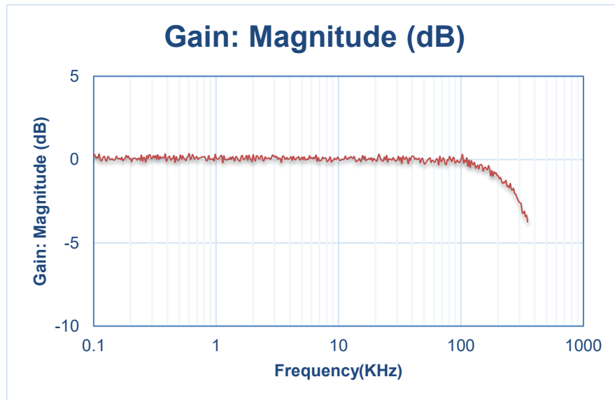
Figure 6.4 NSM2015-Q1 Amplitude frequency response curve
