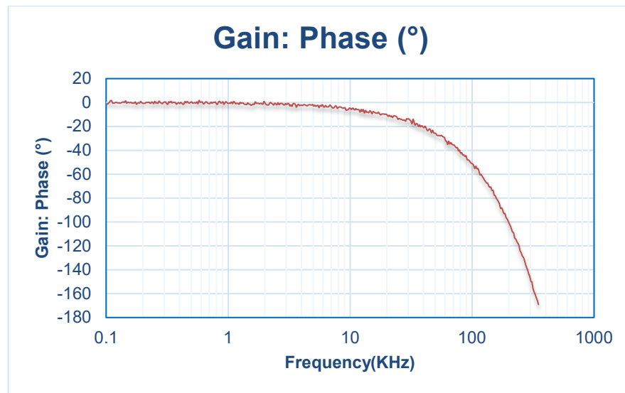
Figure 6.5 NSM2015-Q1 Phase frequency response curve
