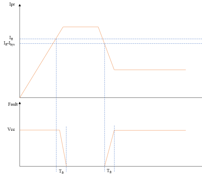
Figure 6.1 NSM2015-Q1 Overcurrent Performance
