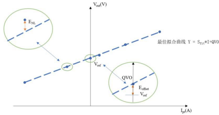
Figure 6.8 NSM2015-Q1 Sensitivity and error
