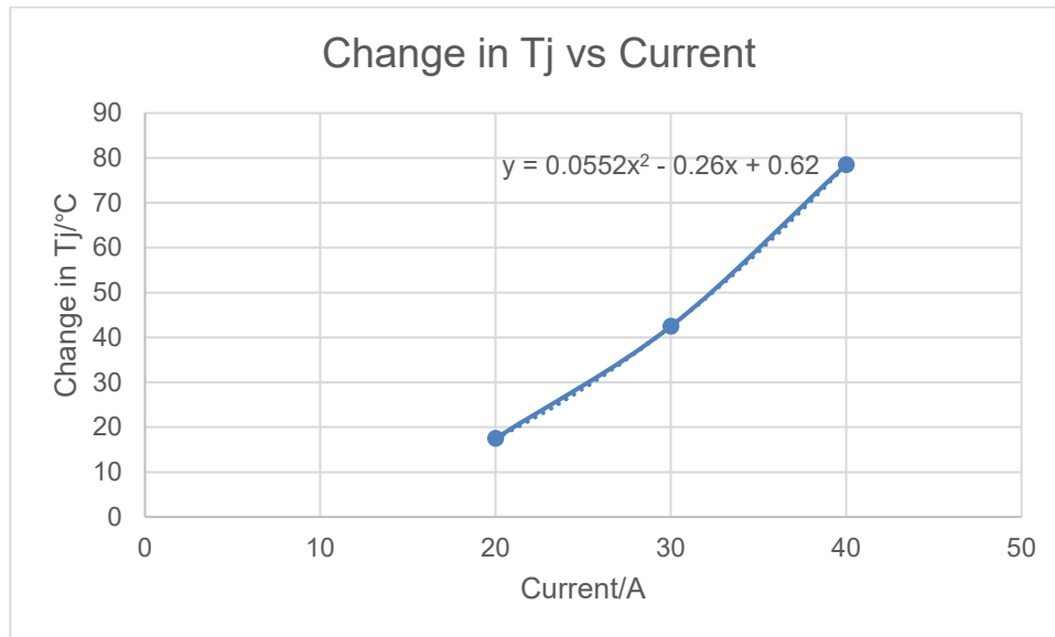
Figure 7.4 NSM2015-Q1 Estimation function of junction temperature at different currents (PCB is in worst case)
