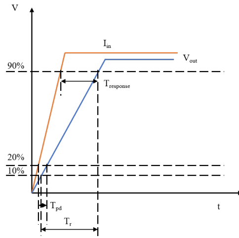
Figure 6.7 NSM2015-Q1 response time
