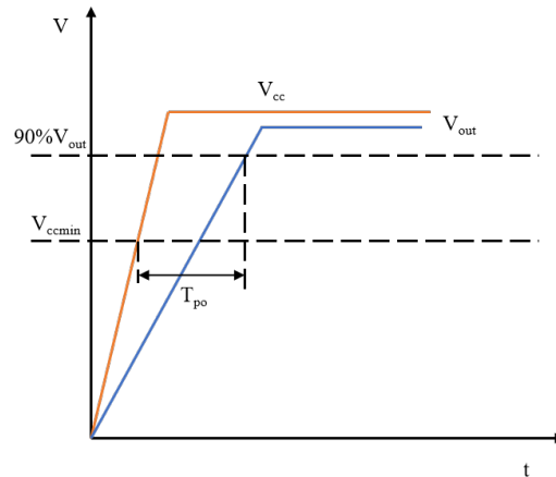
Figure 6.6 NSM2015-Q1 Power-on time
