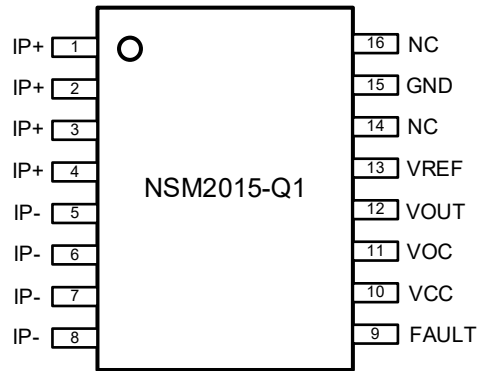
Figure 1.1 NSM2015-Q1 Package
