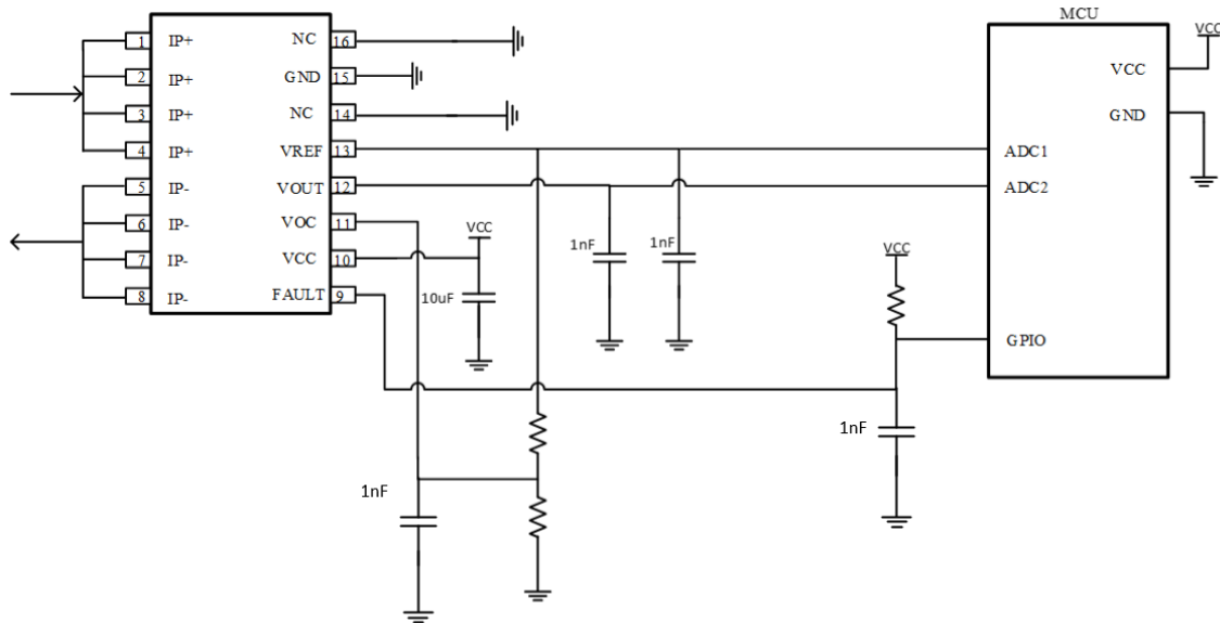
Figure 7.1 Typical Application Diagram of Fixed Output Mode
