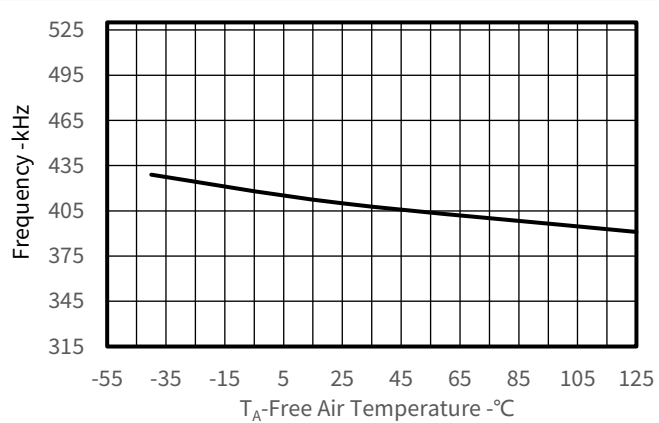
Figure 8.8 Average Frequency vs Free-Air Temperature
