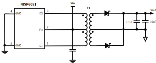
Figure 11.3 Unstable output voltage and low load current
