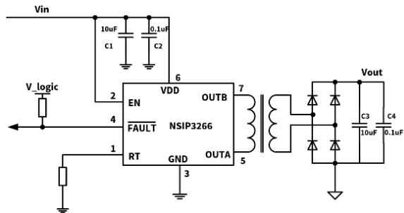
Figure 11.1 Typical Application Schematic
