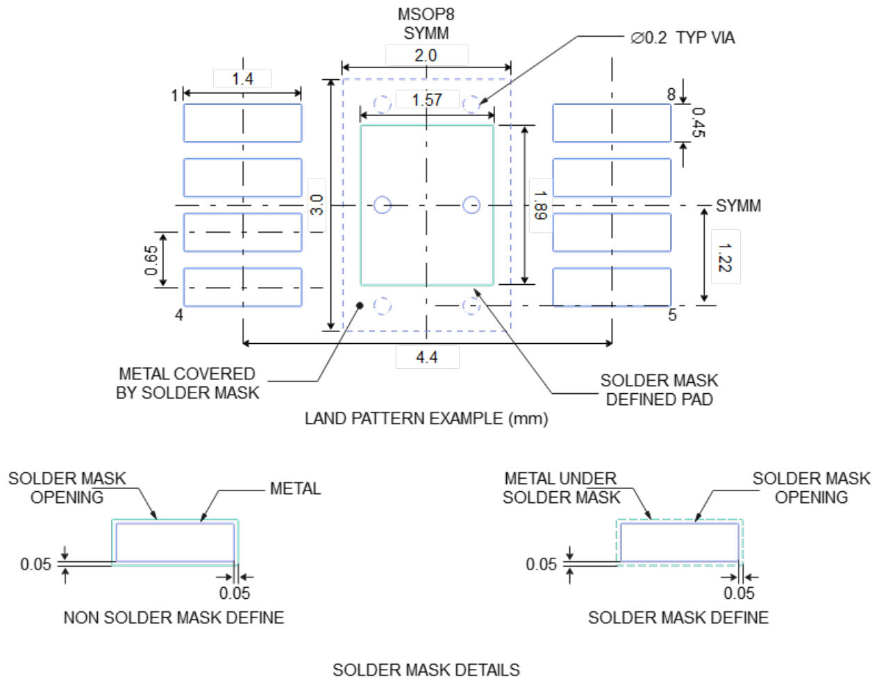
Figure 12.2 HMSOP8 Package Board Layout Example
