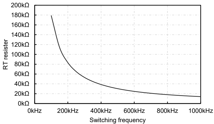
Figure 10.4 RT resister vs Switching frequency
