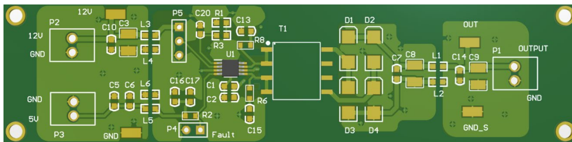
Figure 11.2 Layout Example of 2-Layer Board (NSIP3266E-Q1)
