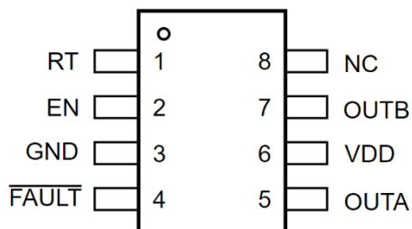
Figure 1.1 NSIP3266E-Q1 Pin Configuration
