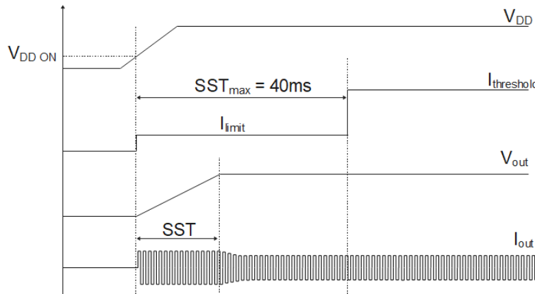
Figure 10.2 Waveform schematic diagram during soft start time
