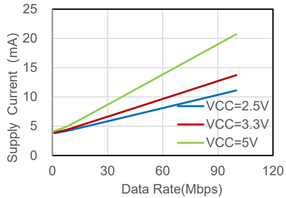
Figure 6.8 NSI8330 VDD2 Supply Current vs Data Rate
