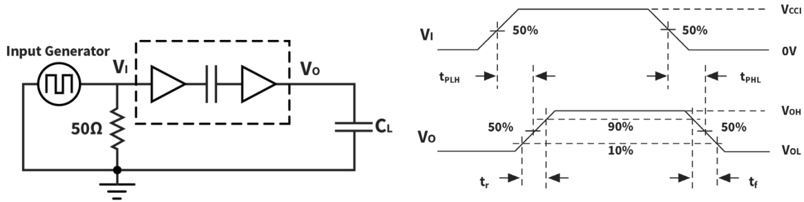
Figure 6.13 Switching Characteristics Test Circuit and Waveform
