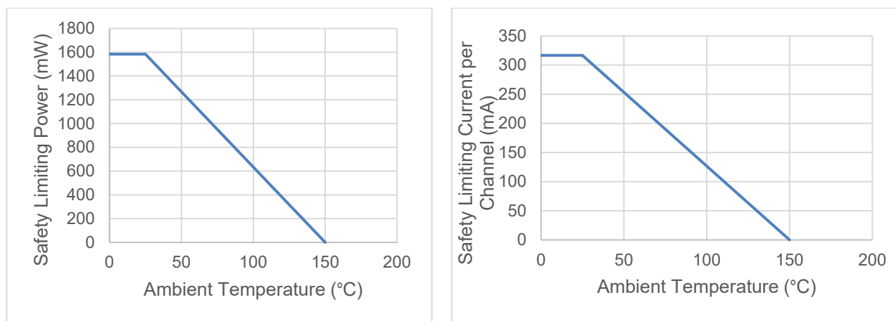
Figure 7.1 NSI83x Thermal derating Curve, Dependence of Safety Limiting Values with Case Temperature per DIN EN IEC 60747-17 (VDE 0884-17).
