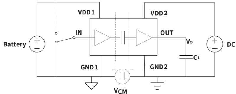
Figure 6.15 Common-Mode Transient Immunity Test Circuit
