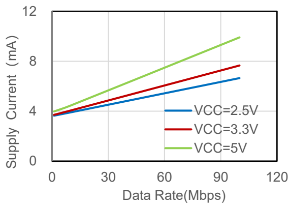
Figure 6.7 NSI8330 VDD1 Supply Current vs Data Rate
