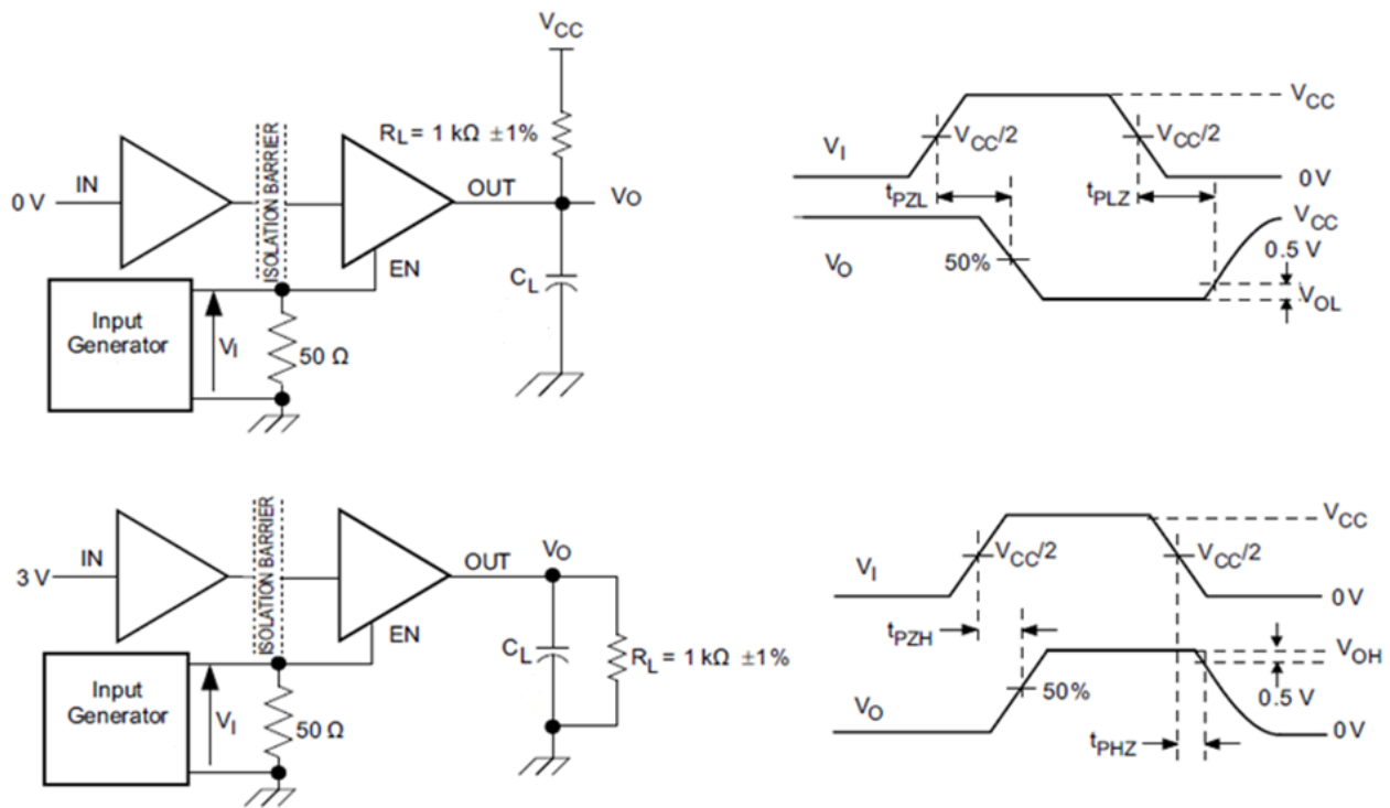
Figure 6.13 Switching Characteristics Test Circuit and Waveform
