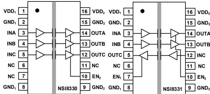
Figure 1.4 NSI8330 Package
