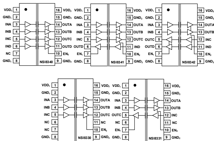
Figure 1. NSI83x Block Diagram
