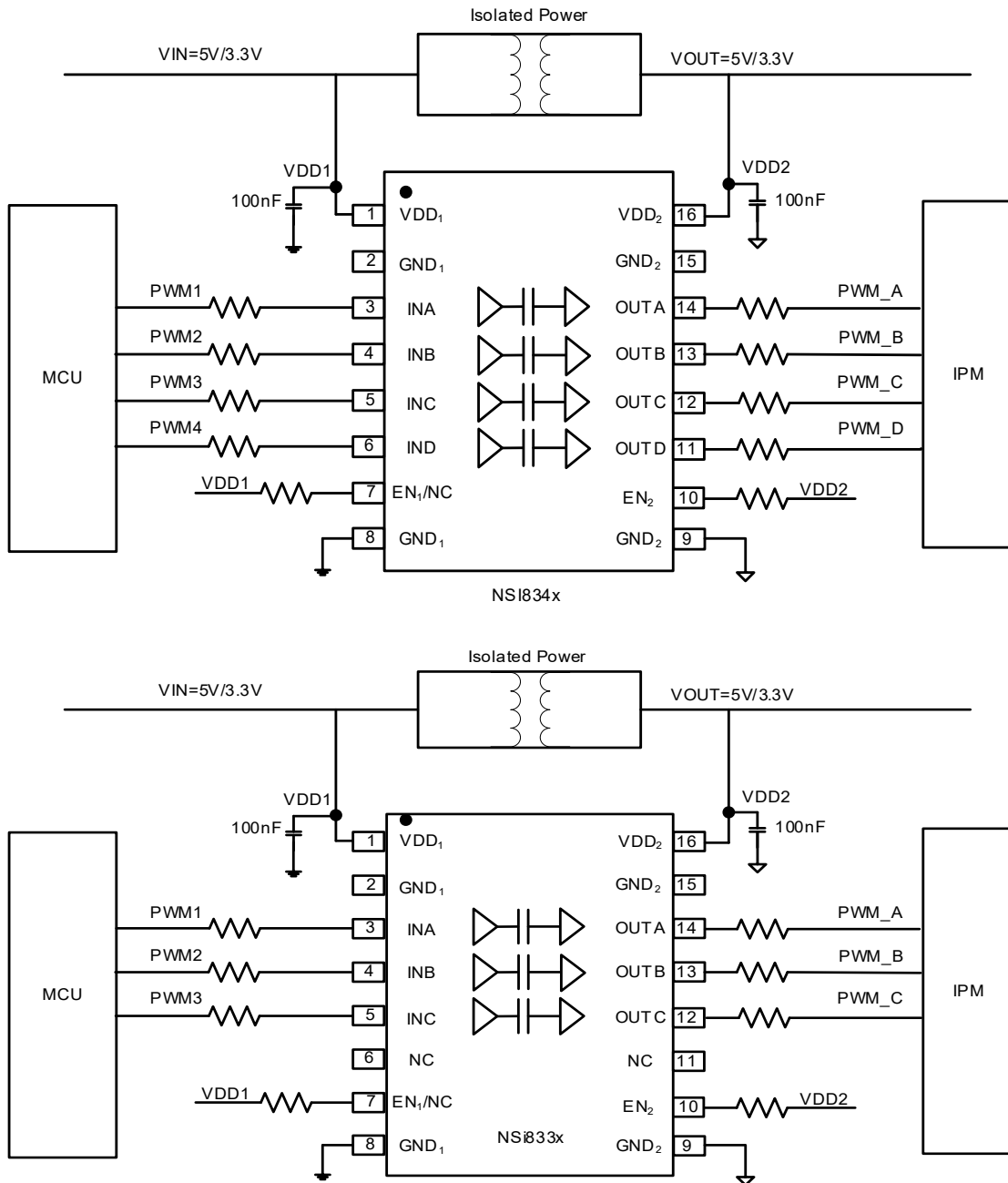
Figure 9.1 Typical PWM isolation circuit for IPM
