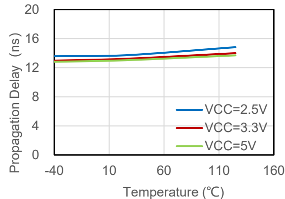
Figure 6.12 Falling Edge Propagation Delay Vs Temp
