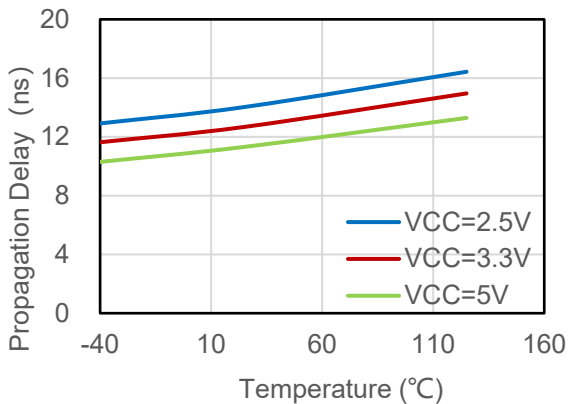
Figure 6.11 Rising Edge Propagation Delay Vs Temp
