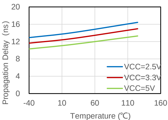
Figure 6.11 Rising Edge Propagation Delay Vs Temp
