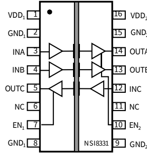
Figure 1.2 NSI8331 Package
