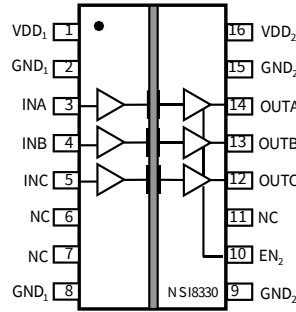
Figure 1.1 NSI8330 Package
