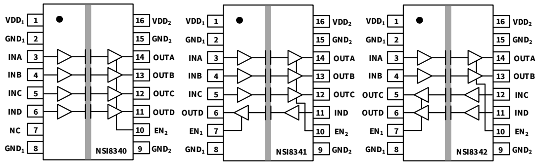
Figure 1.3 NSI8340 Package
