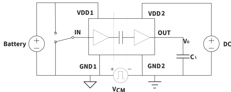
Figure 6.15 Common-Mode Transient Immunity Test Circuit
