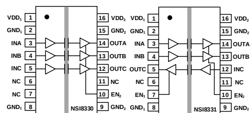
Figure 1. NSI833x Block Diagram
