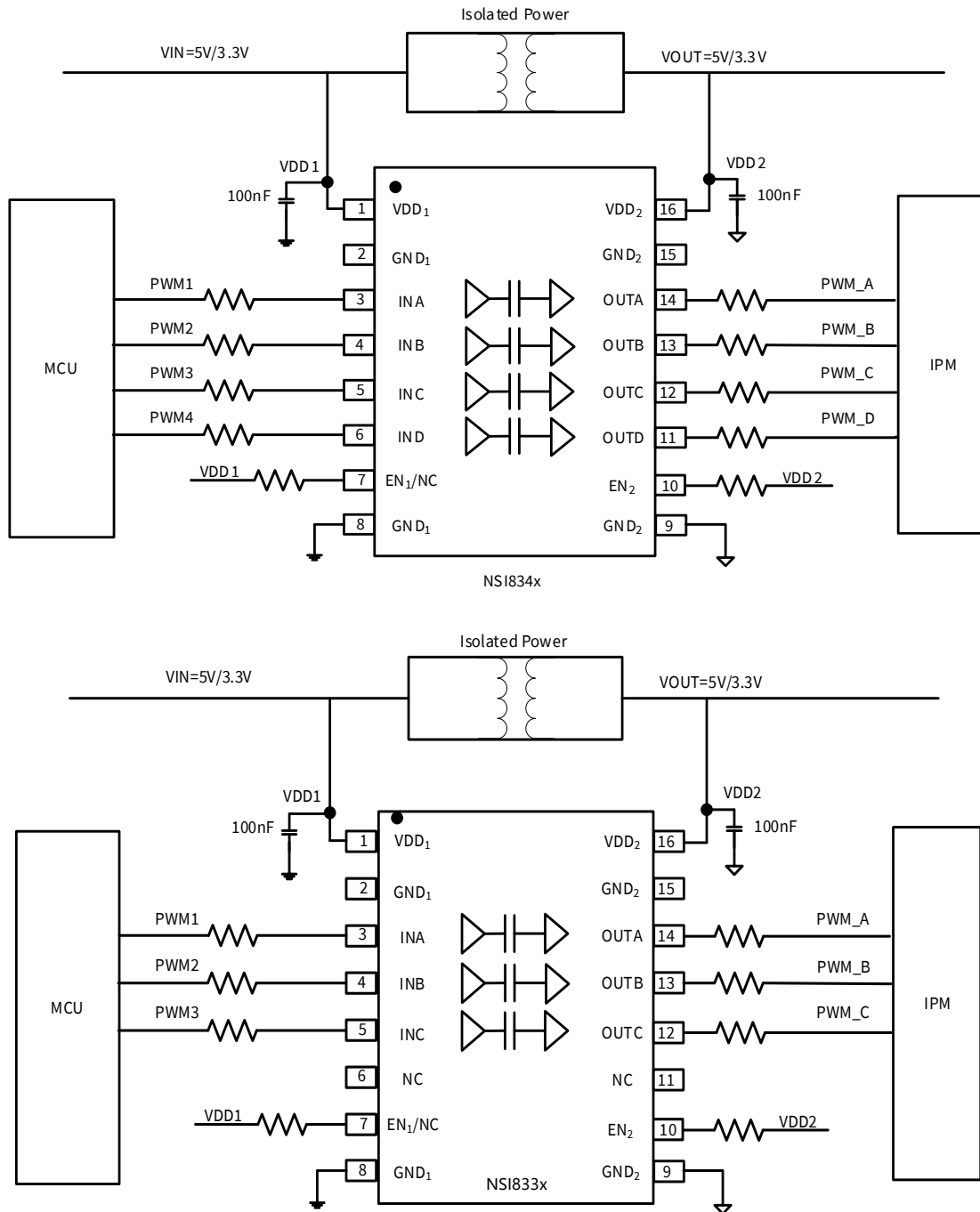
Figure 9.1 Typical PWM isolation circuit for IPM
