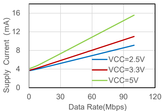
Figure 6.5 NSI83x2 VDD1 Supply Current vs Data Rate
