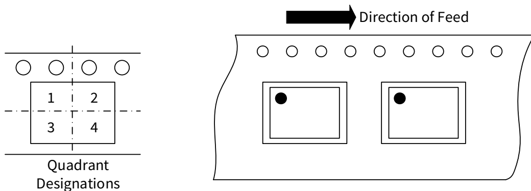
Figure 13.2 Tape Information of SSOP16
