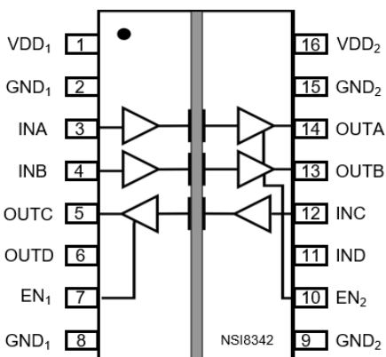
Figure 1.5 NSI8342 Package
