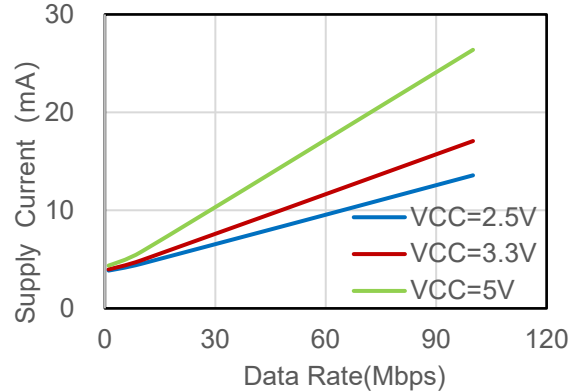
Figure 6.2 NSI83x0 VDD2 Supply Current vs Data Rate
