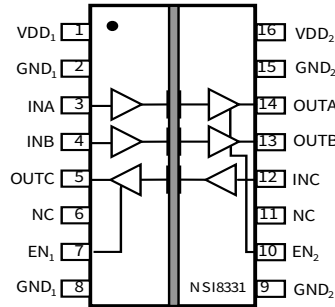
Figure 1.2 NSI8331 Package
