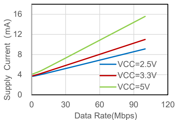
Figure 6.6 NSI83x2 VDD2 Supply Current vs Data Rate
