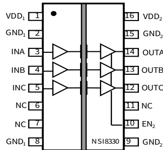
Figure 1.1 NSI8330 Package
