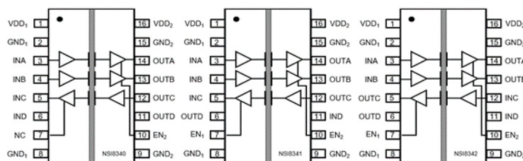
Figure 2. NSI834x Block Diagram
