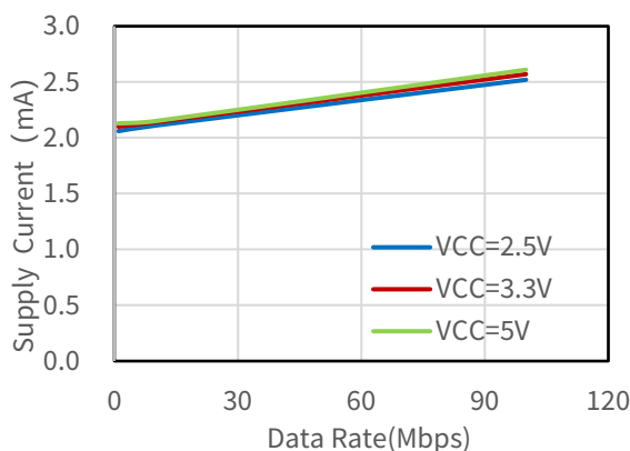
Figure 6.5 NSI8210-DSWVR VDD1 Supply Current vs Data Rate
