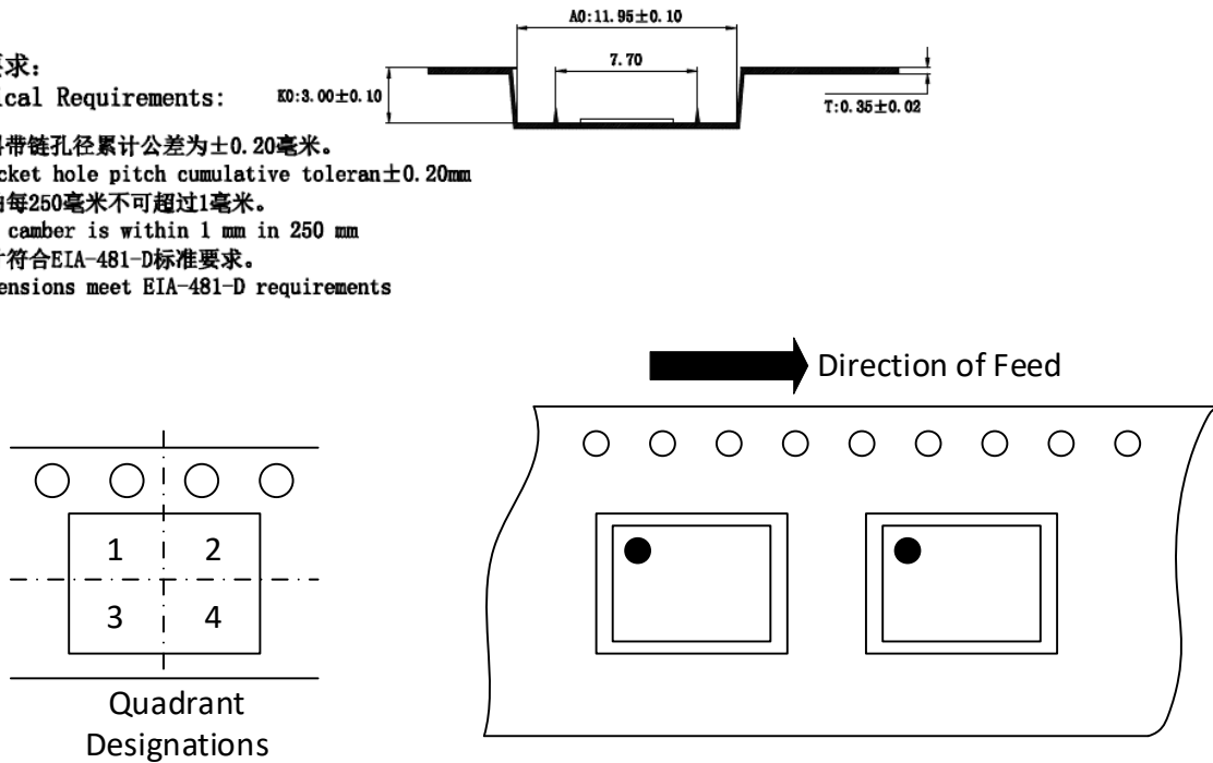
Figure 13.3 Tape Information of SOW8(300mil)
