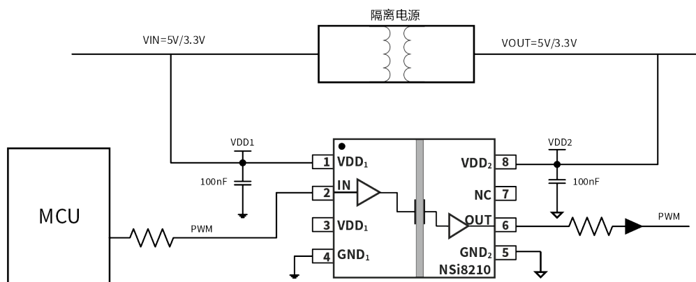
Figure9.1 Typical PWM isolation circuit
