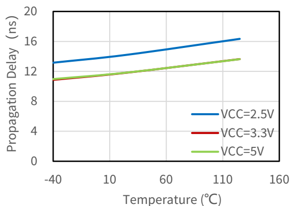
Figure 6.3 NSI8210-DSPR Rising Edge Propagation Delay Vs Temp
