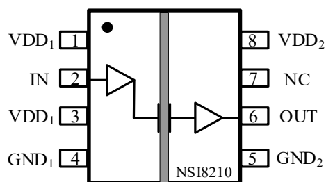
Figure 1.1 NSI8210 Package
