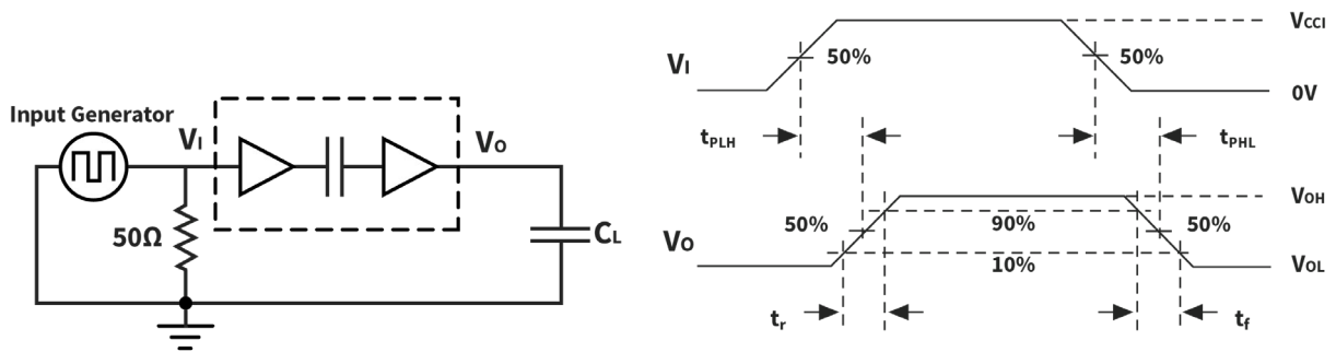
Figure 6.9 Switching Characteristics Test Circuit and Waveform
