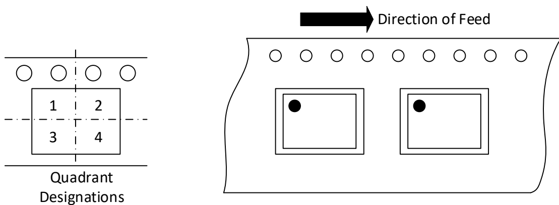
Figure 13.2 Tape Information of SOP8
