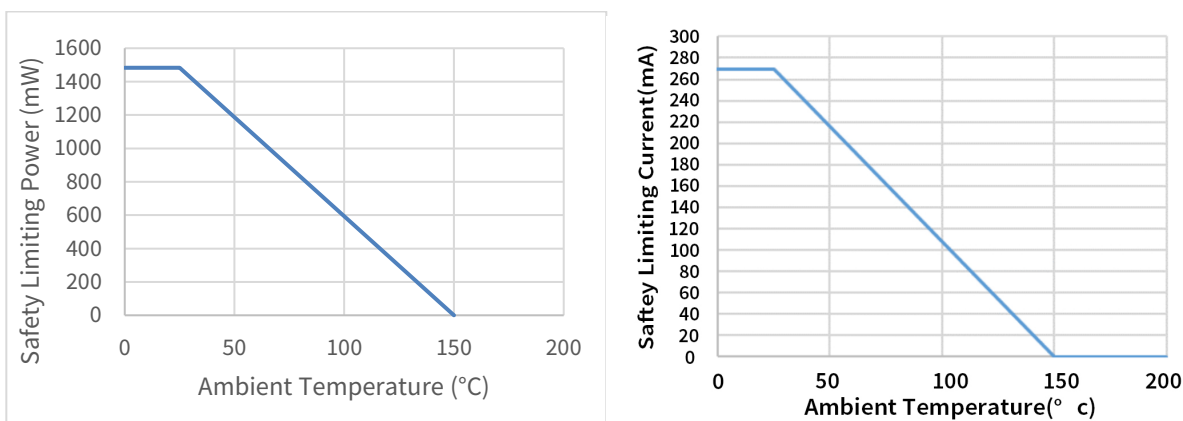
Figure 7.2 NSI8210-DSWVR Thermal Derating Curve, Dependence of Safety Limiting Values with Case Temperature per DIN VDE V 0884-17
