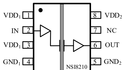
Figure 1.1 NSI8210 Block Diagram
