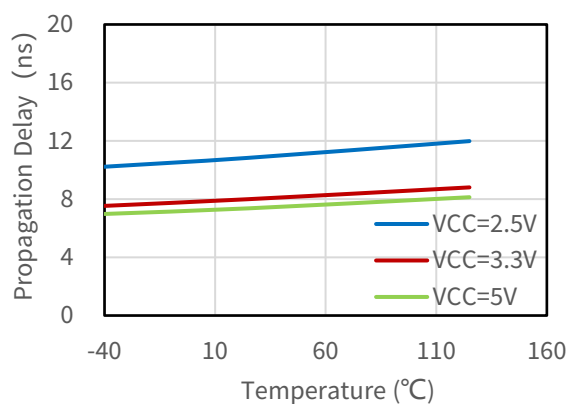
Figure 6.4 NSI8210-DSPR Falling Edge Propagation Delay Vs Temp
