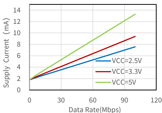
Figure 6.6 NSI8210-DSWVR VDD2 Supply Current vs Data Rate
