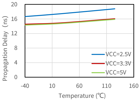
Figure 6.7 NSI8210-DSWVR Rising Edge Propagation Delay Vs Temp
