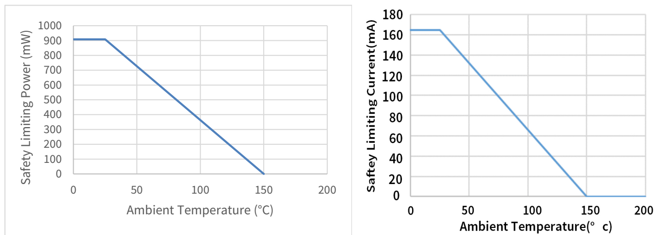
Figure 7.1 NSI8210-DSPR Thermal Derating Curve, Dependence of Safety Limiting Values with Case Temperature per DIN VDE V 0884-17
