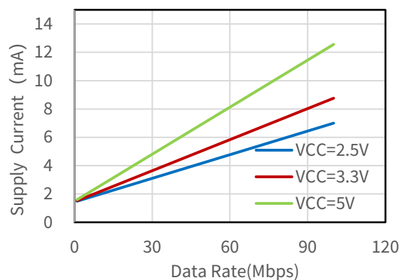
Figure 6.2 NSI8210-DSPR VDD2 Supply Current vs Data Rate
