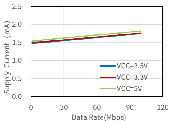
Figure 6.1 NSI8210-DSPR VDD1 Supply Current vs Data Rate
