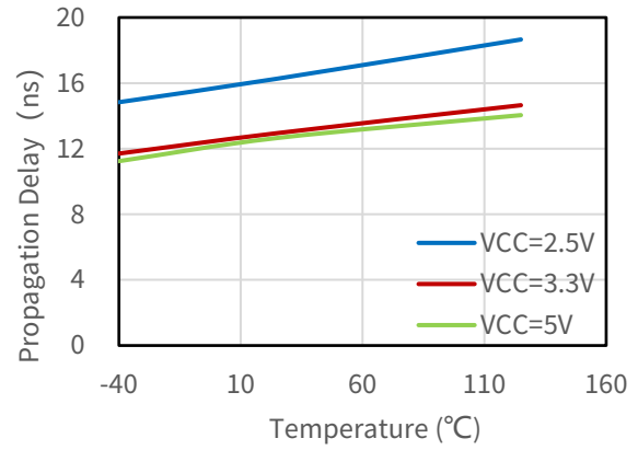
Figure 6.8 NSI8210-DSWVR Falling Edge Propagation Delay Vs Temp
