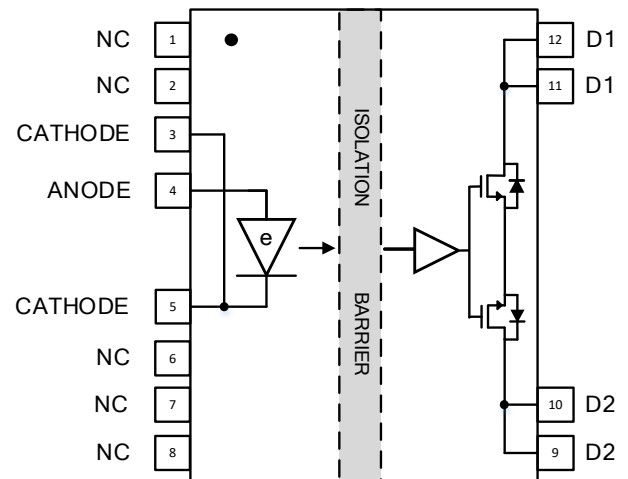
Figure 1. NSI7117 Block Diagram
