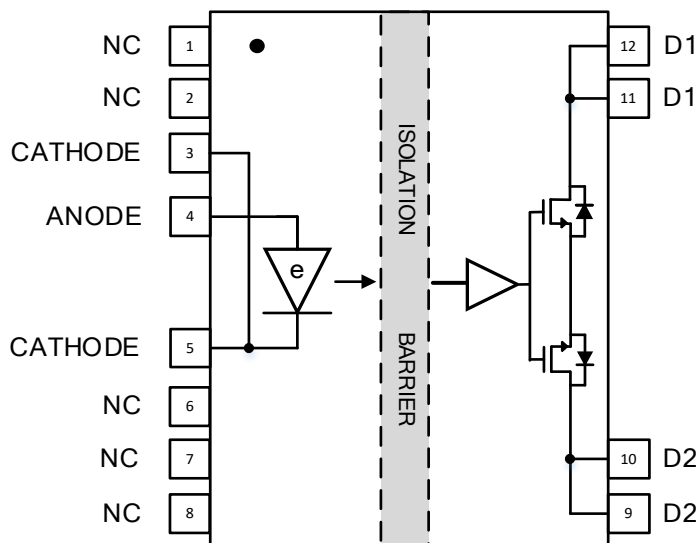
Figure 1.1 NSI7117 Package
