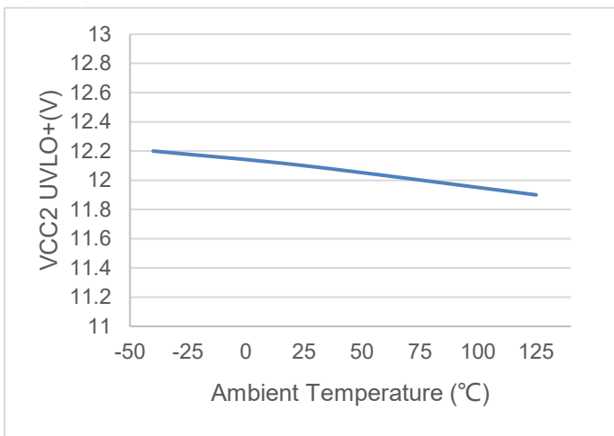
Figure 7.6 VCC2 UVLO+ vs temperature
