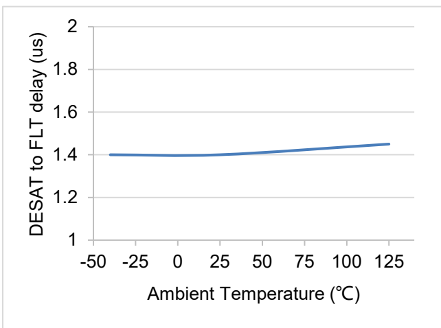
Figure 7.21 DESAT to FLT delay vs temperature
