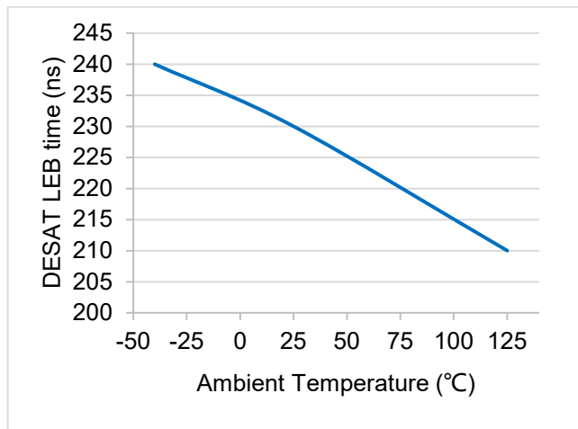
Figure 7.19 DESAT LEB time vs temperature
