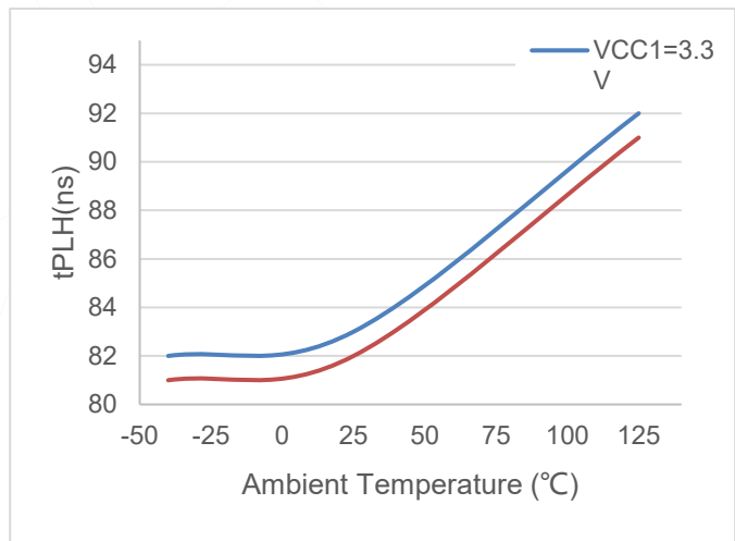
Figure 7.10 t_{PLH\_IN+} vs temperature
