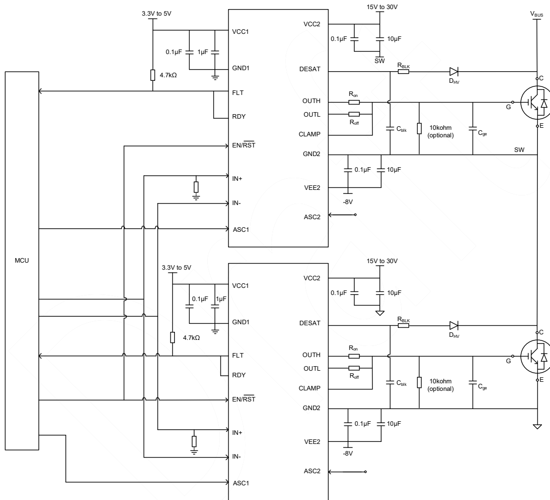
Figure 9.1 typical application
