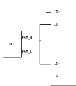
Figure 9.3 interlock protection
