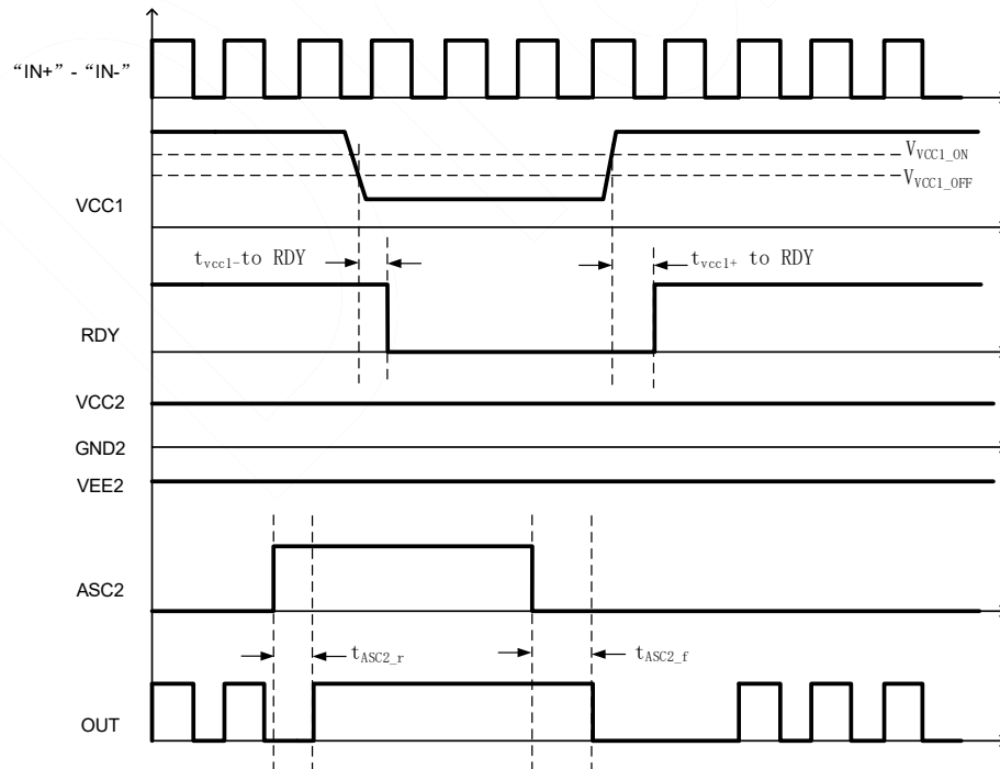
Figure 8.9 ASC2 protection with V_{CC1} UVLO Timing Diagram
