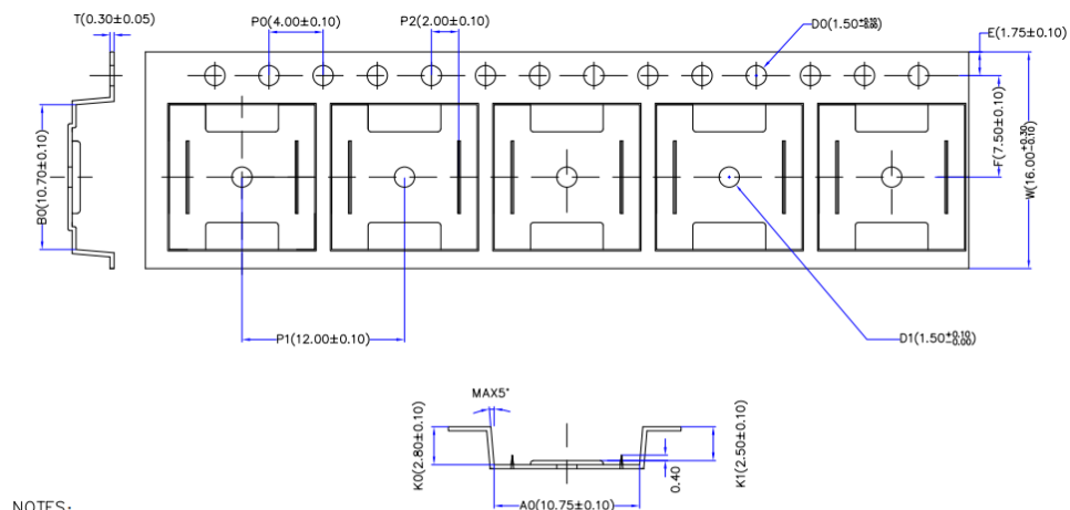
Figure 13.3 Reel Information (TongFu)
