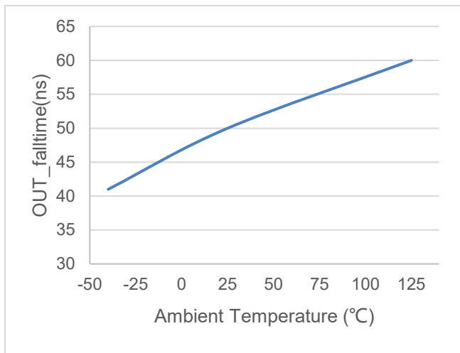
Figure 7.9 fall time vs temperature
