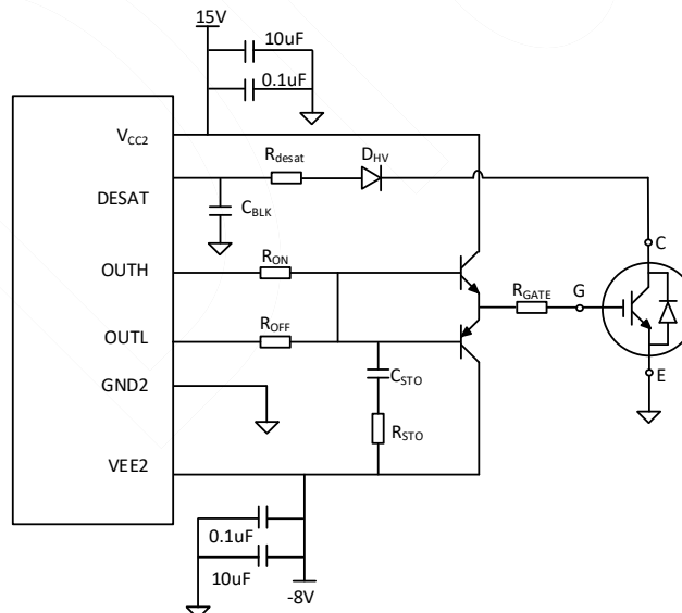
Figure 9.4 external current buffer
