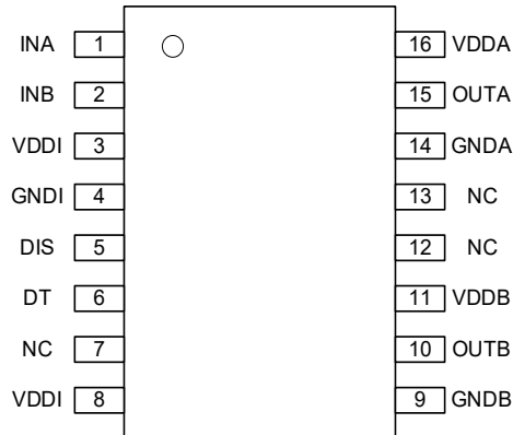
Figure 1.1 NSI6602Hx SOW16/SOP16 Package
