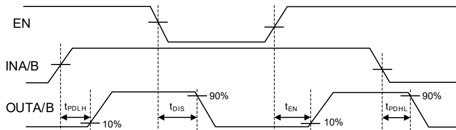
Figure 6.23 Disable Time and Enable Time (NSI6602NHx)
