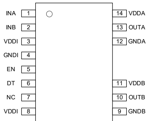
Figure 1.4 NSI6602NHx SOW14 Package
