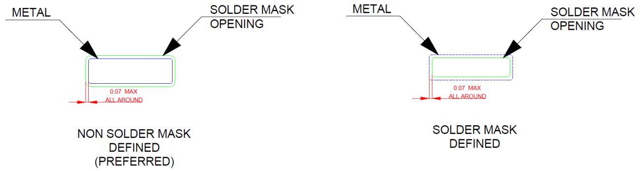
Figure 10.7 Solder Mask Details(mm)
