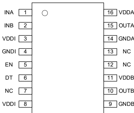
Figure 1.3 NSI6602NHx SOW16/SOP16 Package
