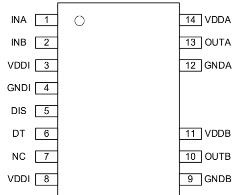
Figure 1.2 NSI6602Hx SOW14 Package
