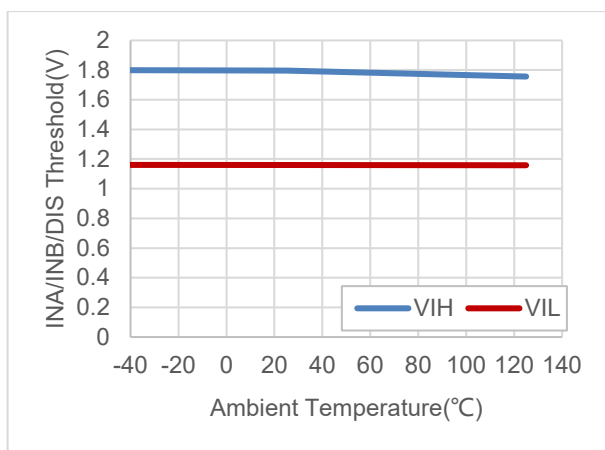
Figure 6.11 INA/INB/DIS(EN) Threshold vs. Temperature
