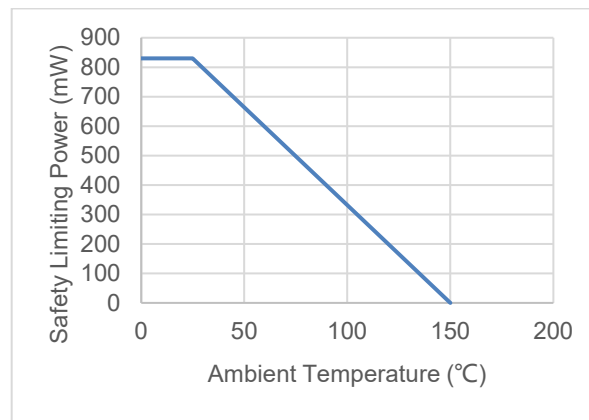
Figure 7.2 NSI6602x-Q1SPNR Thermal Derating Curve, Dependence of Safety Limiting Values with Case Temperature per DIN VDE V 0884-17.
