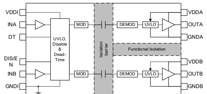
Figure 0.1 NSI6602xHx Block Diagram
