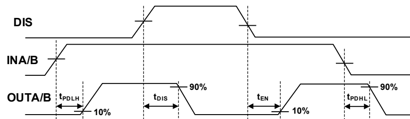
Figure 6.22 Disable Time and Enable Time(NSI6602Hx)
