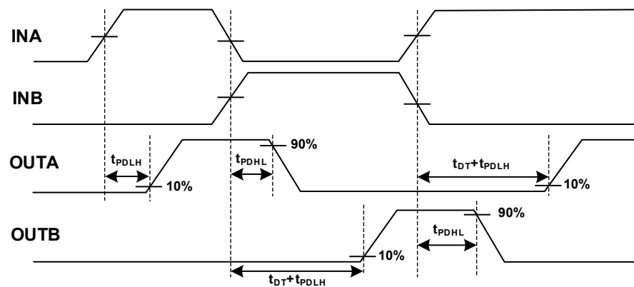
Figure 6.24 Deadtime, Determined by RDT
