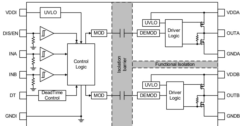
Figure 8.1 Functional Block Diagram
