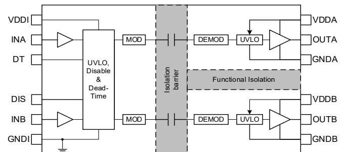
Figure 0.1 NSI6602H Block Diagram
