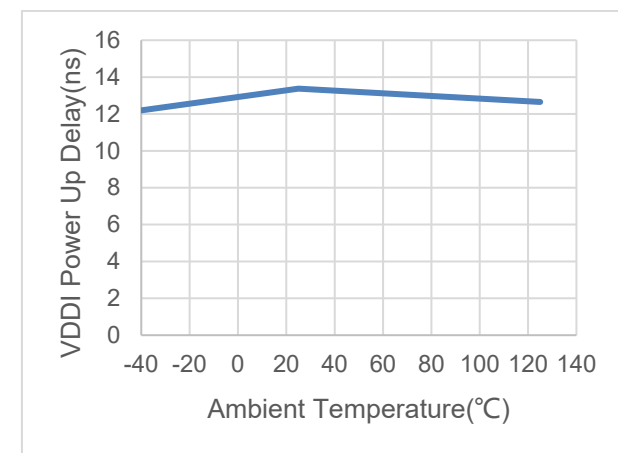
Figure 6.16 VDDI power up delay vs. Temperature
