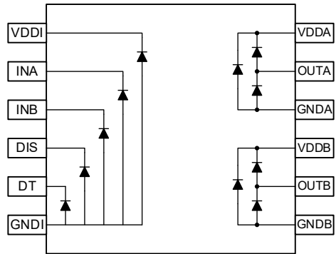
Figure 8.3 ESD Structure
