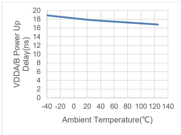
Figure 6.17 VDDA/B power up delay vs. Temperature
