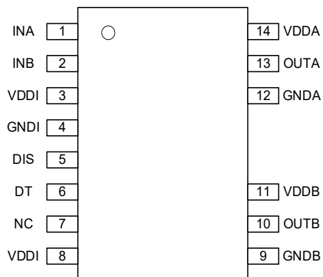
Figure 1.3 NSI6602H SOW14 Package
