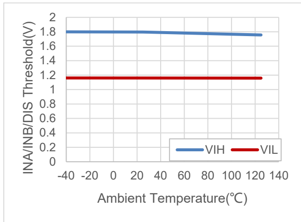
Figure 6.11 INA/INB/DIS Threshold vs. Temperature
