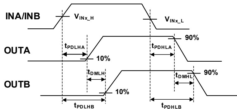
Figure 6.20 Propagation Delay and Channel to Channel Delay Match Time, connect DT to VDDI
