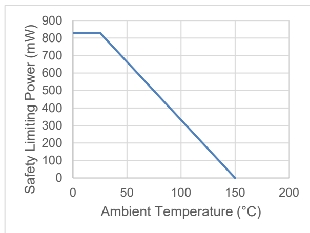
Figure 7.3 NSI6602Hx-DSPxR Thermal Derating Curve, Dependence of Safety Limiting Values with Case Temperature per DIN VDE V 0884-17.
