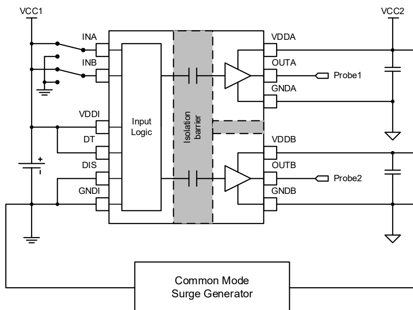
Figure 6.24 Common-Mode Transient Immunity Test Circuit
