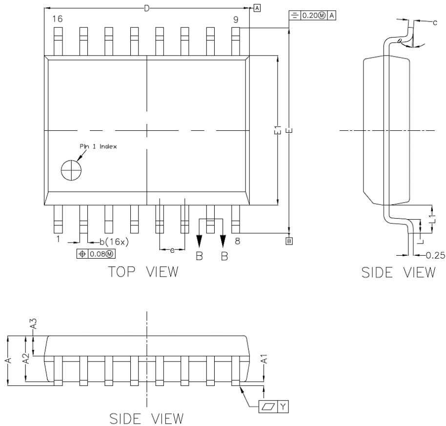
Figure 10.3 SOW16 Package Shape and Dimension
