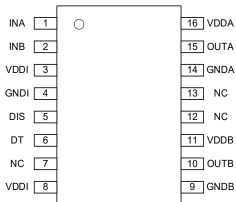
Figure 1.2 NSI6602H SOW16/ SOP16 Package
