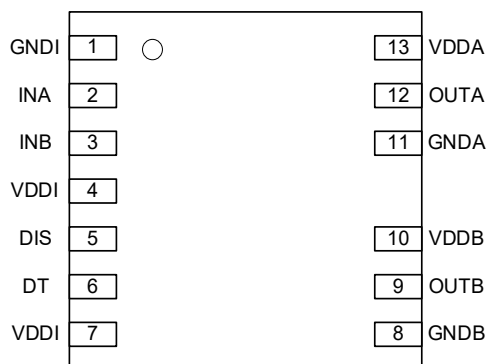
Figure 1.1 NSI6602H LGA13 Package
