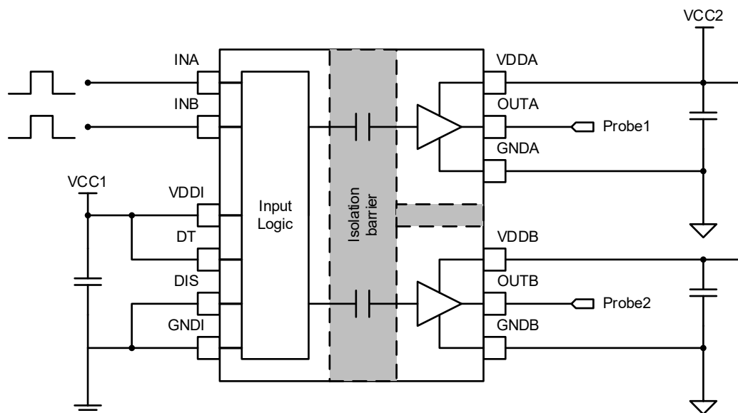
Figure 6.21 Channel to Channel Delay Match Test Circuit
