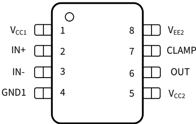
Figure 1.1 NSI6601ME Versions (Top View)
