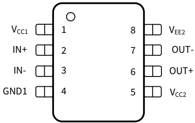
Figure 1.2 NSI6601AE Versions (Top View)
