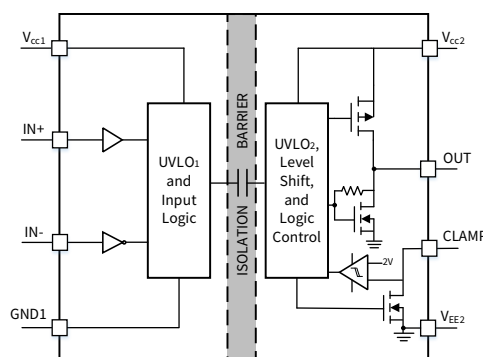
Figure 0.1 NSI6601ME Diagram
