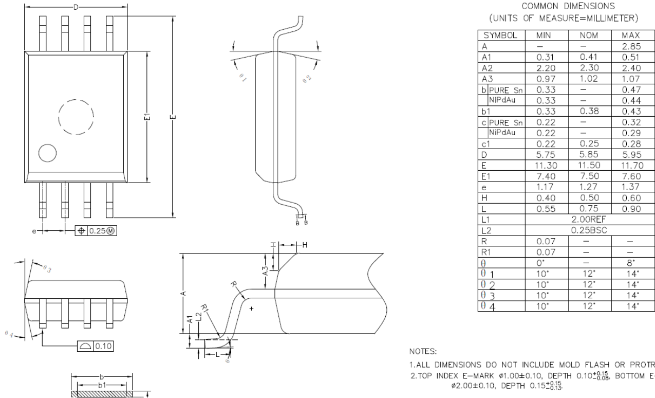
Figure 10.4 SOW8 Package Shape and Dimension in millimeters
