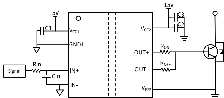
Figure 9.2 NSI6601AE Typical Application Circuit
