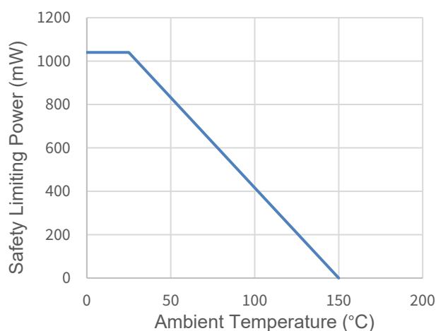
Figure 7.1 Thermal Derating Curve for Limiting Power per DIN VDE V 0884-17 for SOP8 Package
