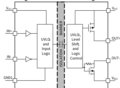
Figure 0.2 NSI6601AE Diagram
