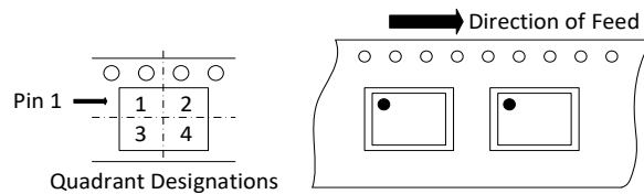
Figure 13.2 Tape Information of SOP16(300mil)
