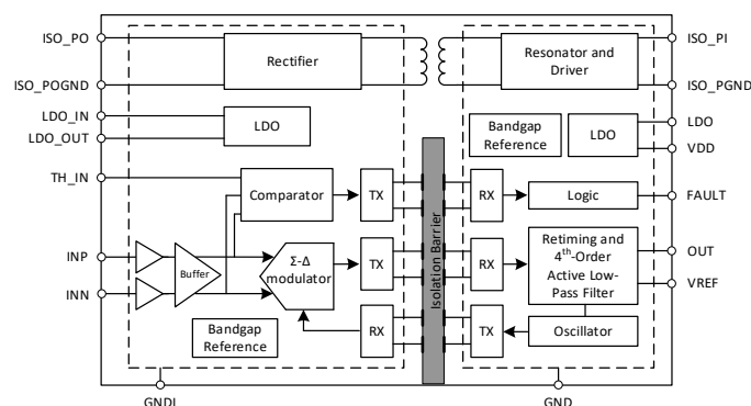
Figure 1. Function Block Diagram of NSI36C12R
