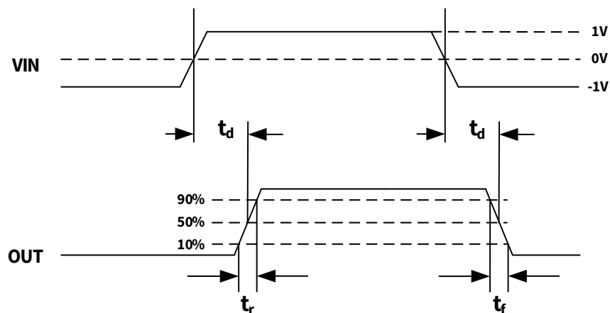
Figure 6.1 Propagation Delay and Output Fall Time Definition
