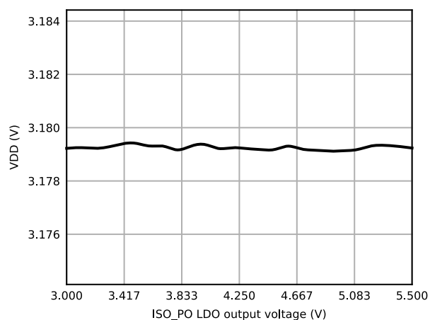
Figure 6.32 ISO-PO LDO Regulation
