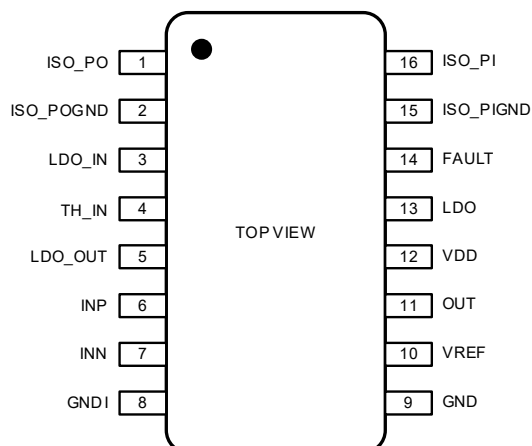
Figure 1.1 NSI36C12R Package
