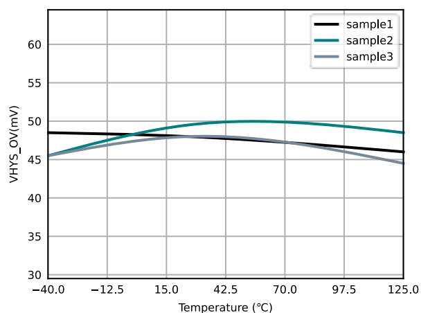
Figure 6.31 VHYS_OV vs Temperature
