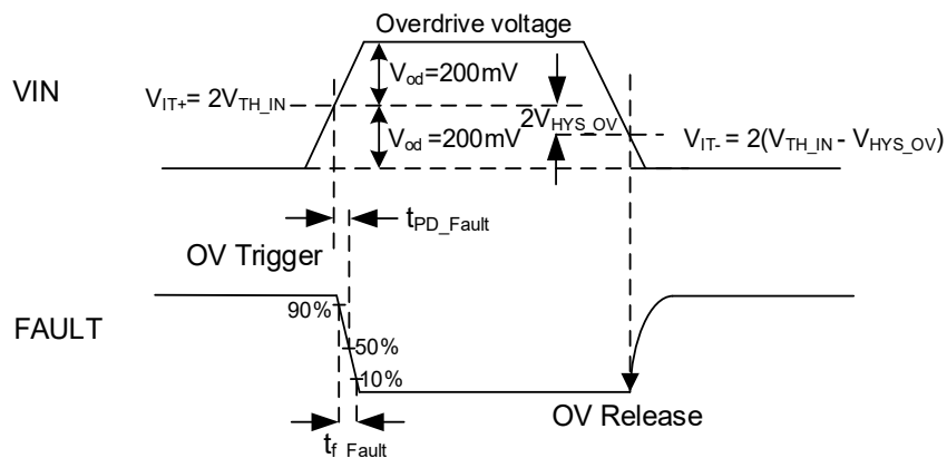
Figure 6.2 Propagation Delay and Output Fall Time Definition for Protection Comparator
