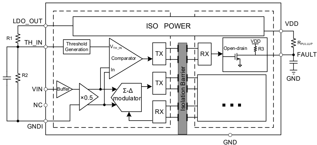
Figure 8.5 Function Block Diagram of Comparator
