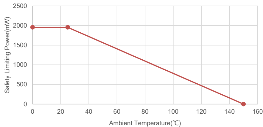
Figure 7.1 NSI36C11R Thermal Derating Curve, Dependence of Safety Limiting Values with Case Temperature per DIN VDE V 0884-11
