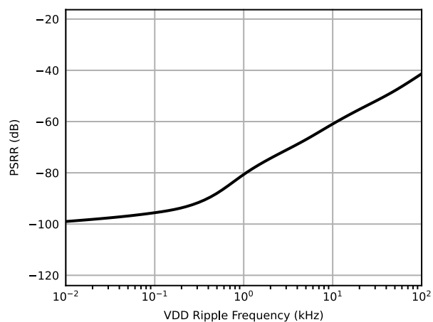
Figure 6.28 Power-Supply Rejection Ratio vs VDD Input Frequency
