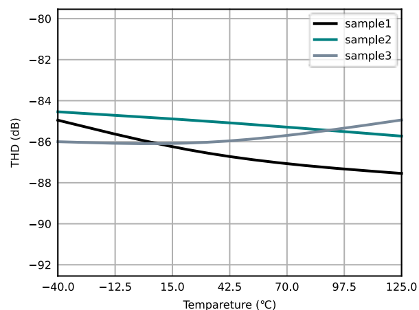
Figure 6.16 Total Harmonic Distortion vs Temperature
