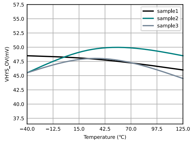
Figure 6.26 V_{HYS\_OV} vs Temperature
