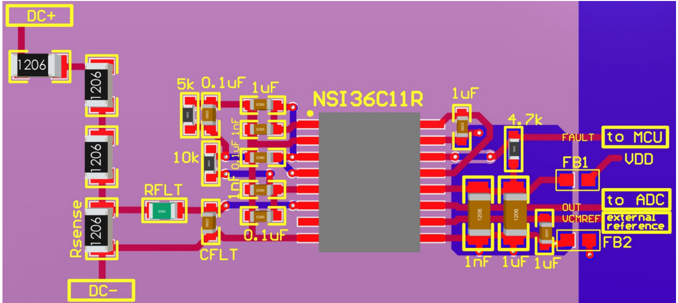
Figure 9.3 PCB layout example of NSI36C11R
