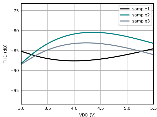
Figure 6.15 Total Harmonic Distortion vs Supply Voltage ( V_{REF} = VDD )
