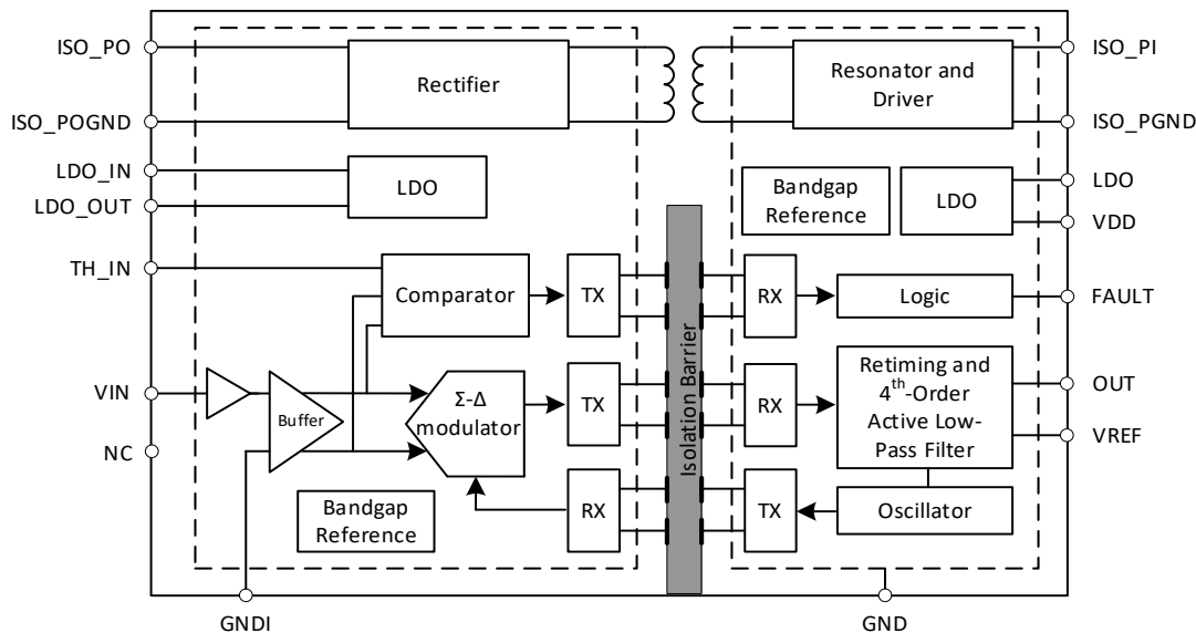
Figure 8.1 Function Block Diagram of NSI36C11R
