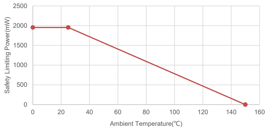
Figure 7.1 NSI36C11R Thermal Derating Curve, Dependence of Safety Limiting Values with Case Temperature per DIN VDE V 0884-11
