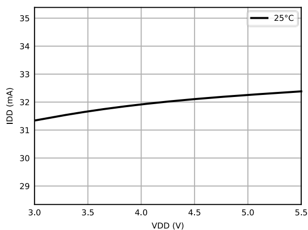
Figure 6.19 Input Supply Current vs Supply Voltage ( I_E=0.5\text{mA} , over-threshold protection not triggered)
