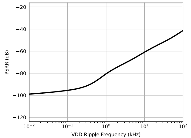
Figure 6.28 Power-Supply Rejection Ratio vs VDD Input Frequency
