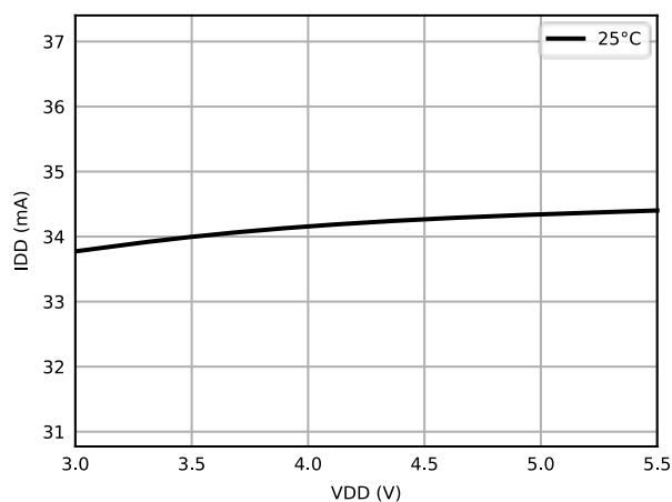
Figure 6.21 Input Supply Current vs Supply Voltage ( I_E=0.5\text{mA} , over-threshold protection triggered)
