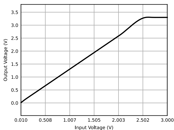
Figure 6.3 Output Voltage vs Input Voltage ( V_{REF} = V_{DD} = 3.3V )
