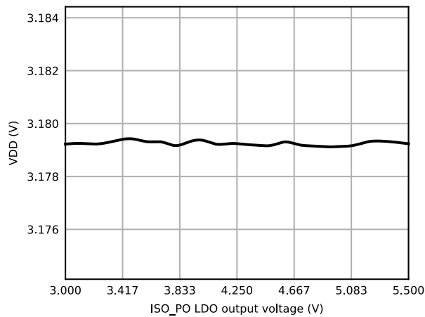
Figure 6.27 ISO-PO LDO Regulation
