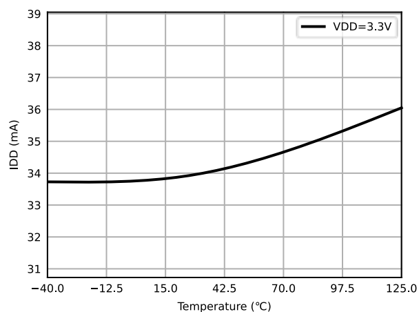
Figure 6.22 Input Supply Current vs Temperature ( I_E=0.5\text{mA} , over-threshold protection triggered)
