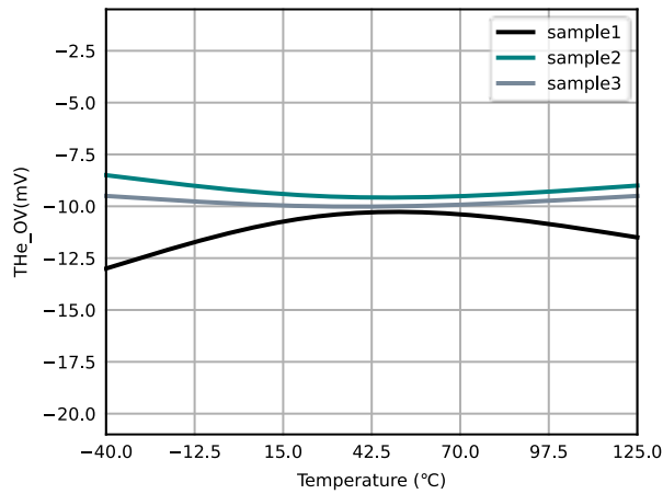
Figure 6.25 The_{OV} vs Temperature
