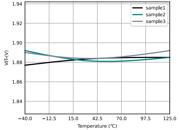
Figure 6.24 VIT- vs Temperature ( V_{TH\_IN} = 2 \times 0.5 \text{ V} )
