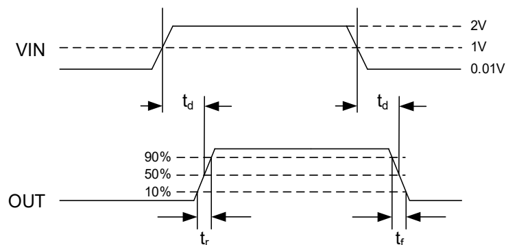
Figure 6.1 Propagation Delay and Output Fall Time Definition
