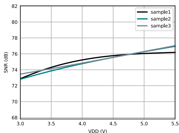
Figure 6.13 Signal to Noise Ratio vs Supply Voltage ( V_{REF} = VDD )
