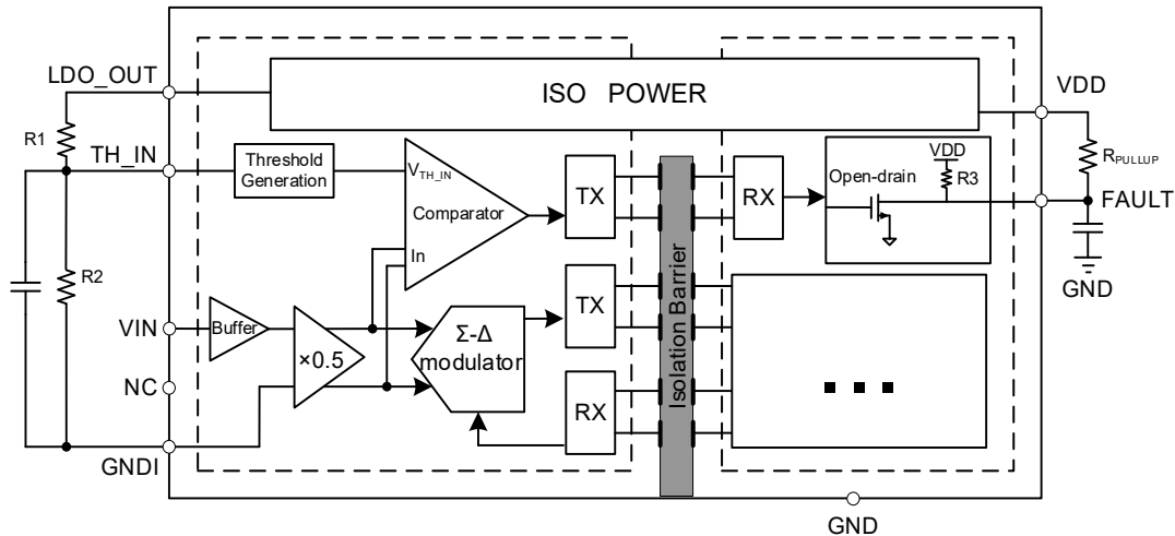
Figure 8.5 Function Block Diagram of Comparator
