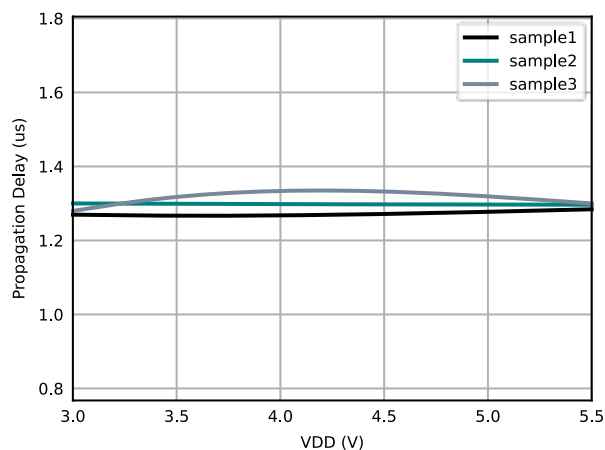
Figure 6.17 Input and Output Signal Delay time vs Supply Voltage
