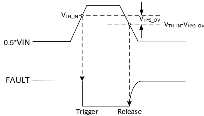
Figure 8.6 Switching Characteristic of Input Over-threshold Protection Function
