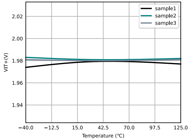
Figure 6.23 VIT+ vs Temperature ( V_{TH\_IN} = 2 \times 0.5 \text{ V} )
