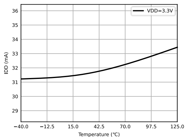
Figure 6.20 Input Supply Current vs Temperature ( I_E=0.5\text{mA} , over-threshold protection not triggered)
