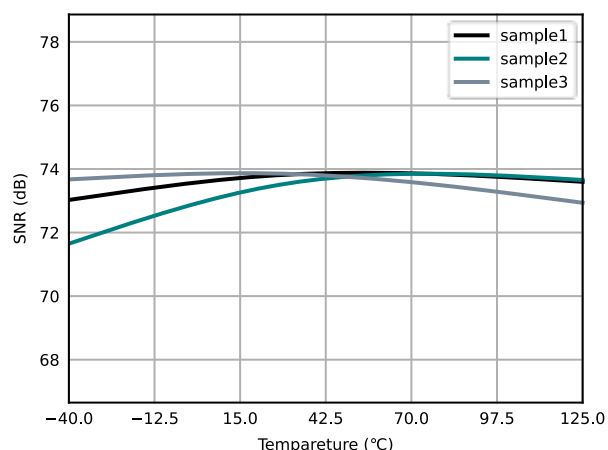
Figure 6.14 Signal to Noise Ratio vs Temperature
