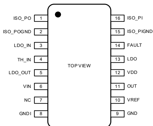
Figure 1.1 NSI36C11R Package
