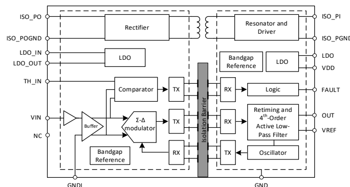
Figure 1. Function Block Diagram of NSI36C11R
