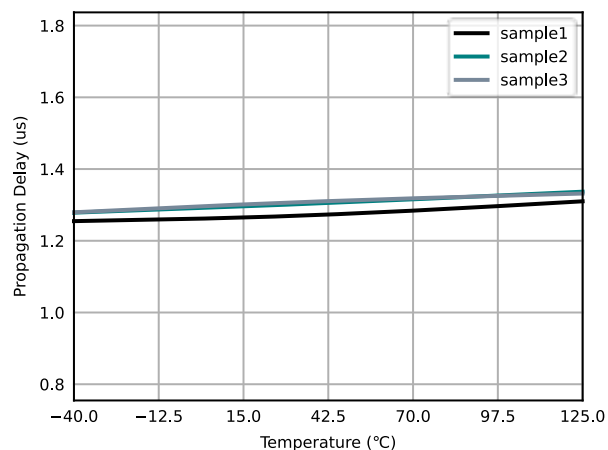
Figure 6.18 Input and Output Signal Delay time vs Temperature
