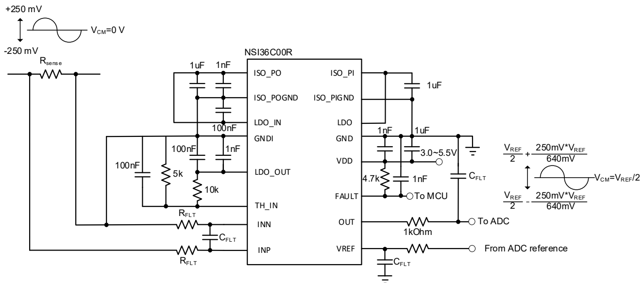
Figure 9.1 Typical application circuit
