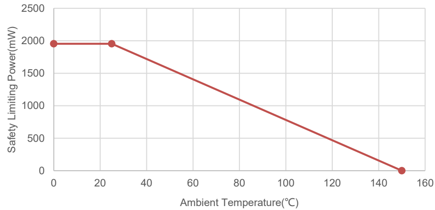
Figure 7.1 NSI36C00R Thermal Derating Curve, Dependence of Safety Limiting Values with Case Temperature per DIN VDE V 0884-11
