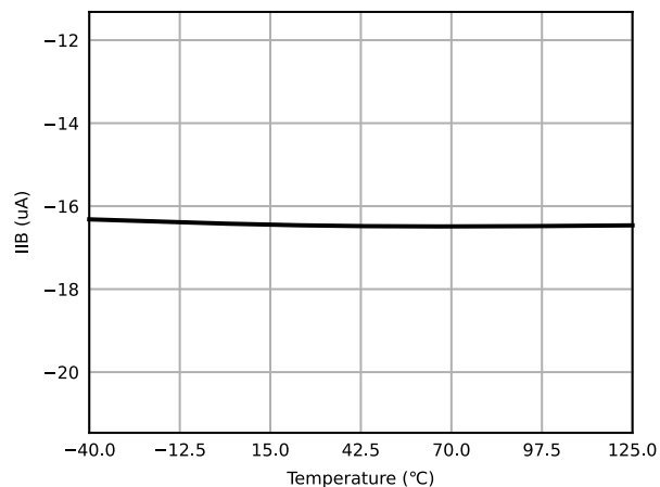
Figure 6.4 Input Bias Current vs Temperature
