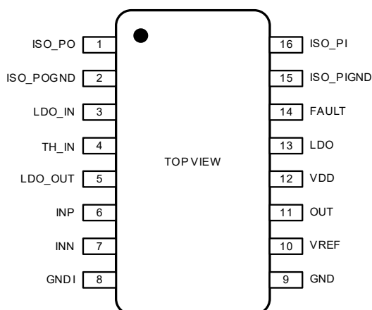
Figure 1.1 NSI36C00R Package
