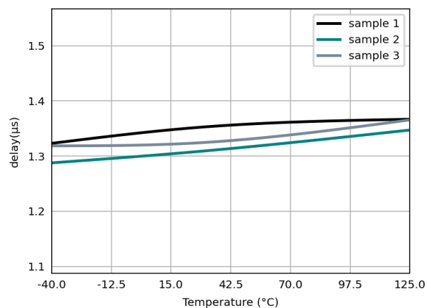
Figure 6.36 Input and Output Signal Delay time vs Temperature
