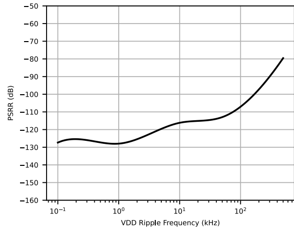
Figure 6.21 Power-Supply Rejection Ratio vs VDD Input Frequency
