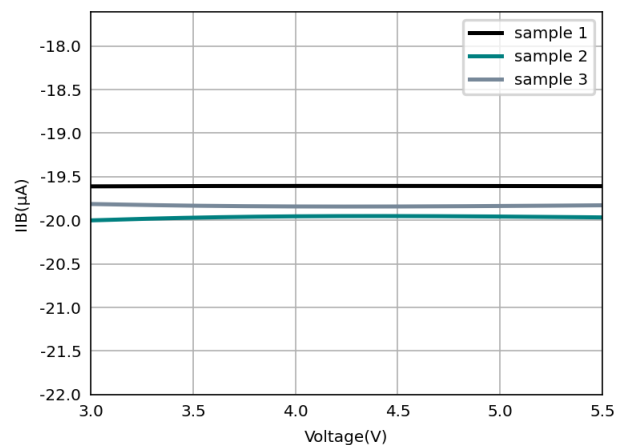
Figure 6.3 Input Bias Current vs Supply Voltage
