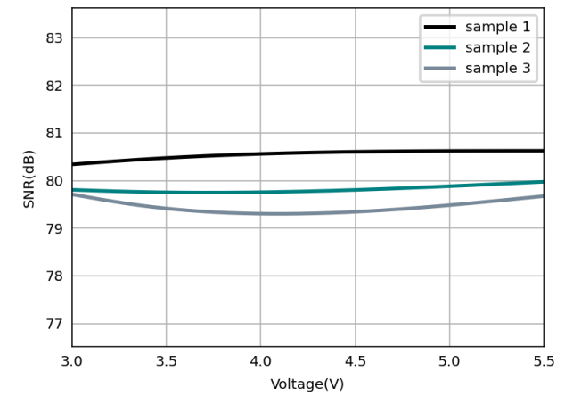
Figure 6.15 Signal to Noise Ratio vs Supply Voltage
