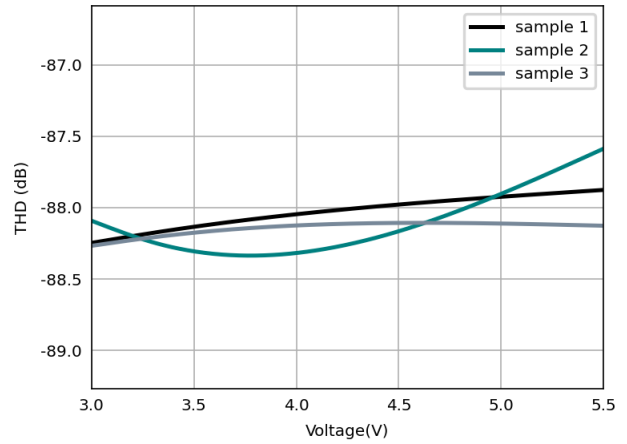
Figure 6.17 Total Harmonic Distortion vs Supply Voltage
