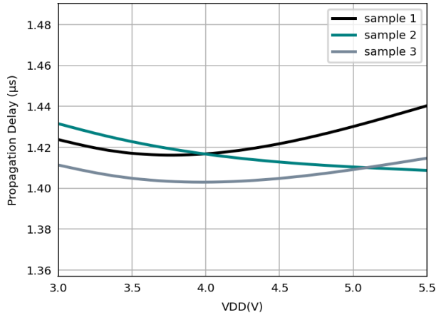
Figure 6.27 Input and Output Signal Delay time vs Supply Voltage
