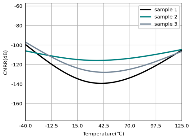
Figure 6.20 Common-Mode Rejection Ratio vs Temperature
