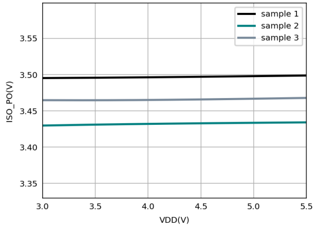
Figure 6.23 ISO-PO LDO Regulation
