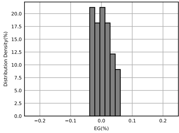
Figure 6.11 Gain Error Distribution (1)
