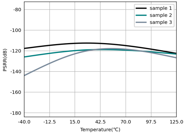
Figure 6.22 Power-Supply Rejection Ratio vs Temperature
