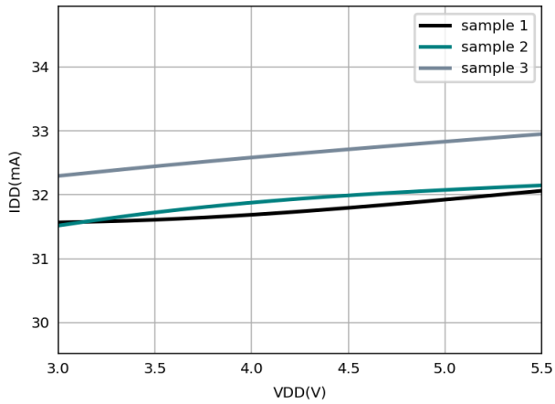
Figure 6.24 Input Supply Current vs Supply Voltage (IE=1mA)
