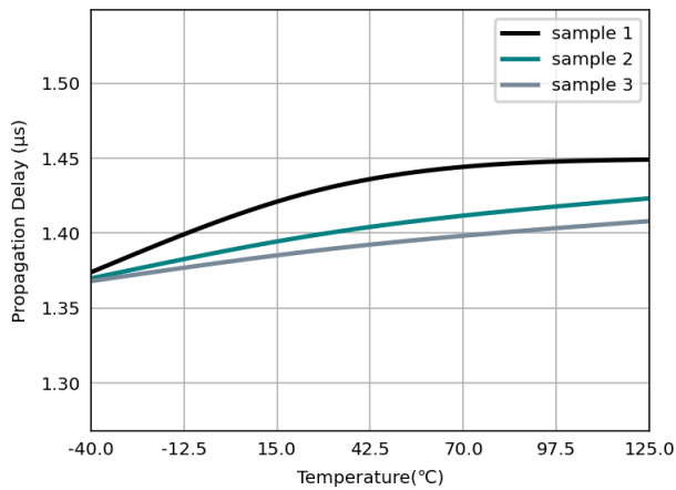
Figure 6.26 Input and Output Signal Delay time vs Temperature
