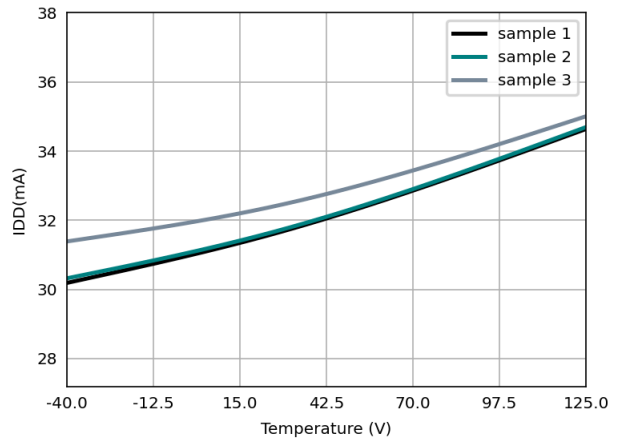
Figure 6.25 Input Supply Current vs Temperature (IE=1mA)
