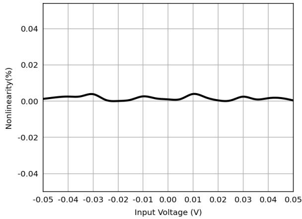
Figure 6.18 Nonlinearity vs Input Voltage
